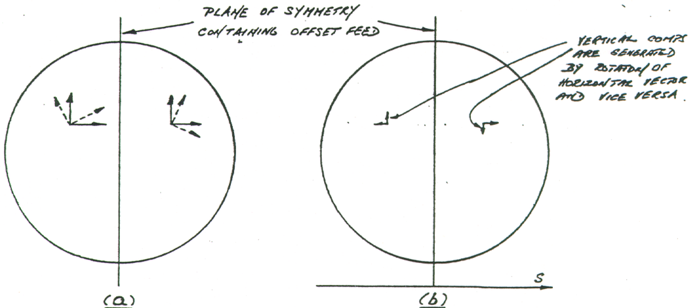
Figure 2. Aperture of antenna. (a) Full-line arrows show E-vector as transmitted from feed, and broken arrows as rotated after reflection. (b) Rotation is equivalent to the generation of the cross polarization vectors shown.
