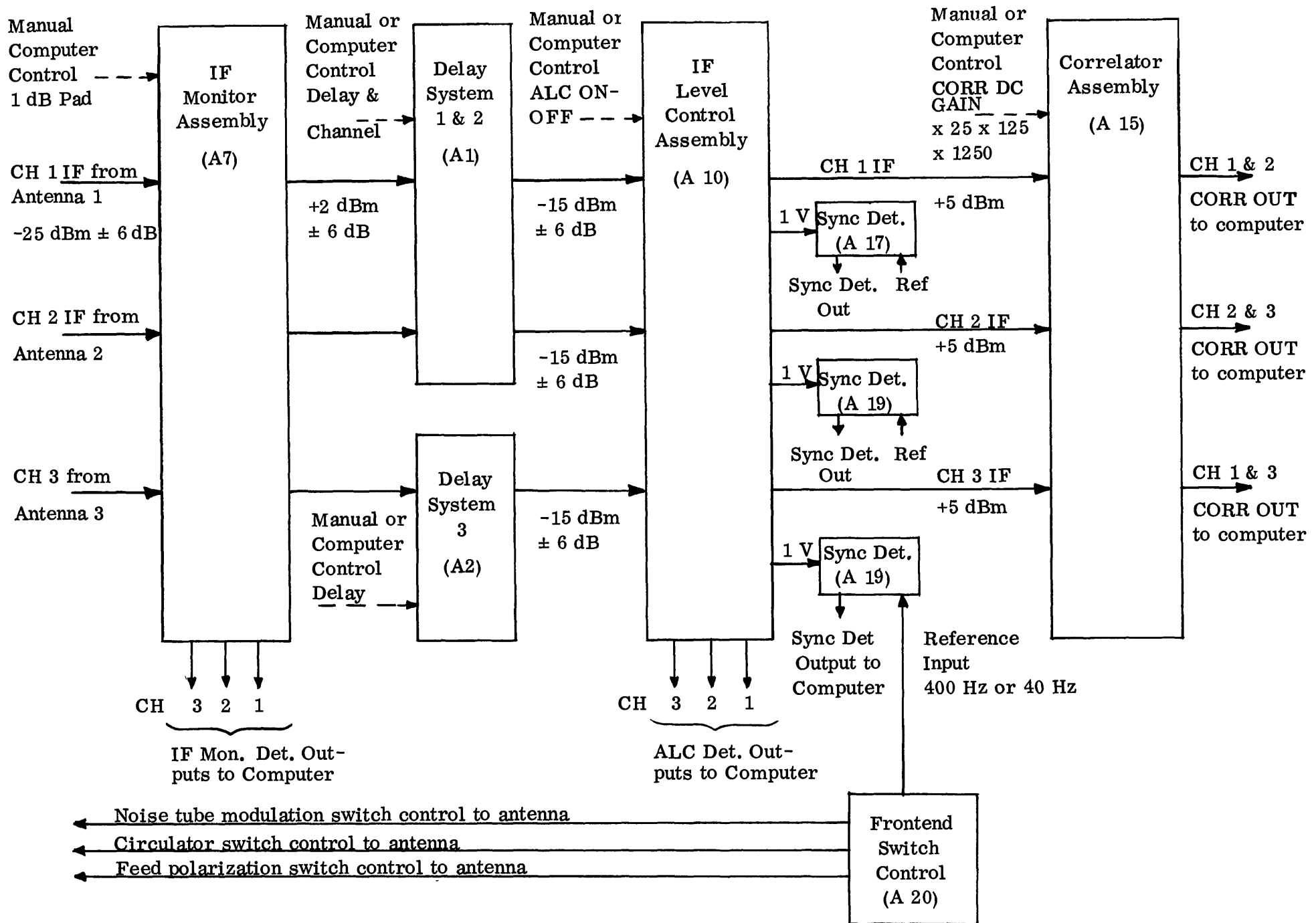
Figure 1 - 3-Element Interferometer Receiver Backend Block Diagram
