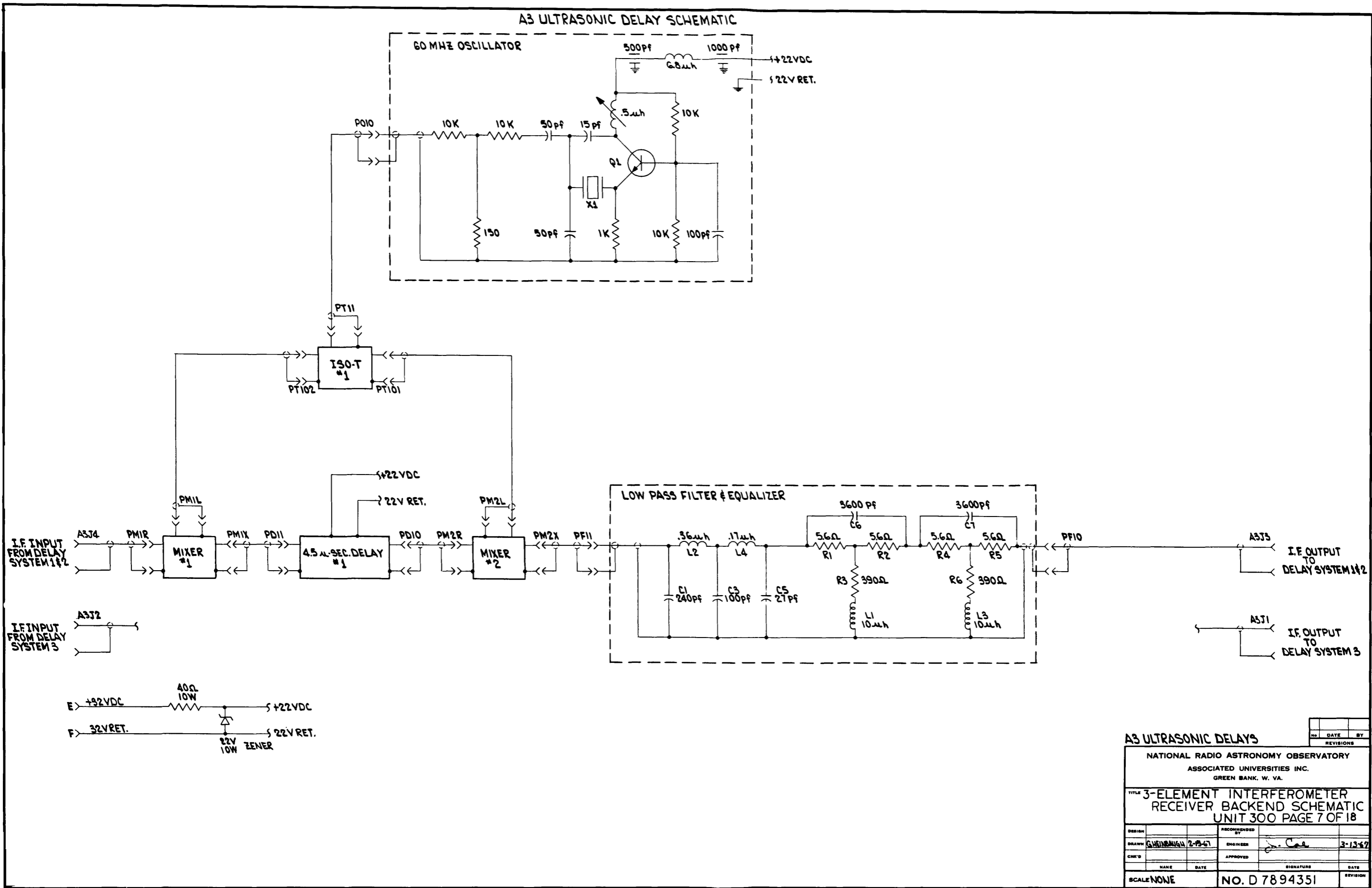
Figure 10 - Ultrasonic Delay System Schematic
