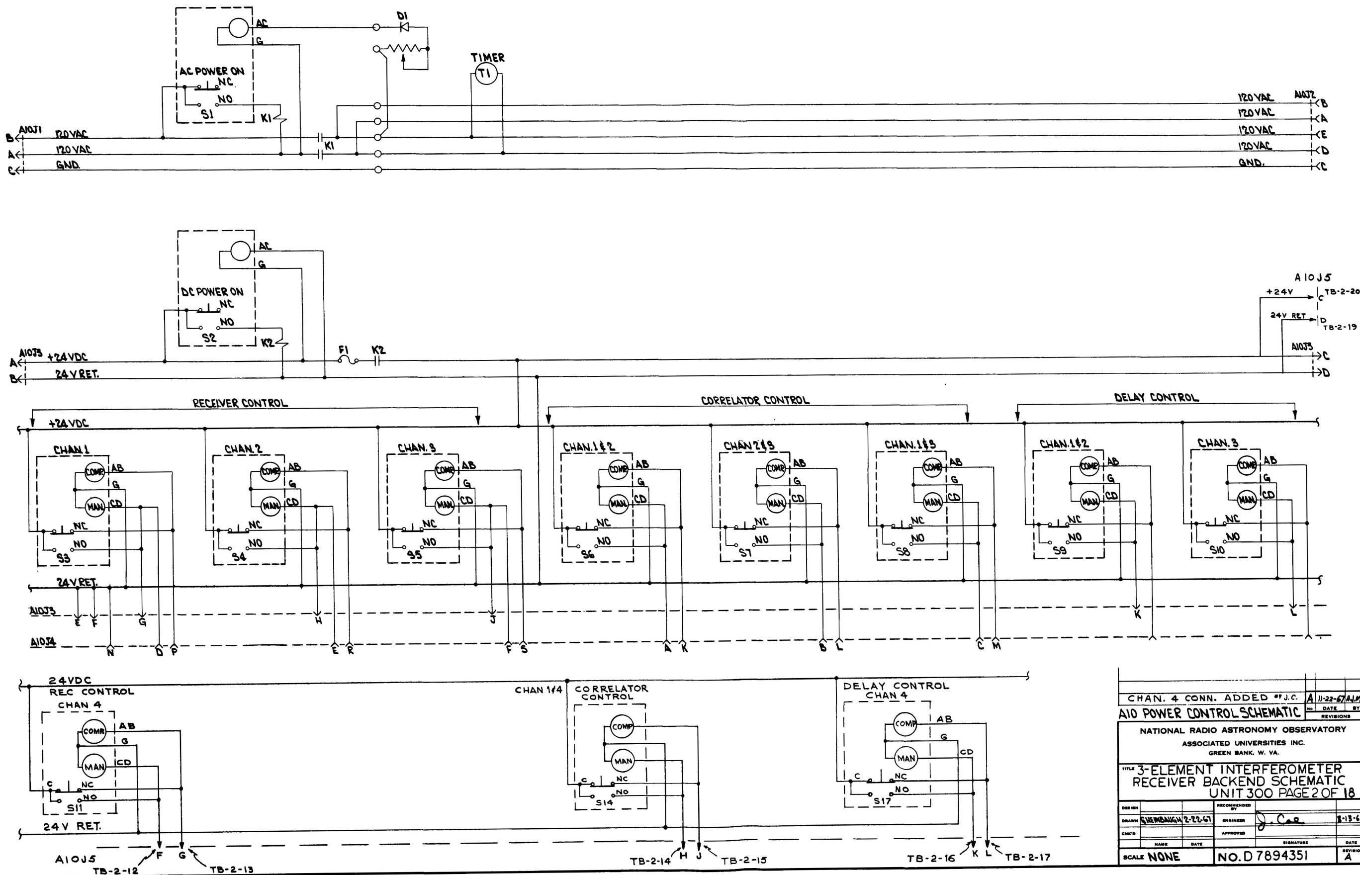
Figure 19 — Power Control Schematic
