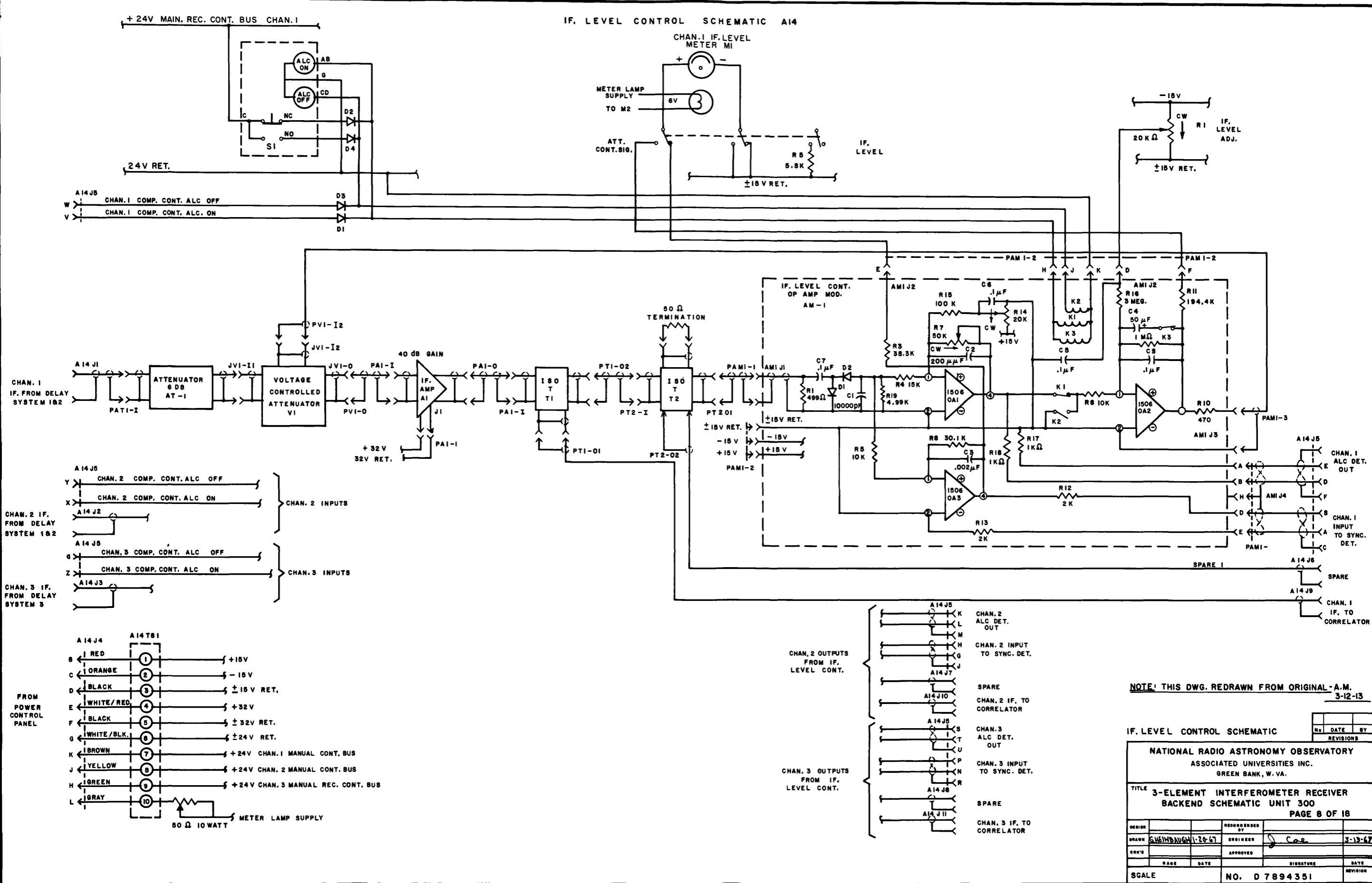
Figure 11 - IF Level Control Assembly Schematic
