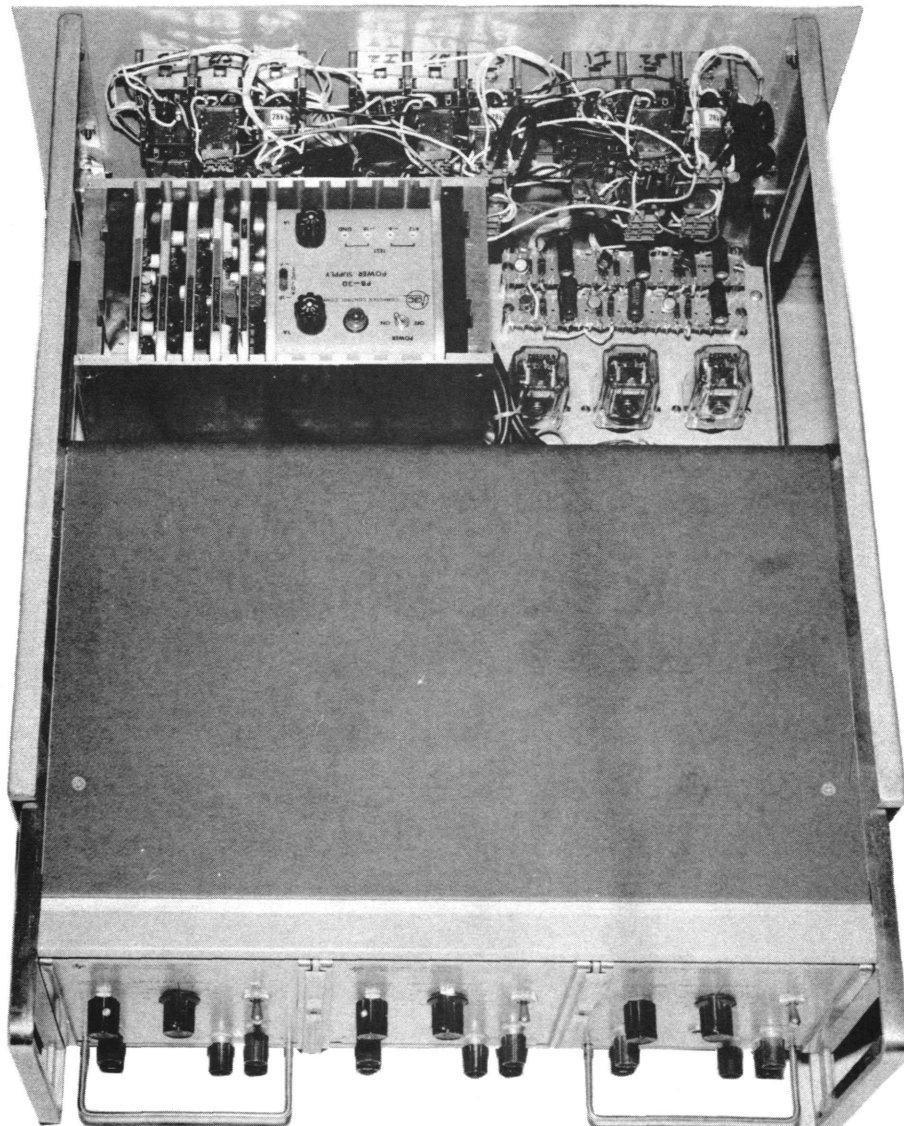
Figure 18 — Frontend Switch Control Front Panel and Chassis
