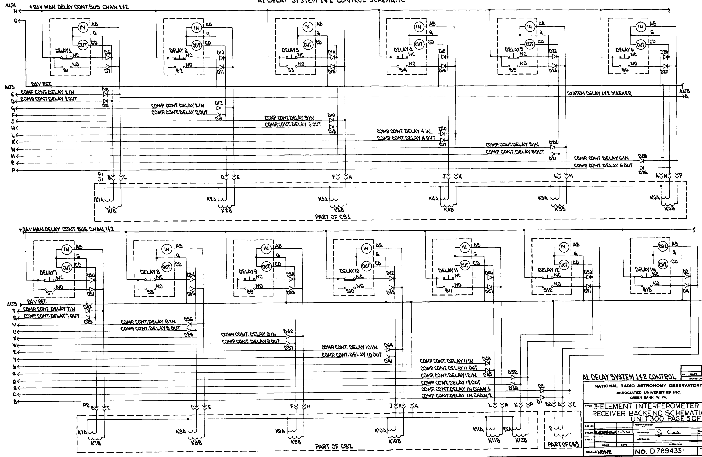
Figure 6 - Delay System 1 & 2 Control Schematic
