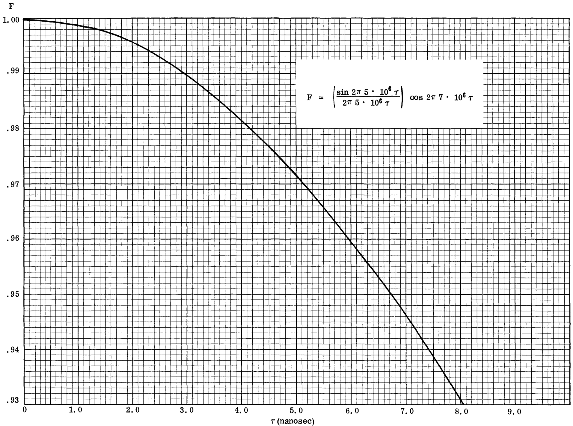
Figure 5 — Fringe Amplitude (F) vs. Time Delay (τ)
