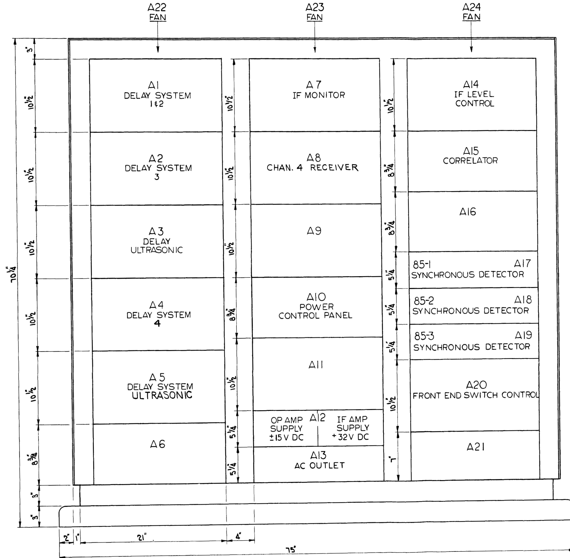
Figure 2 — 3-Element Interferometer Receiver Backend Assembly
