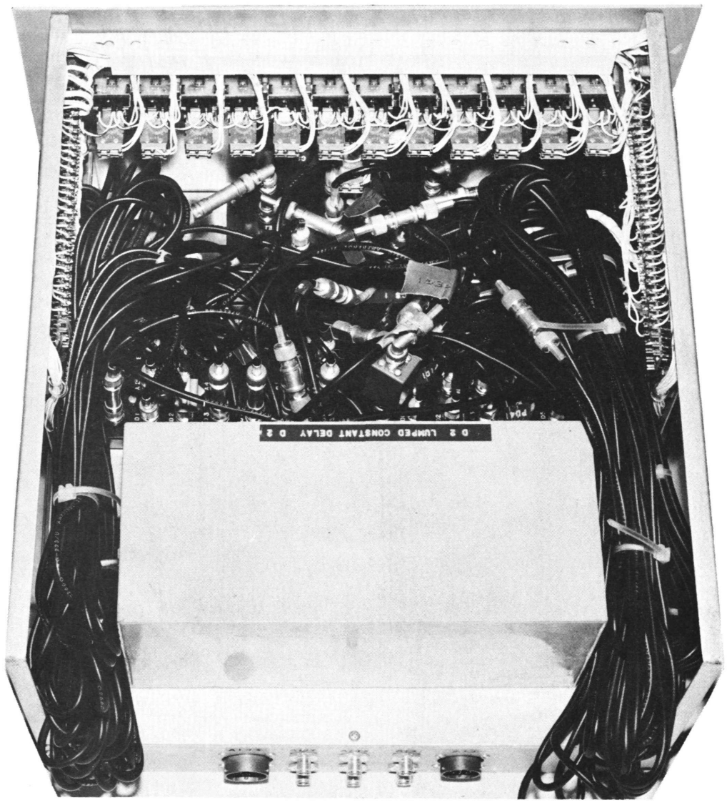
Figure 8 — Delay System 1 & 2 Front Panel and Chassis
