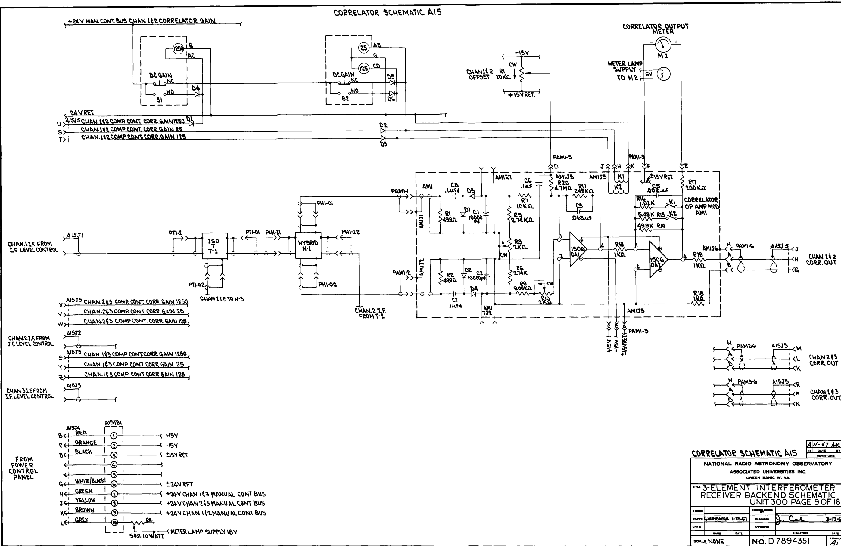
Figure 14 — Correlator Assembly Schematic
