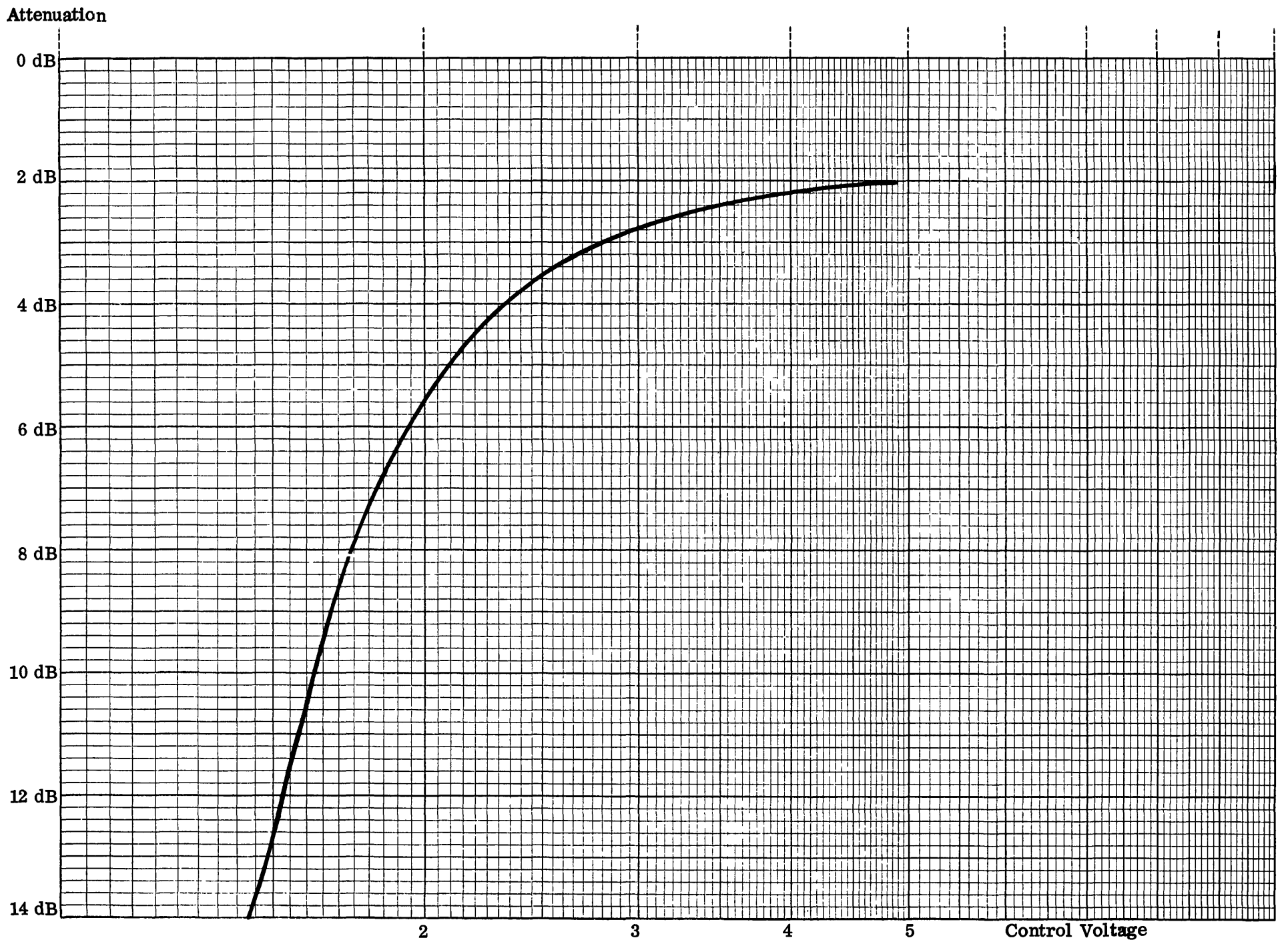
Figure 13 — Voltage Control Attenuator Response
