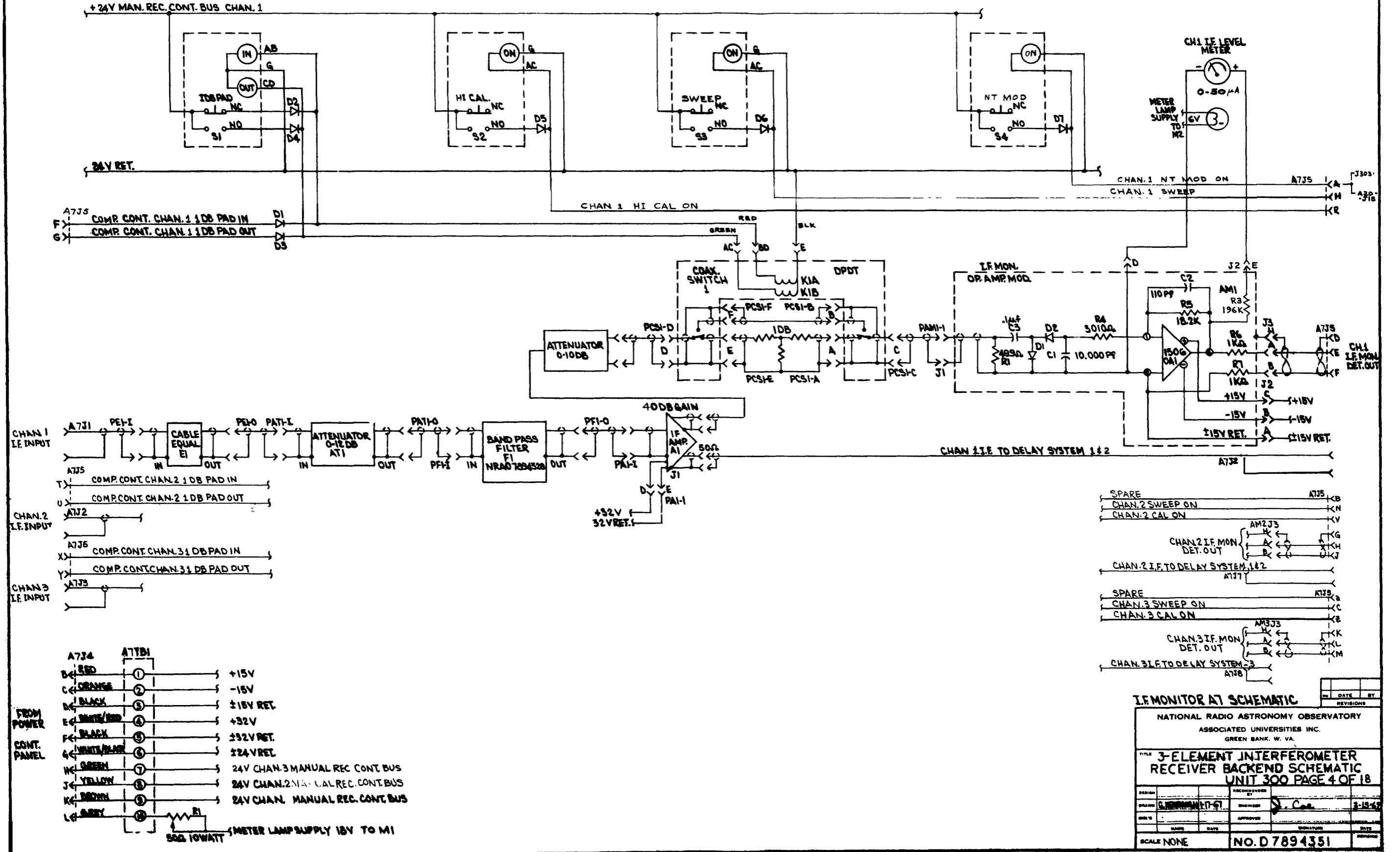
Figure 3 - IF Monitor Assembly Schematic
