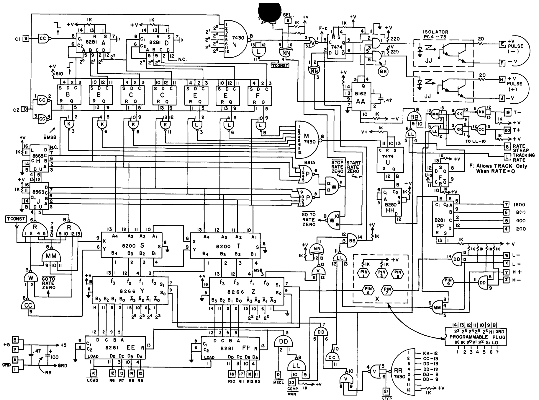
TRANSLATOR DRIVE CONTROL CARD # 2345
