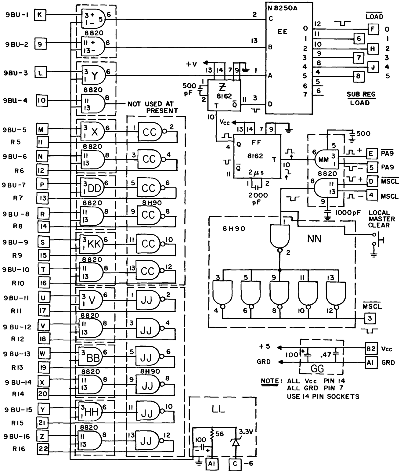
COMPUTER INTERFACE CARD # 1 COMPUTER CONTROL INTERFACE PACKAGE 300FT. TELESCOPE DRIVE SYSTEM
