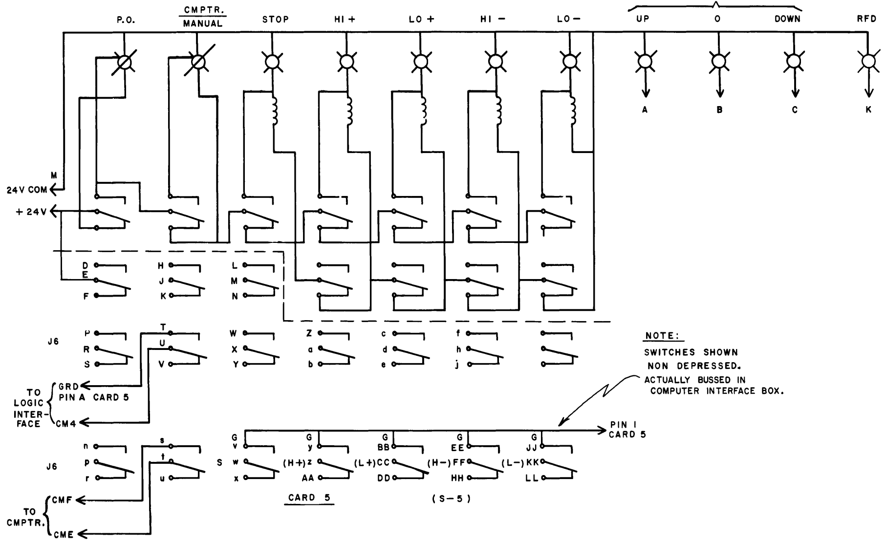
SCHMATIC 3
