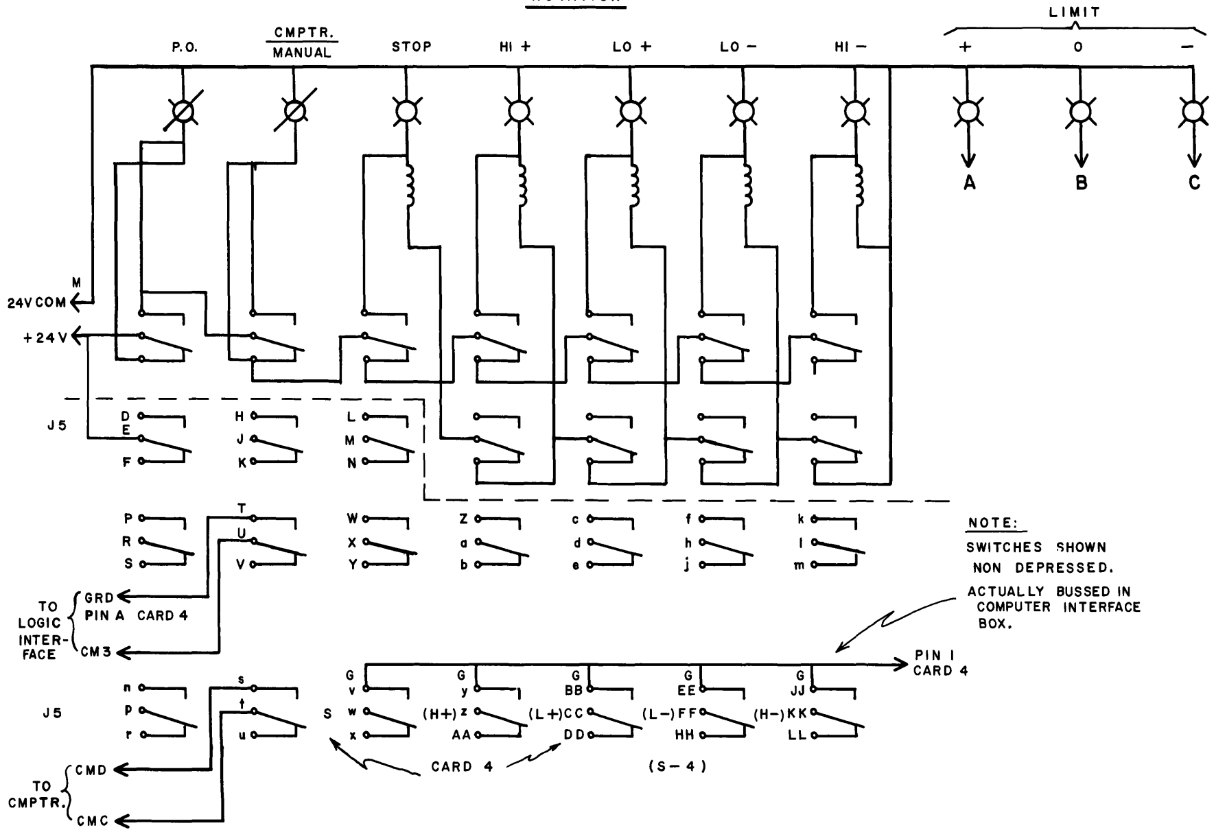
SCHEMATIC 2
