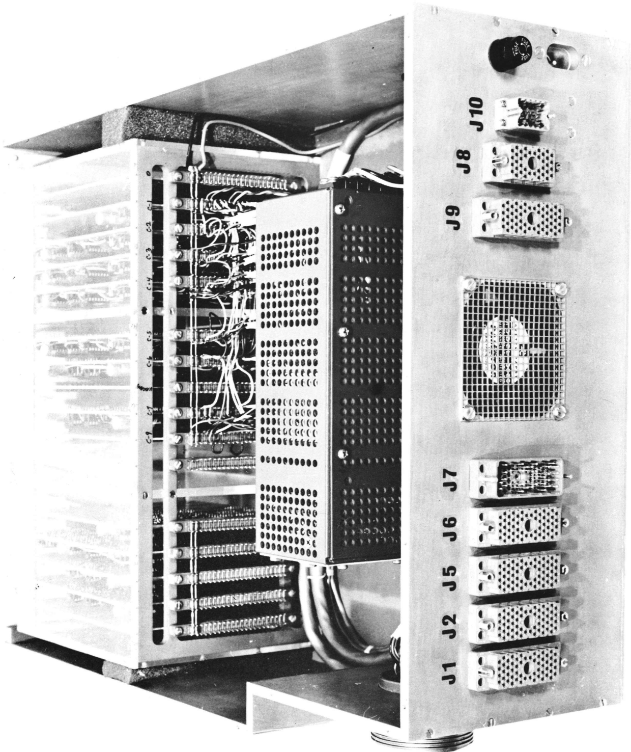
2. Computer interface box, back view.
