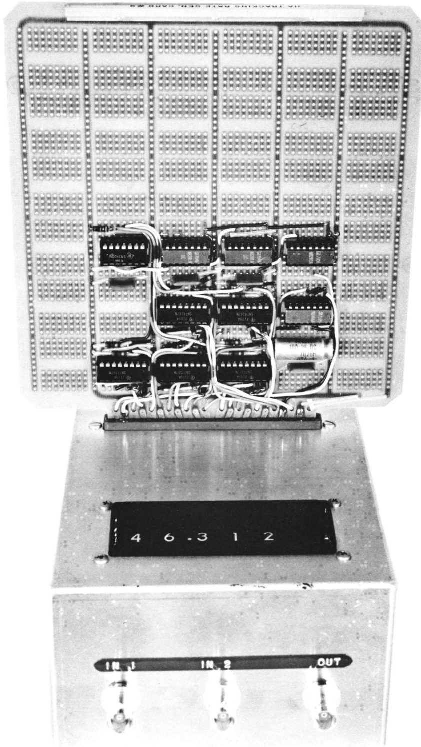
5. Manual rate generator and test set.
