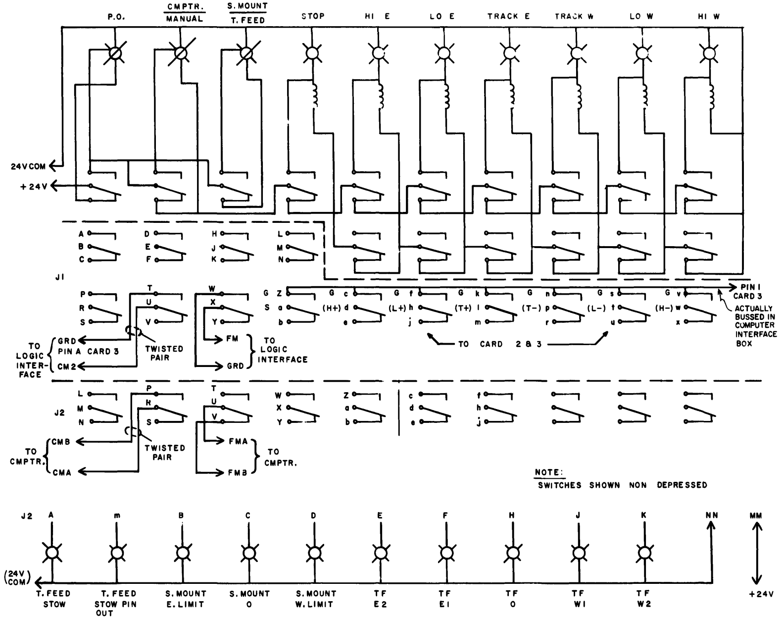
SCHEMATIC 1
