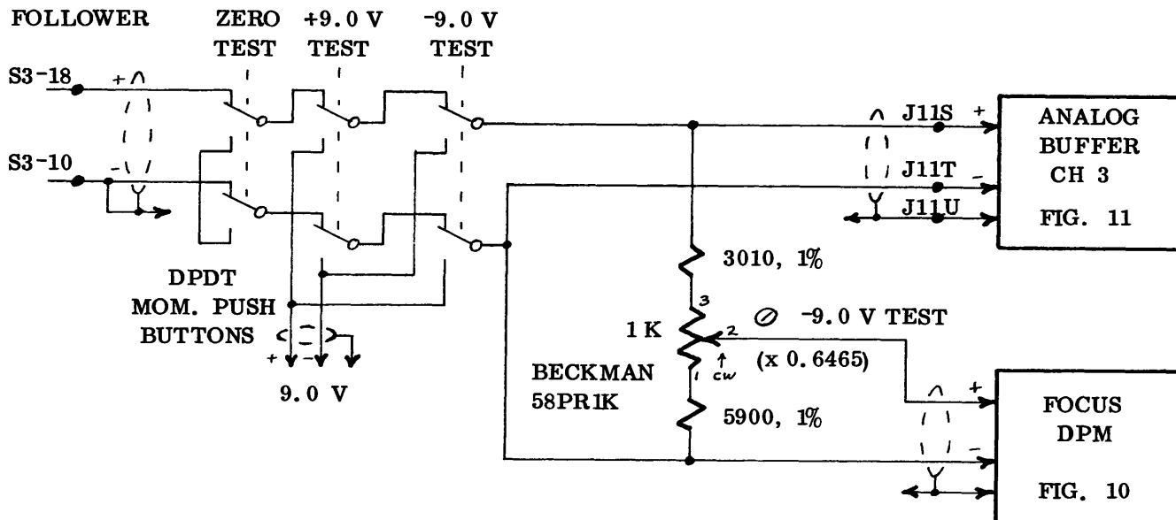
ROTATION AND FOCUS READOUT: CALIBRATION INSERTION AND ADJUSTMENT CIRCUITS
