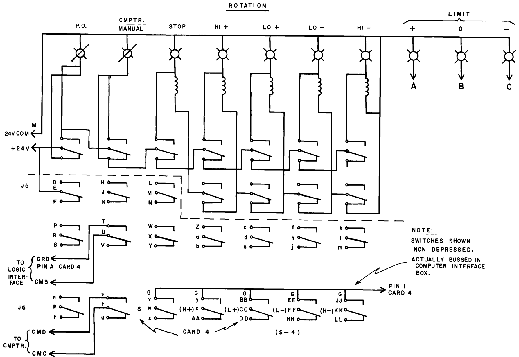
STERLING MOUNT ROTATION CONTROL PANEL: SCHEMATIC
