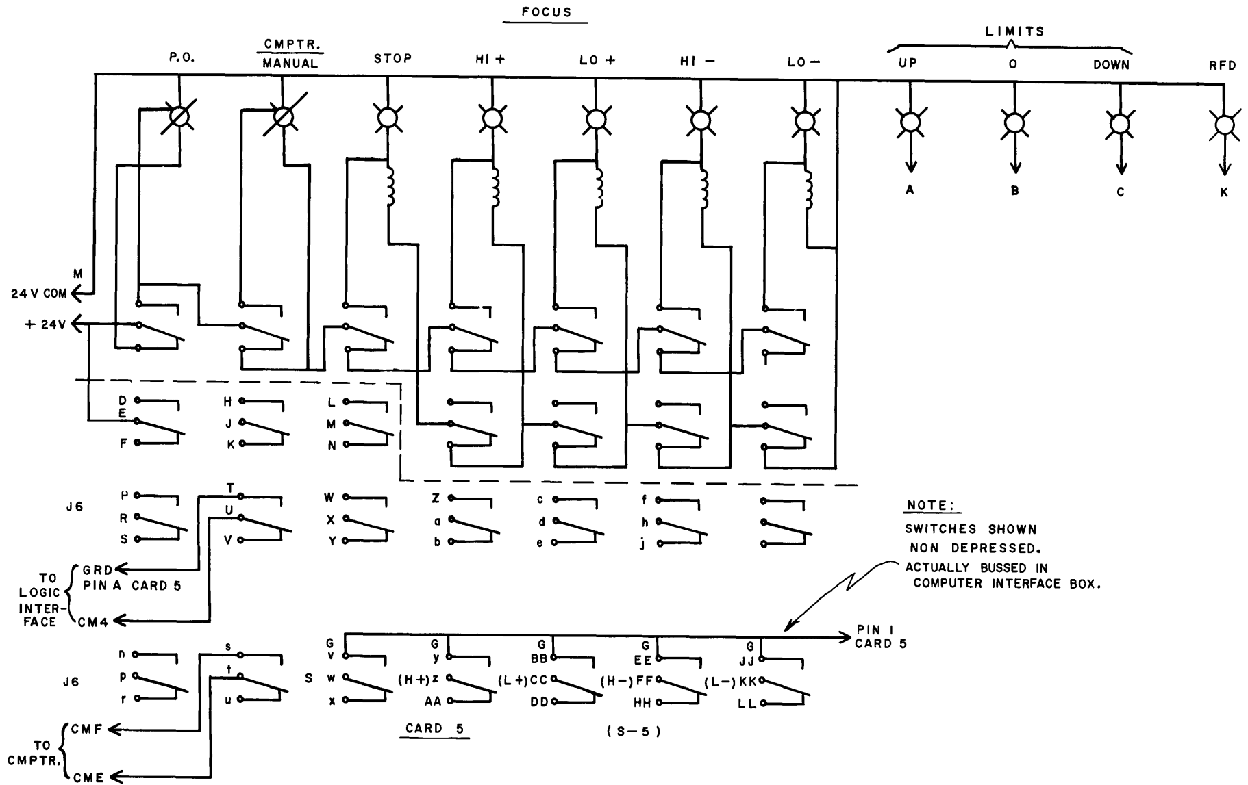
STERLING MOUNT FOCUS CONTROL PANEL: SCHEMATIC
