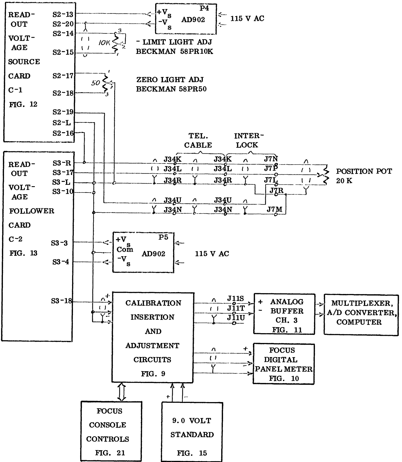
POSITION READOUT CIRCUIT: STERLING MOUNT FOCUS
