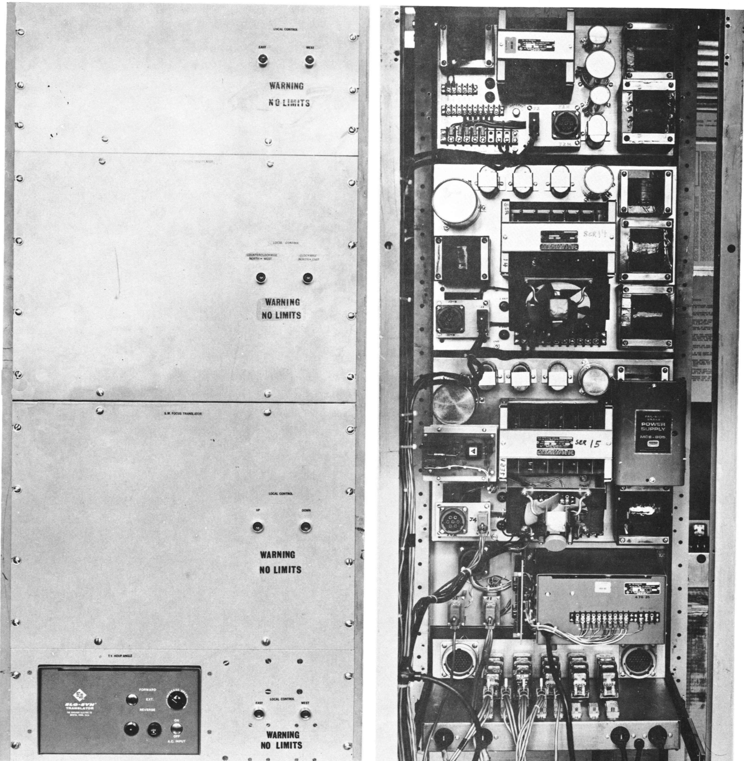
TRANSLATORS IN TELESCOPE FOCAL CABIN: SM HOUR ANGLE, ROTATION, FOCUS, TF HOUR ANGLE AND INTER-LOCK FROM TOP TO BOTTOM
