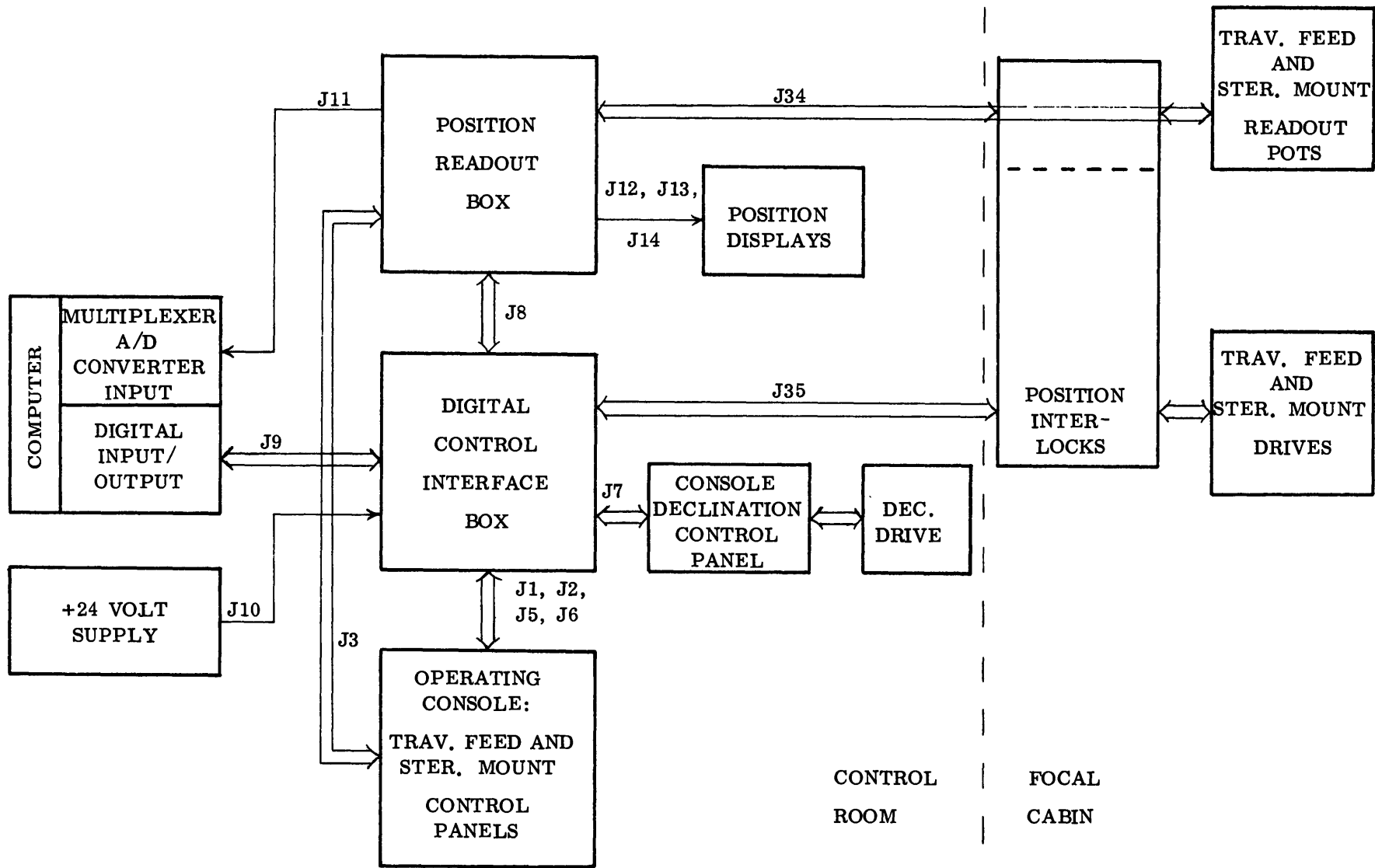
SIMPLIFIED BLOCK DIAGRAM OF TOTAL 300-FT TELESCOPE POINTING CONTROL SYSTEM
