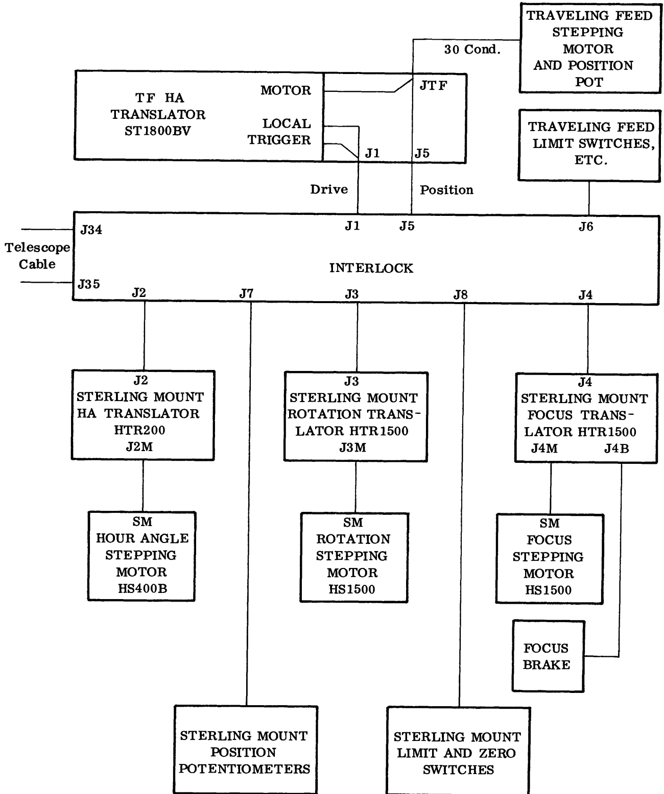
INTERLOCK: INTERCONNECTION BLOCK DIAGRAM
