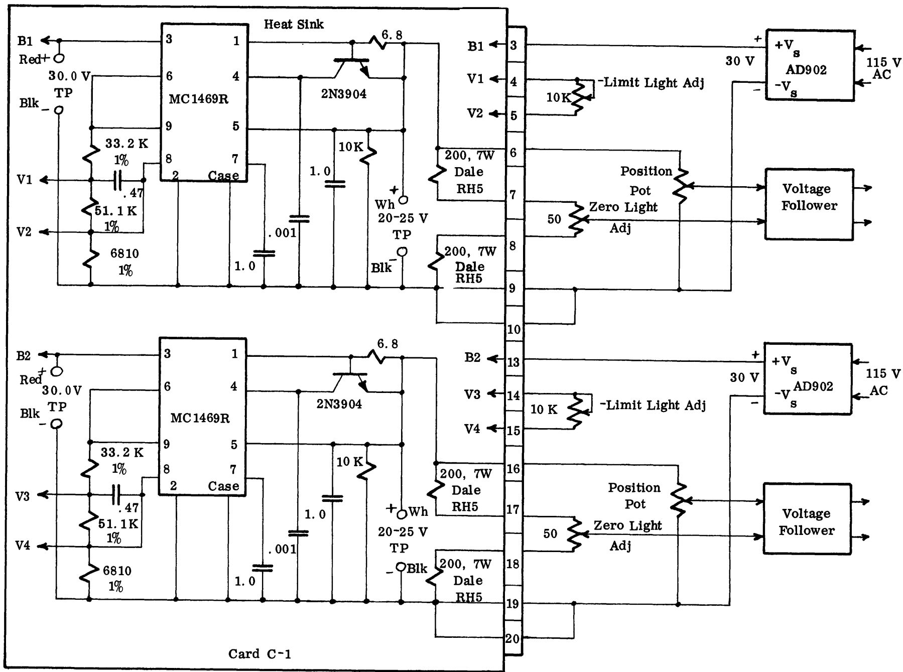
READOUT VOLTAGE SOURCE CARD C-1
