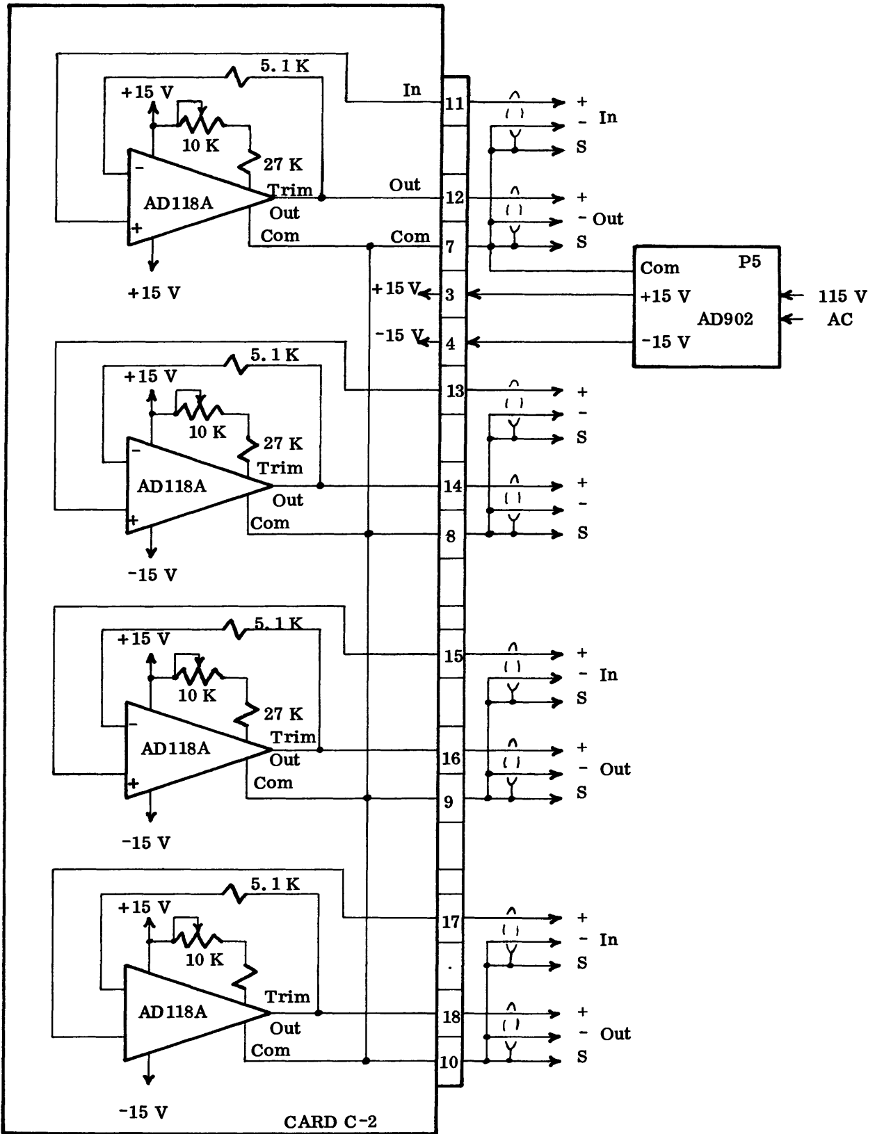
READOUT VOLTAGE FOLLOWER CARD C-2
