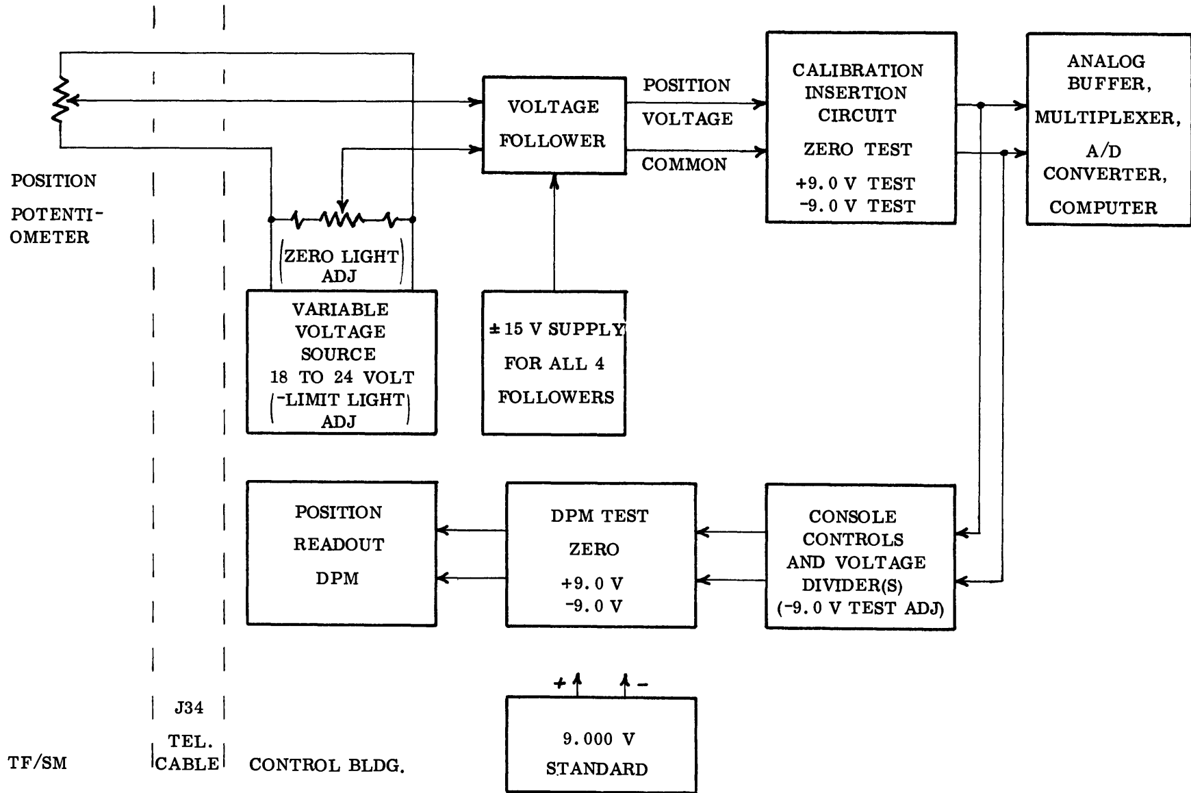
POSITION READOUT CIRCUIT: TYPICAL BLOCK DIAGRAM
