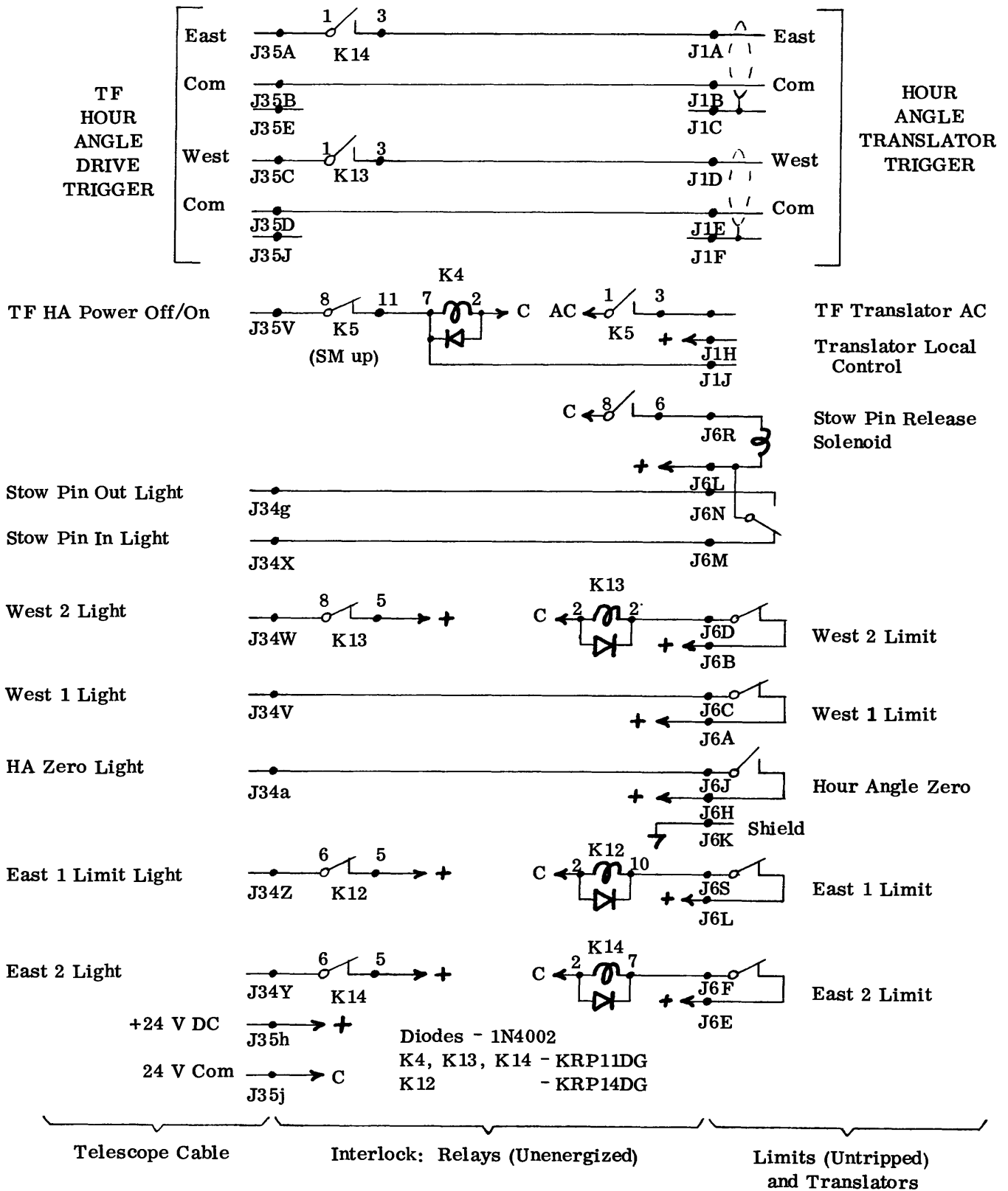
INTERLOCK CIRCUIT: TRAVELING FEED
