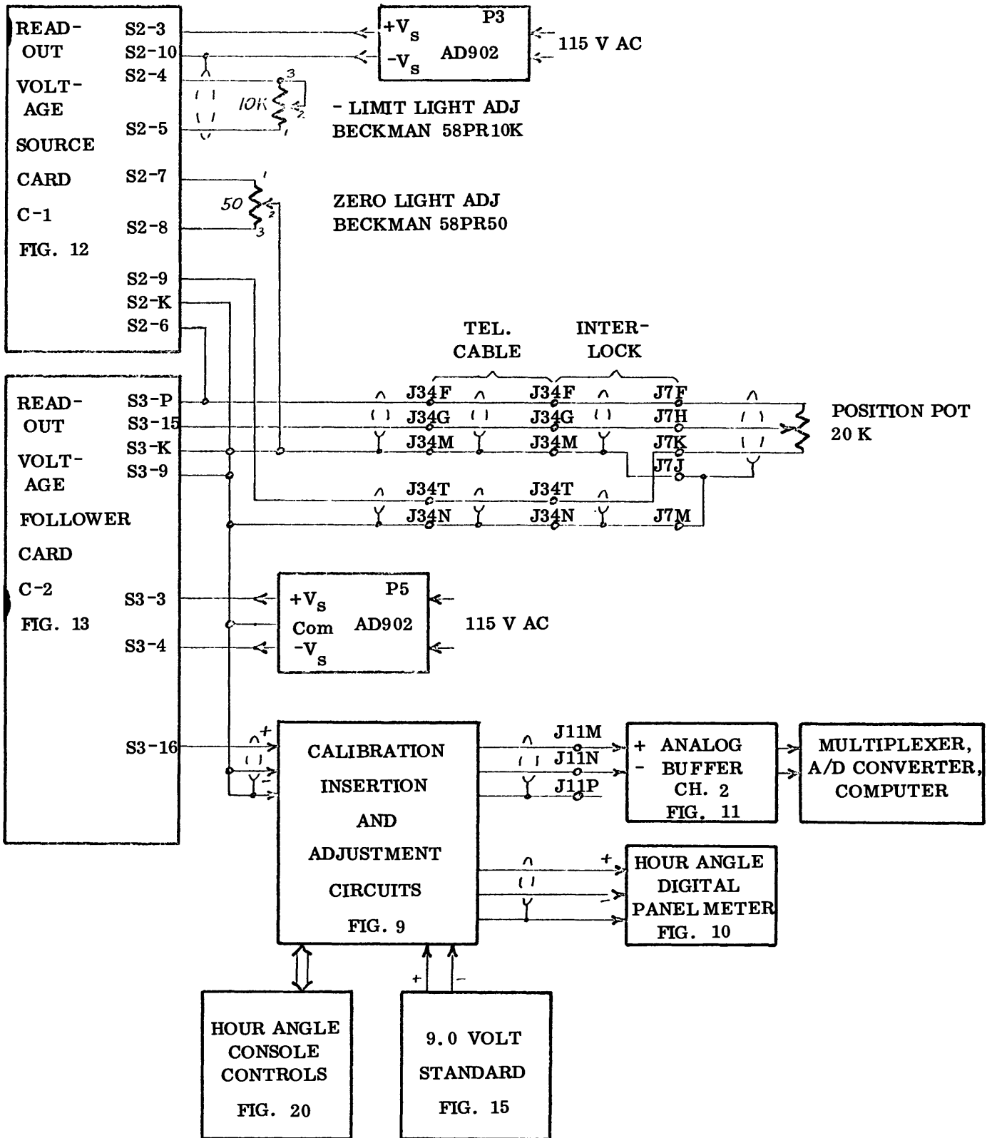
POSITION READOUT CIRCUIT: STERLING MOUNT ROTATION
