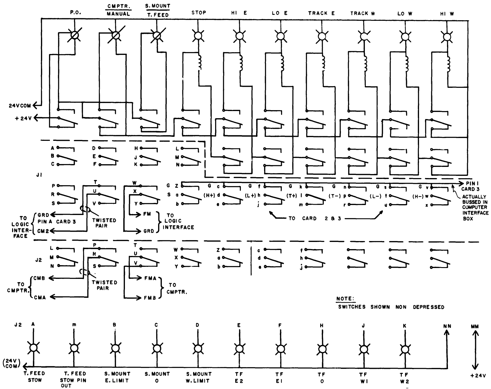
CONSOLE CONTROL PANEL: SCHEMATIC
