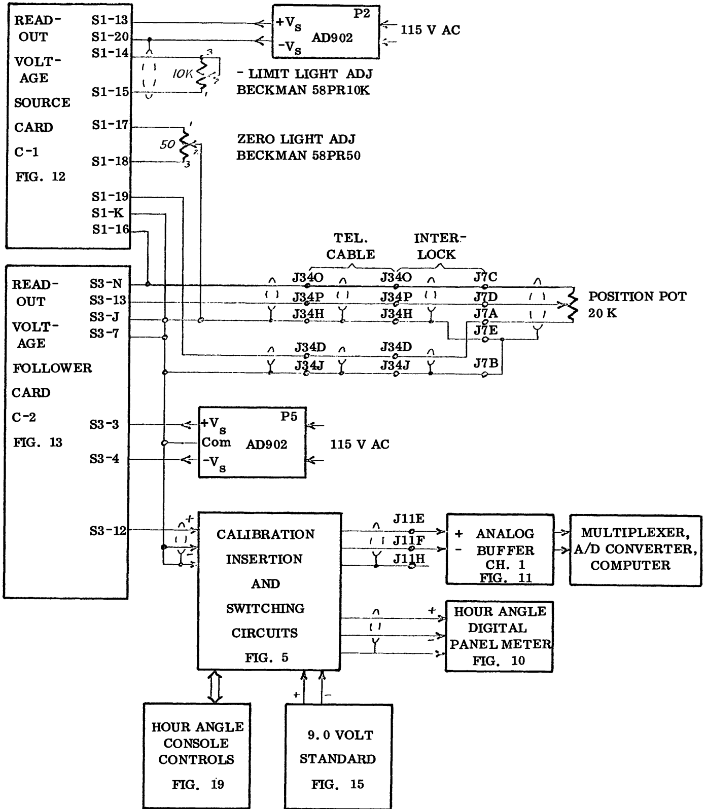
POSITION READOUT CIRCUIT: STERLING MOUNT HOUR ANGLE
