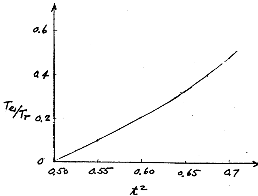
Fig. 3. Excess noise T_{el}/T_r vs power transmission factor t^2 .
