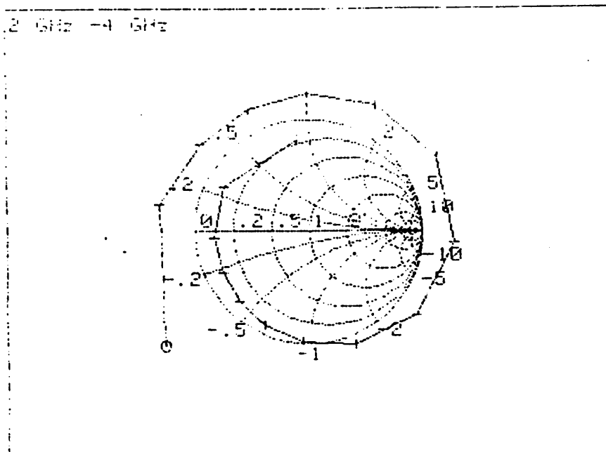
Fig. 10. The input impedance.
