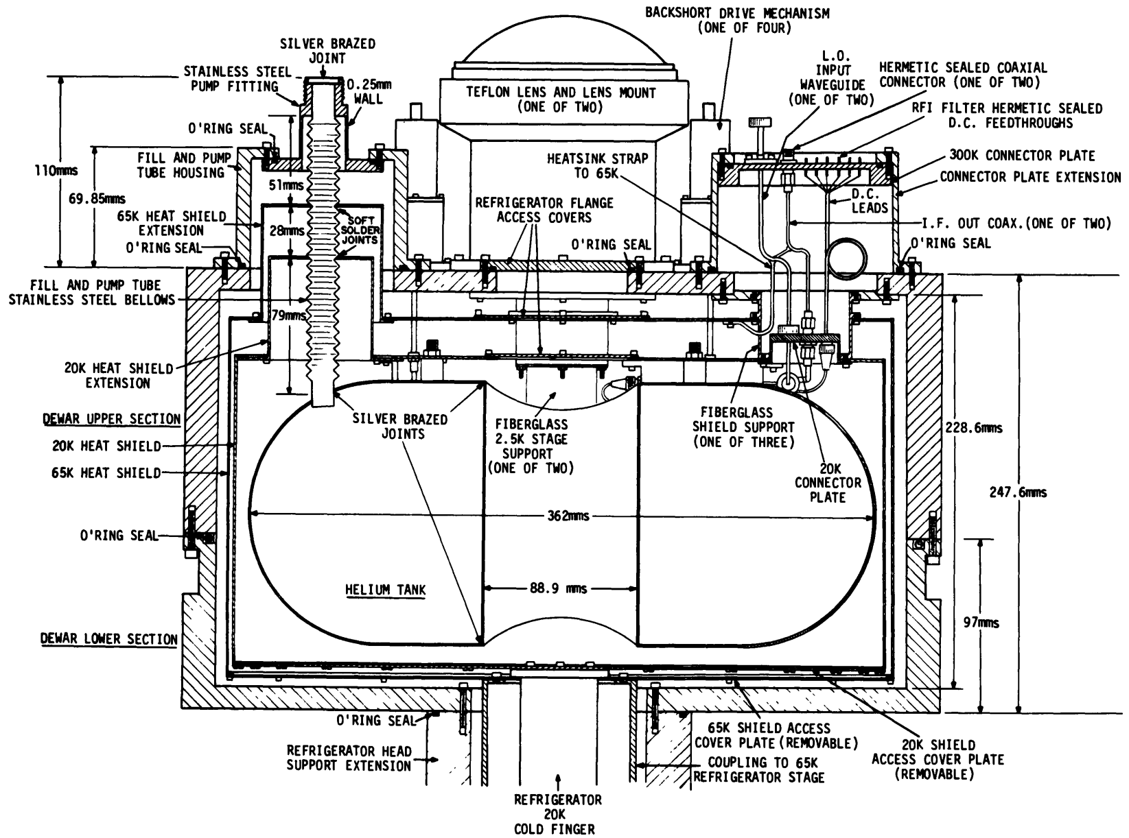
Fig. 2. Cross-sectional view of the complete dewar assembly along the diagonal AA shown in Figure 1. This sketch shows the tank mounting arrangement, heat shield locations and fill/pump tube configuration.
