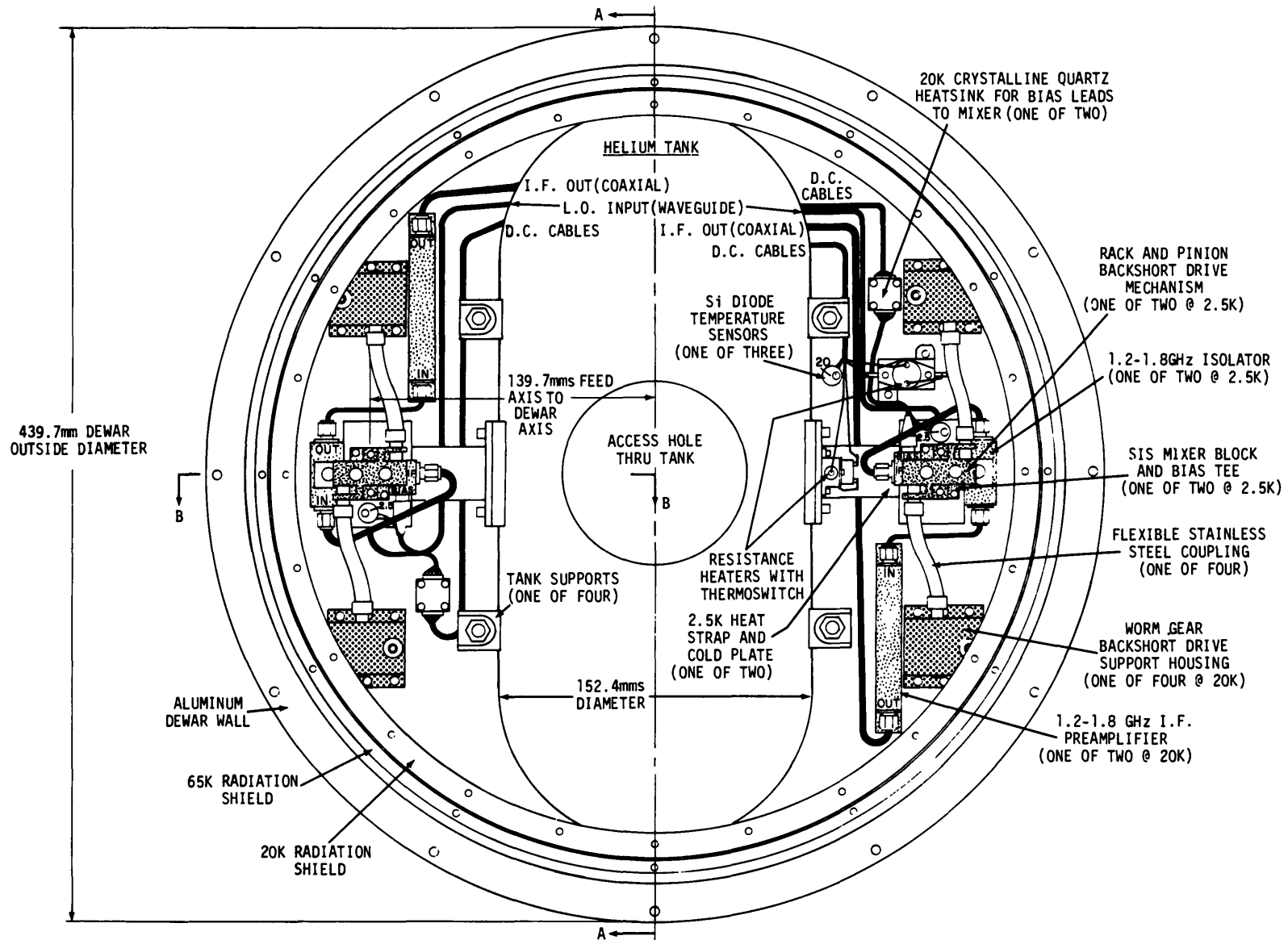
Fig. 1. A view of the interior of the top section of the vacuum dewar after the radiation shield covers have been removed.
