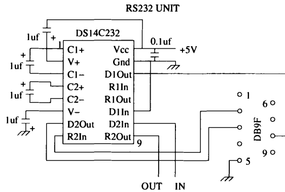
Figure 3: Schematic diagram of RS232 interface circuit.
