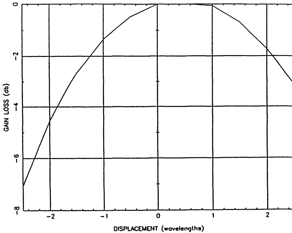
Fig. 3. Gain loss vs. displacement of M1 along 38.79° axis at 1.42 GHz.
