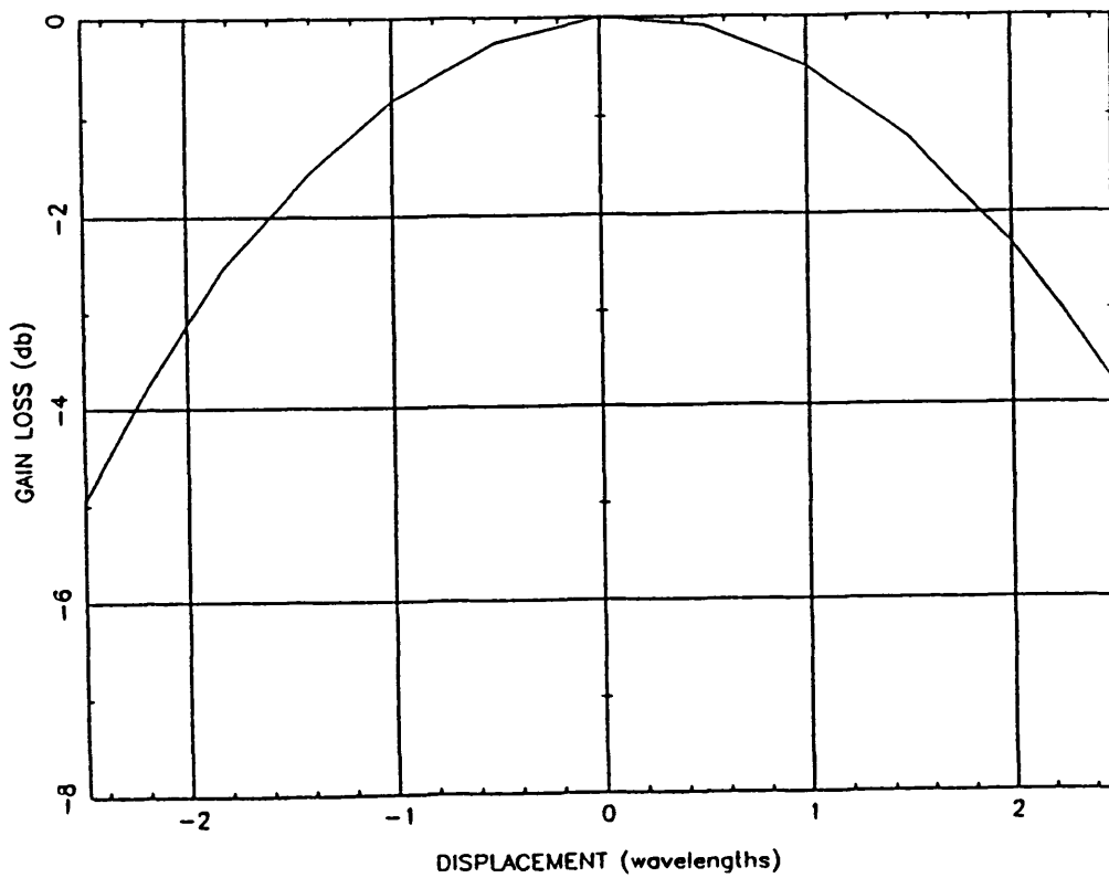
Fig. 4. Gain loss vs. displacement of M2 along 38.79° axis at 5 GHz.
