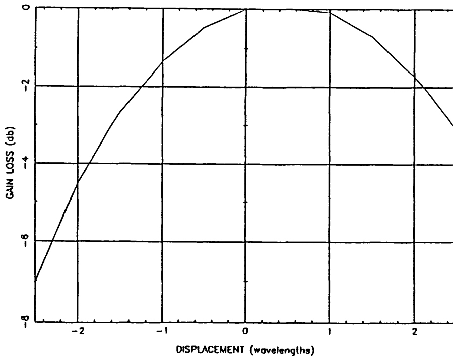
Fig. 2. Gain loss vs. displacement of M1 along 36.73° axis at 1.42 GHz.
