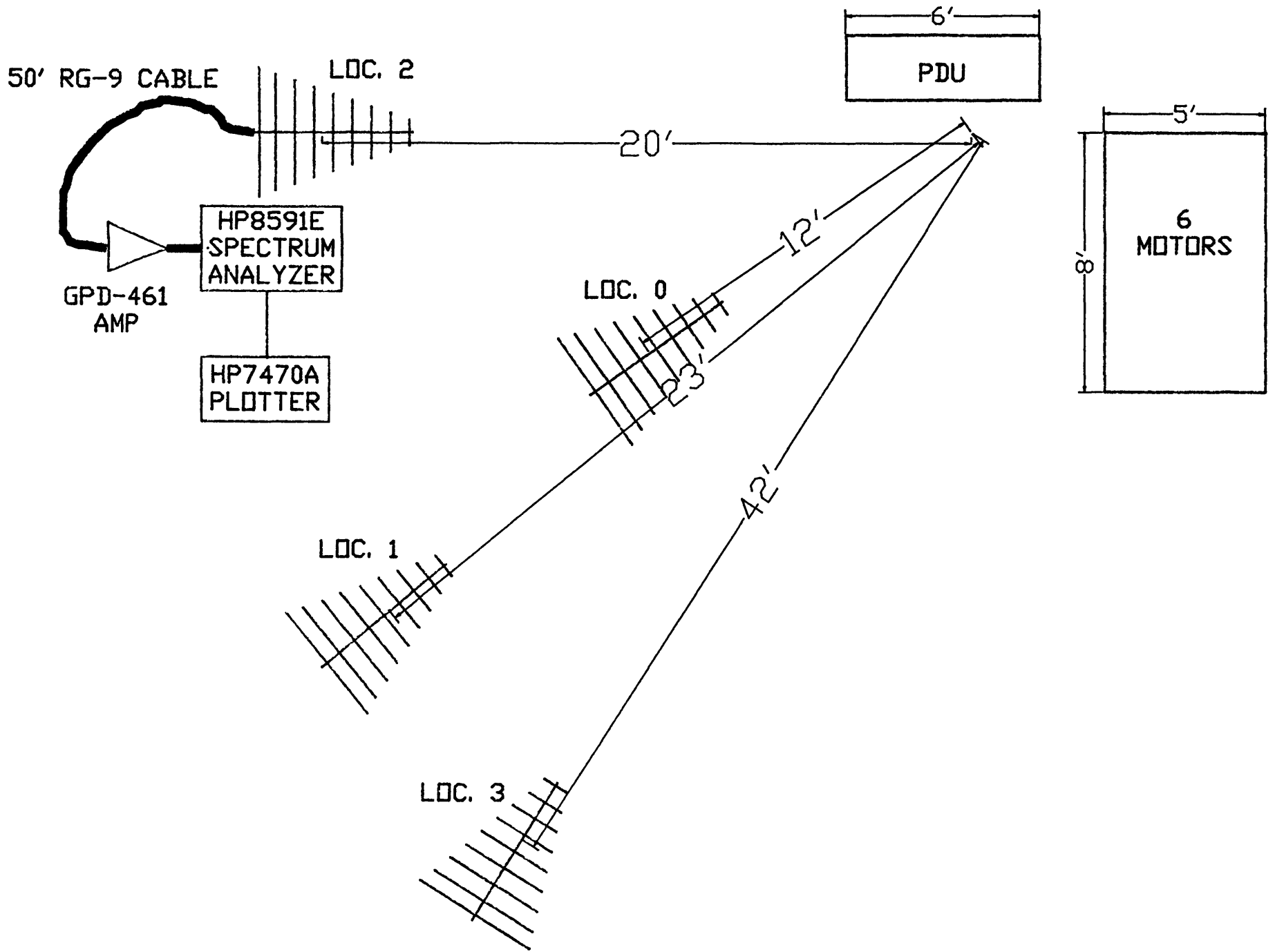
FIGURE 1: SET-UP FOR MEASURING RFI FROM PDU AND MOTORS.
