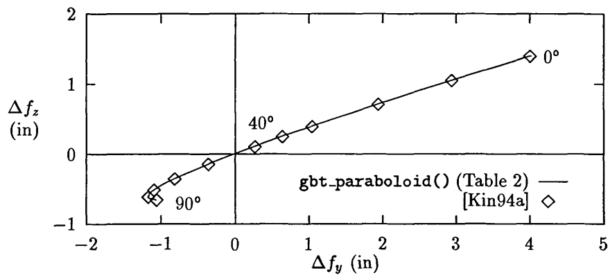
Figure 7: Prime-Focal-Point trajectory as a function of Elevation
