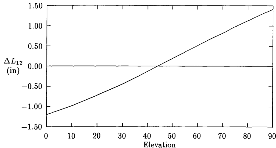
Figure 10: BFP-to-GregorianFeed distance minus 11 meters
