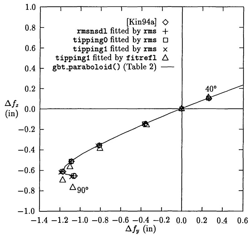
Figure 3: Six Prime-Focal-Point Trajectories
