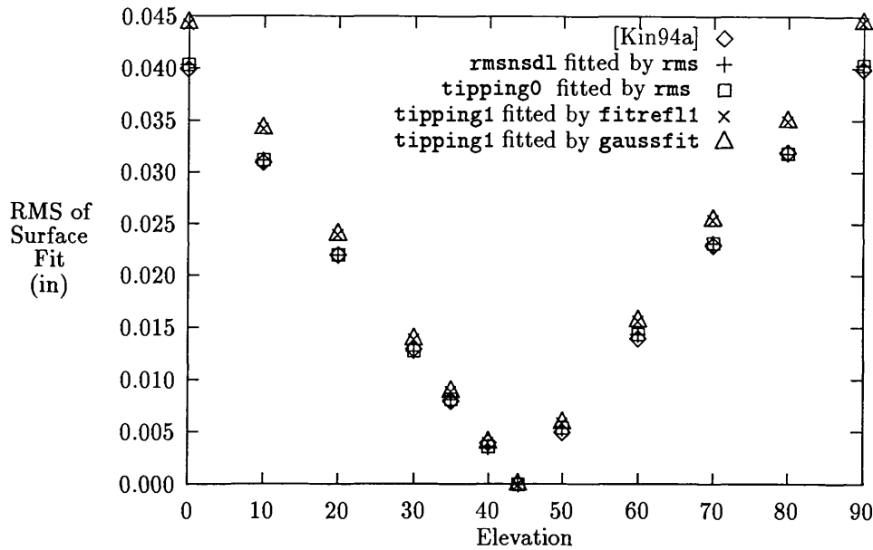
Figure 2: RMS-of-Fit as a function of Elevation
