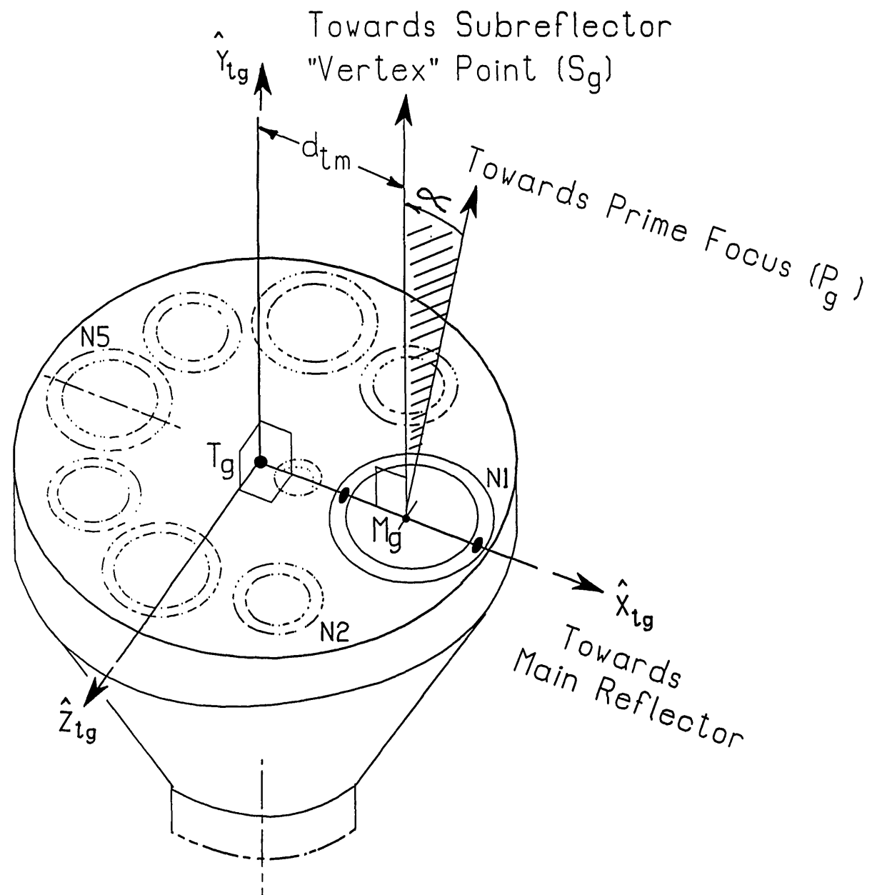
Figure 5. The Turret Frame.
