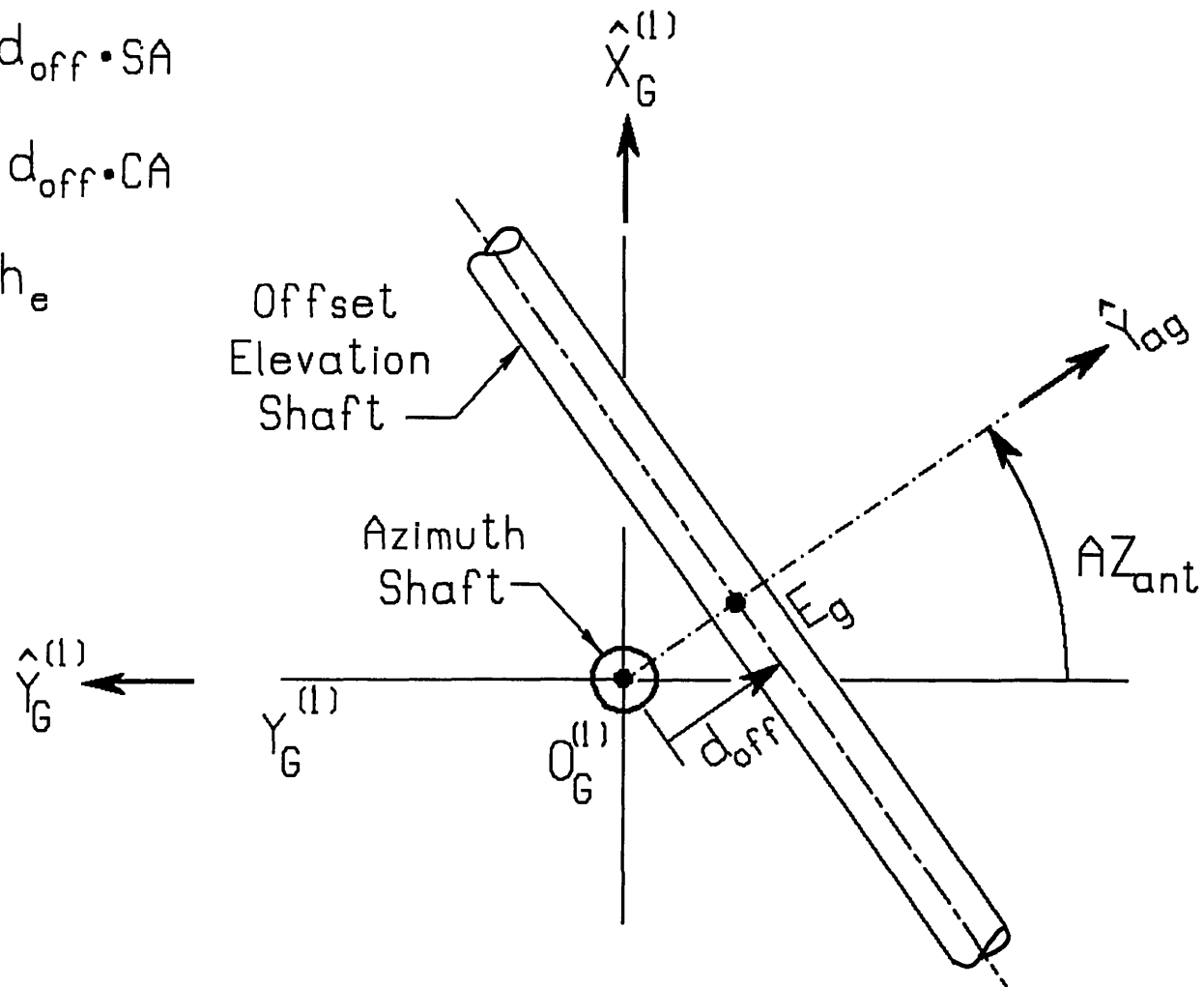
Figure 9. Ground Frame Coordinates Of The Offset Elevation Frame's Origin Point
