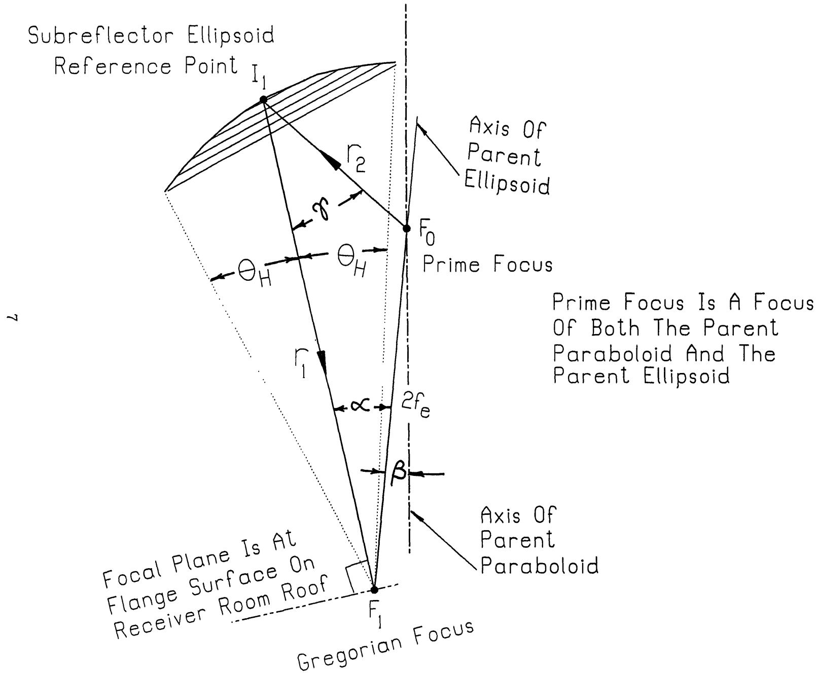
Figure 1. The Subreflector Ellipsoid Reference Geometry
