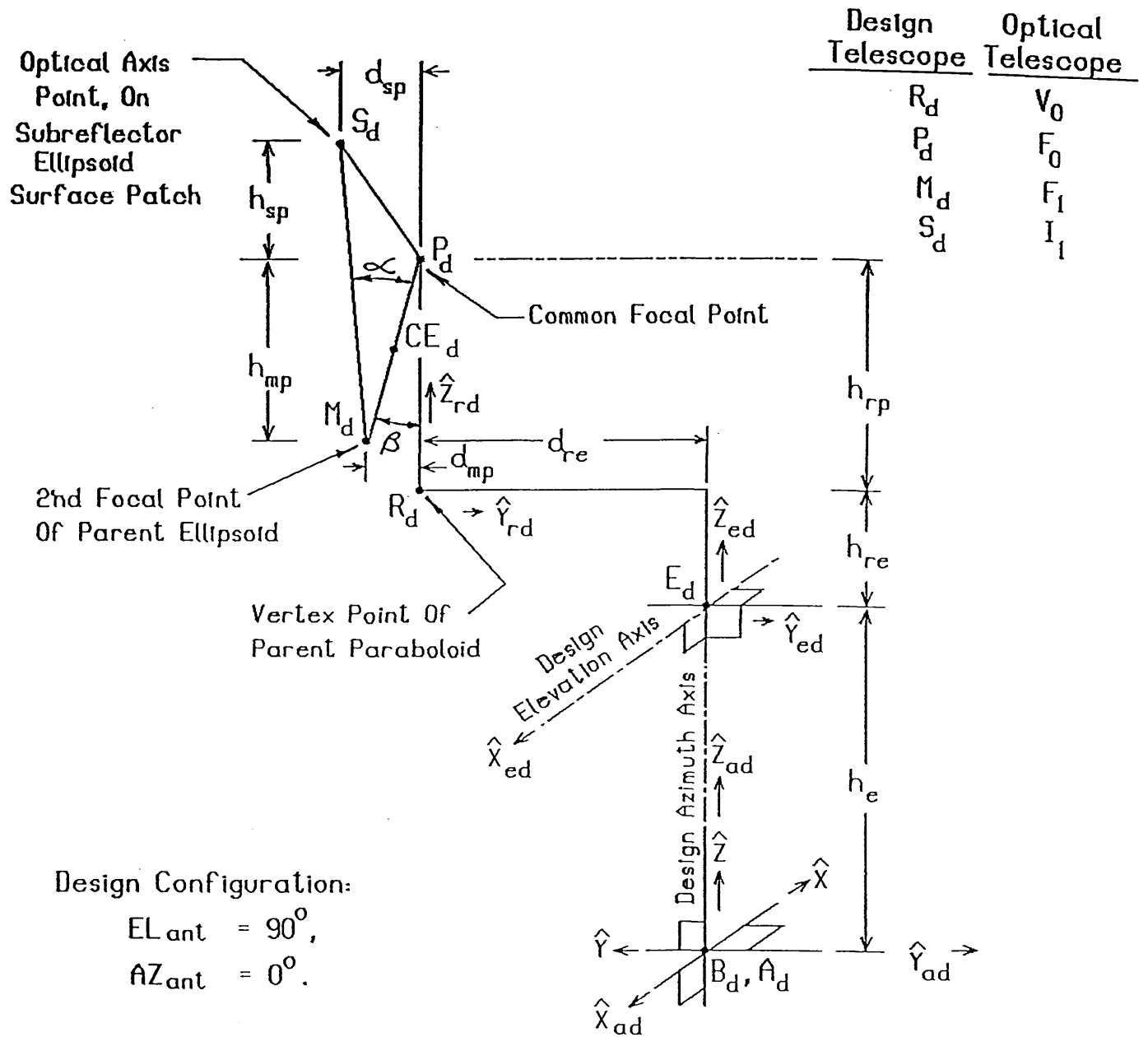
Figure 2. Design Telescope Reference Points
