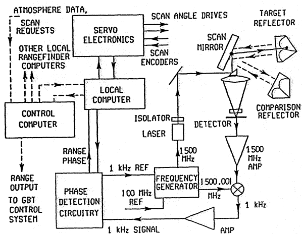
Fig. 3. Block Diagram of Rangefinder
