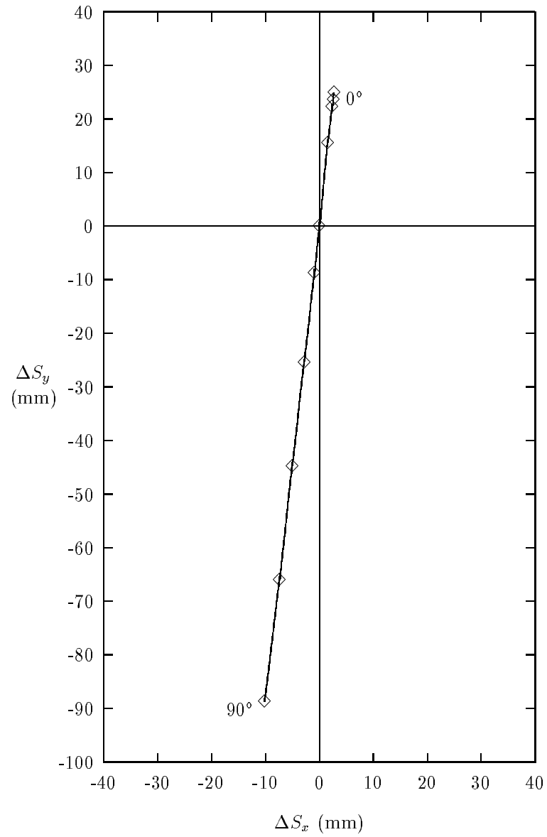
Figure 4: Focus tracking 'center' trajectory in ray-tracing coordinates (Table 1) [1:1 scale]
