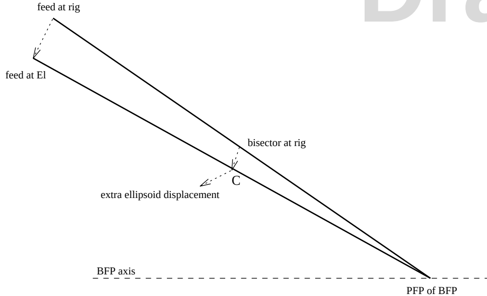
Figure 3: Center-Offset of the Subreflector [Step 11]
