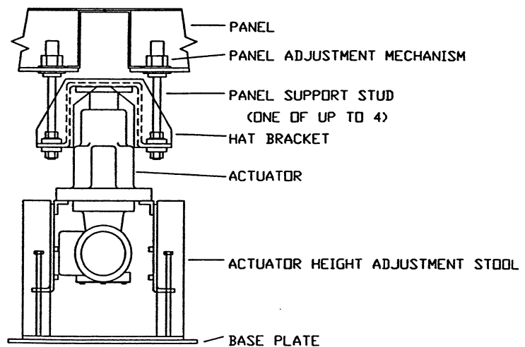
Figure 2: Mechanical configuration of the panel actuators.
