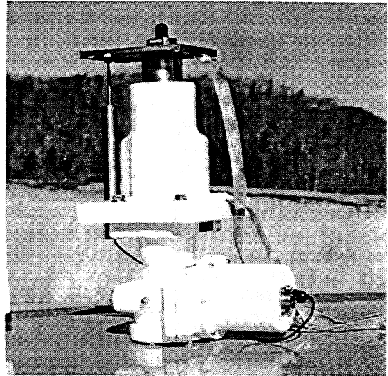
Figure 4: Photograph of a panel actuator.
