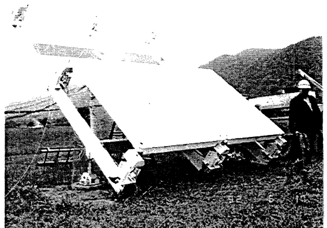
Figure 7: Four panel, nine actuator test jig used for testing production actuators.
