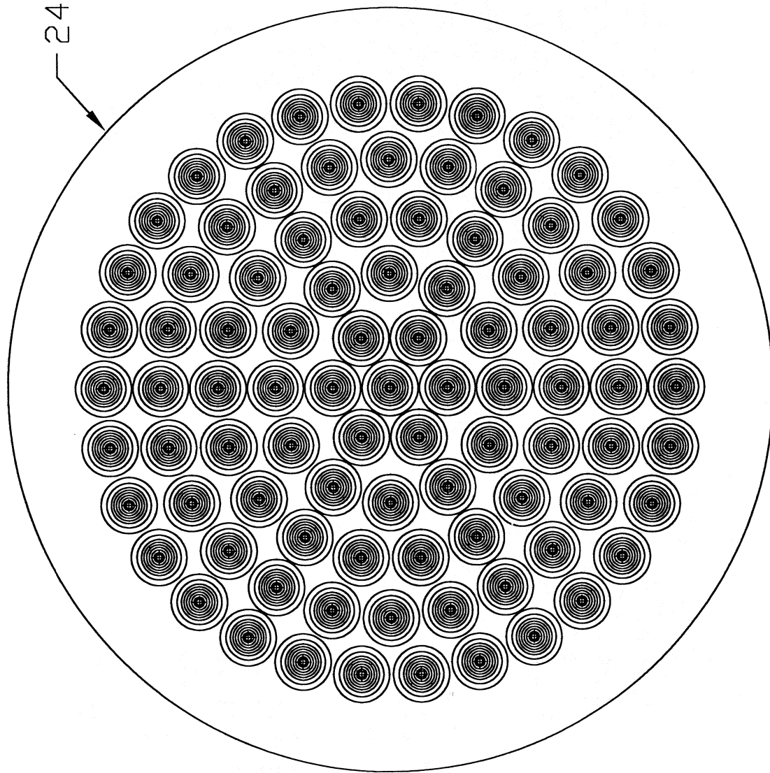
FIGURE 1 ARRAY OF 91 7mm FEEDS, OUTER RING AT 22.5cm OFFSET, FEED OD 4.5cm.
