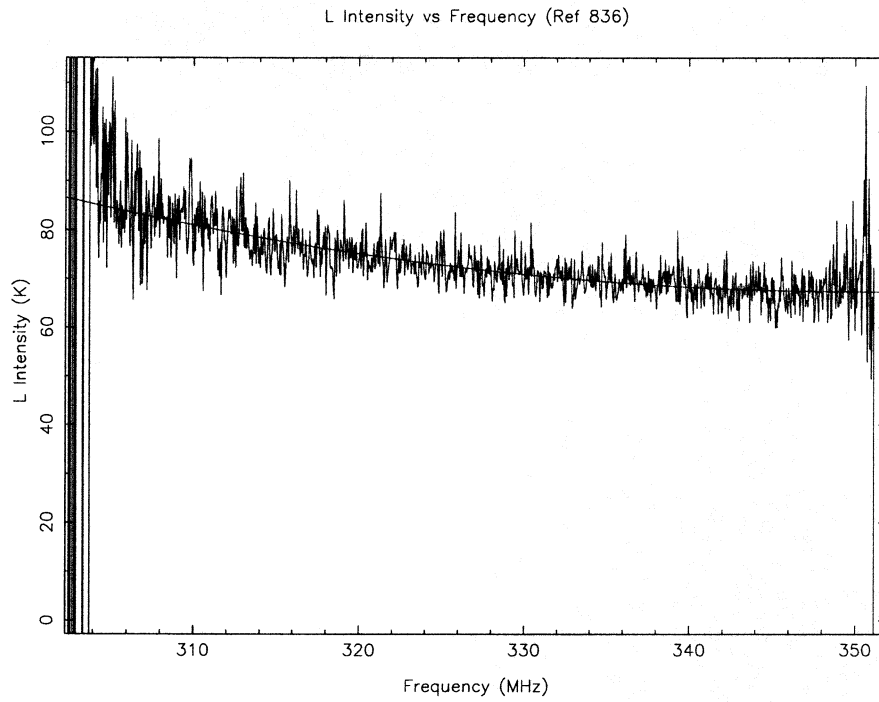
Figure 14: LCP spectrum measured for the system temperature of the reference scan. A second order polynomial was fit to the data.
