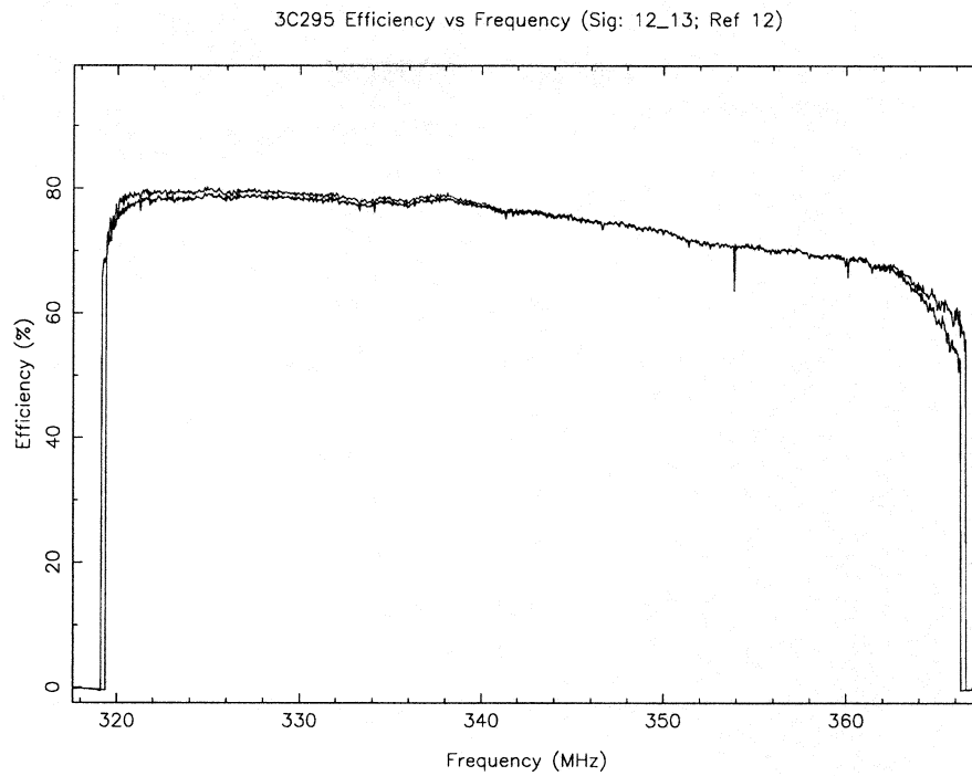
Figure 6: Measured GBT Efficiency based on observations of 3C295. This and the following plots are produced by glish scripts: setFluxes() ; updateEfficiency()
