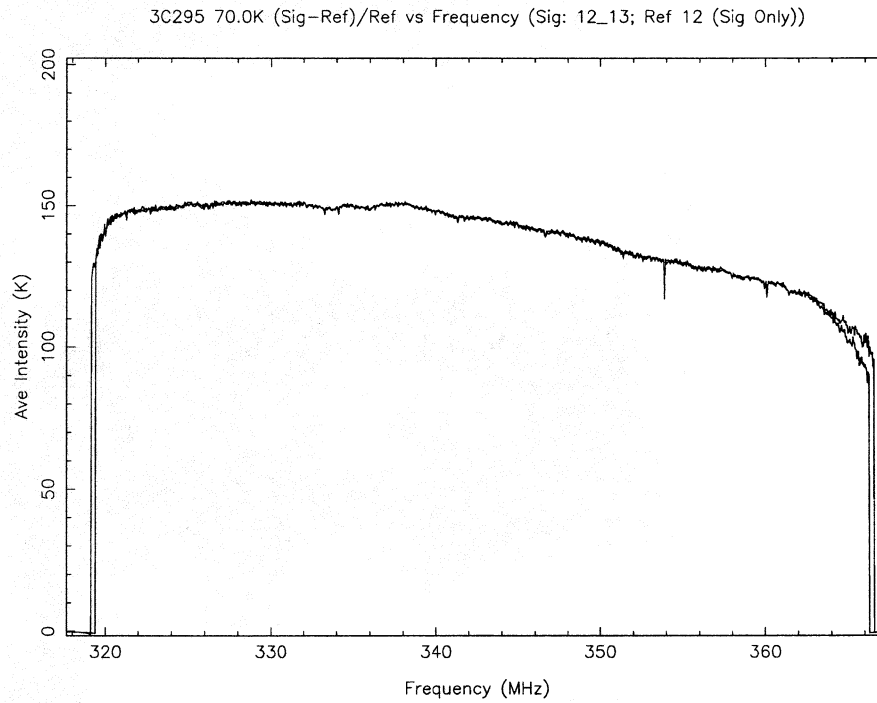
Figure 3: LCP and RCP spectra of 3C295 produced by T_{sys} \times (\text{Signal-Reference})/\text{Reference} calibration. This is the output of the flare([12,13],[12]) glish script, were scans 12 and 13 were processed. The reference scan number is 12. Notice the IF gain ripple is successfully calibrated out.
