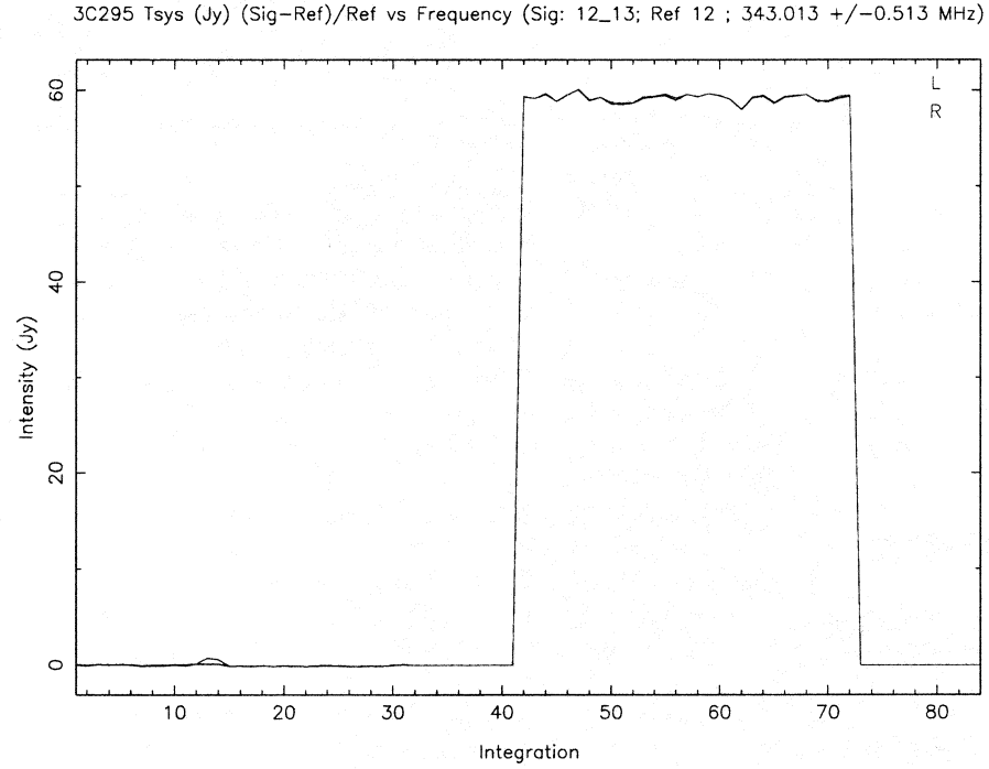
Figure 10: Average intensity versus time plot for the frequency range 342.5 to 343.5 MHz for reference and signal scans towards 3C295. The data are T_{sys} \times (Sig - Ref)/Ref calibrated separately for LCP and RCP data. The average reference spectra for this time range was subtracted from both reference and signal. There are 10 integrations with zero intensity after each scan.
