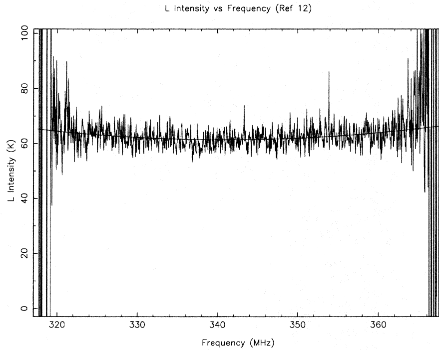
Figure 4: LCP spectrum measured for the system temperature of the reference scan, 12. A second order polynomial is fit to the data.
