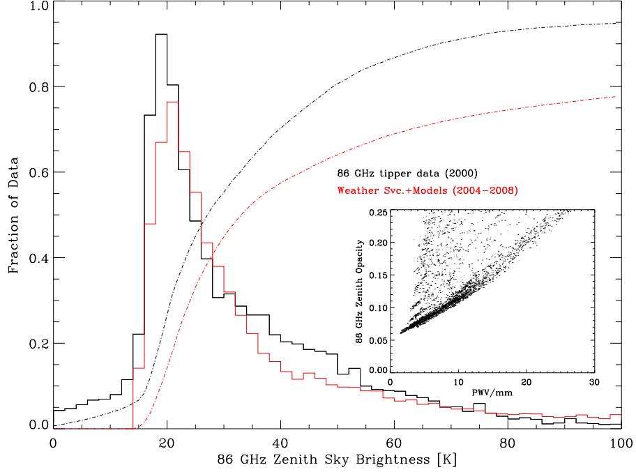
Figure 6: Distribution of 86 GHz zenith opacity measurements from the GB tipper in the year 2000, with NWS model-based predictions of the 86 GHz zenith opacity over the period 2004-2008. The tail of the tipper measurements below 15K zenith brightness results from measurements with large uncertainties; these are not edited so as to avoid biasing the distribution. (Data courtesy of Ron Maddalena)
