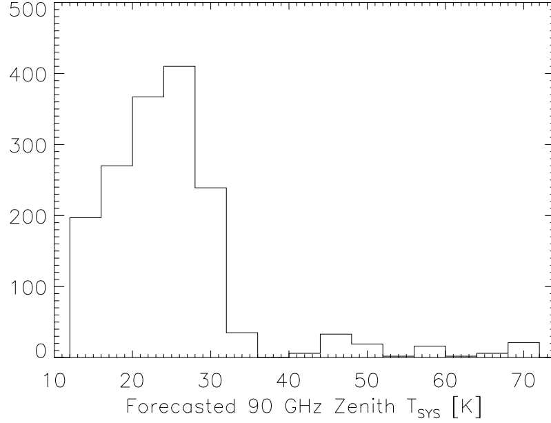
Figure 2: The distribution of forecast 90 GHz zenith system temperature due to the atmosphere and hydrosols for the scans in our analysis. 6.5% of scans have T_{sys} > 35 K.
