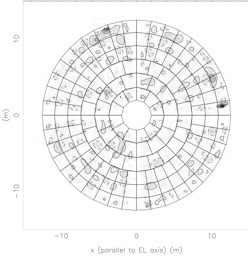
Figure 14: Antenna 14
