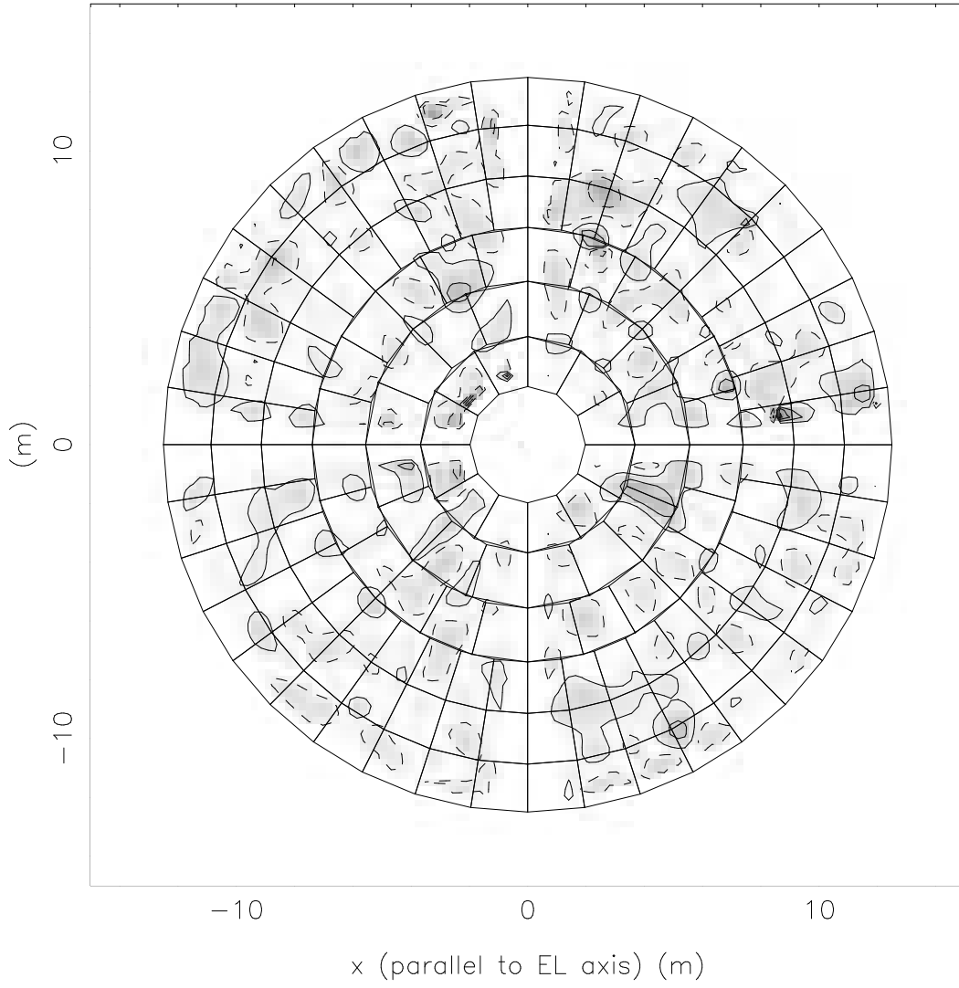
Figure 17: Antenna 17
