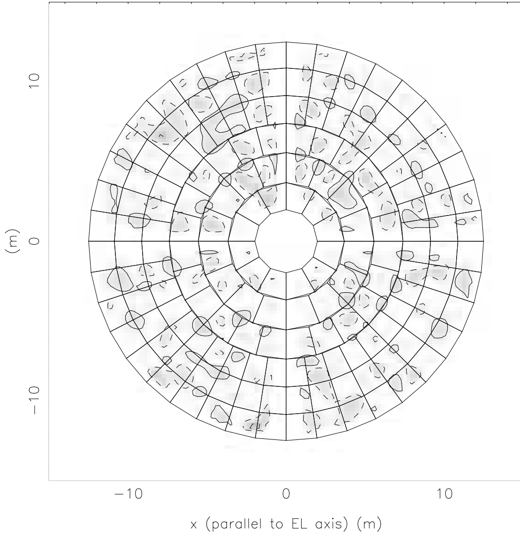
Figure 24: Antenna 24
