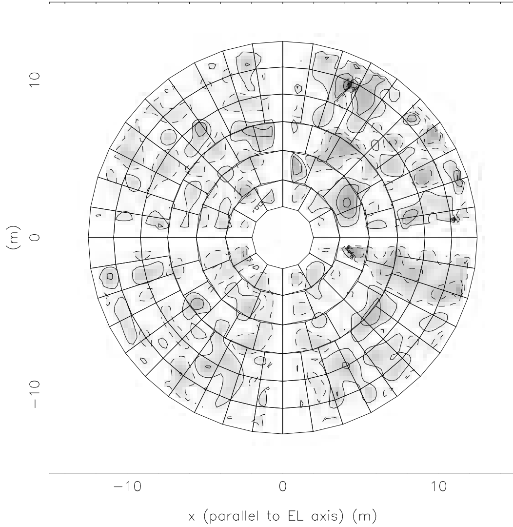
Figure 3: Antenna 3
