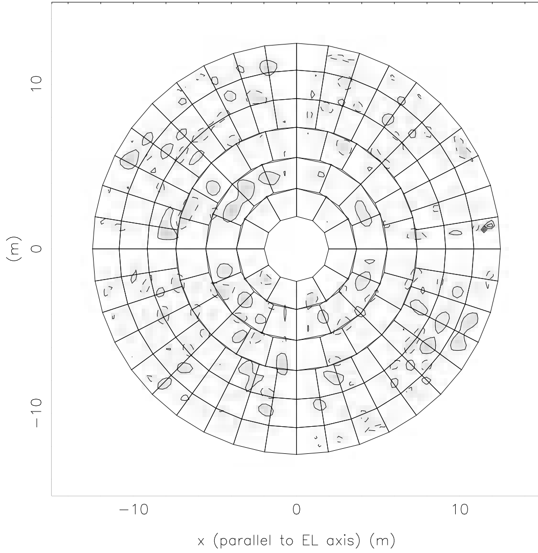
Figure 7: Antenna 7
