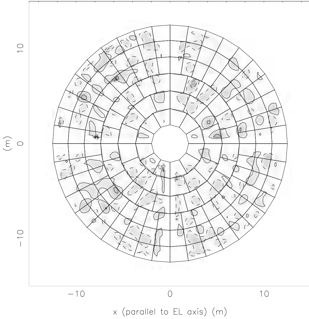
Figure 23: Antenna 23
