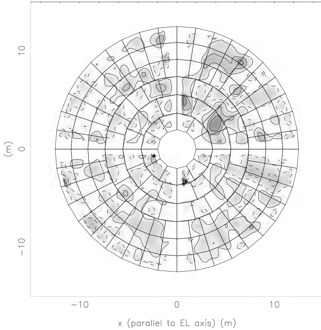
Figure 4: Antenna 4
