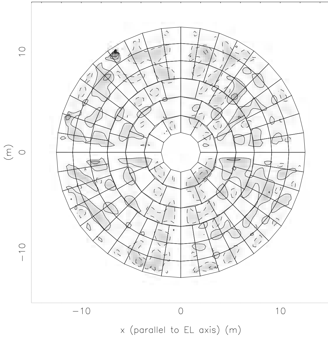
Figure 28: Antenna 28
