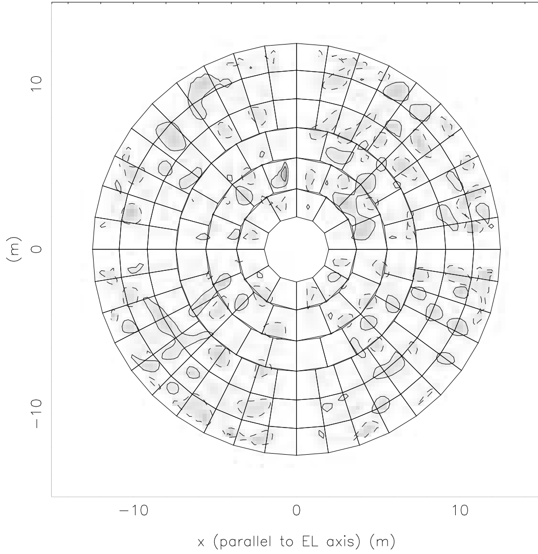
Figure 12: Antenna 12
