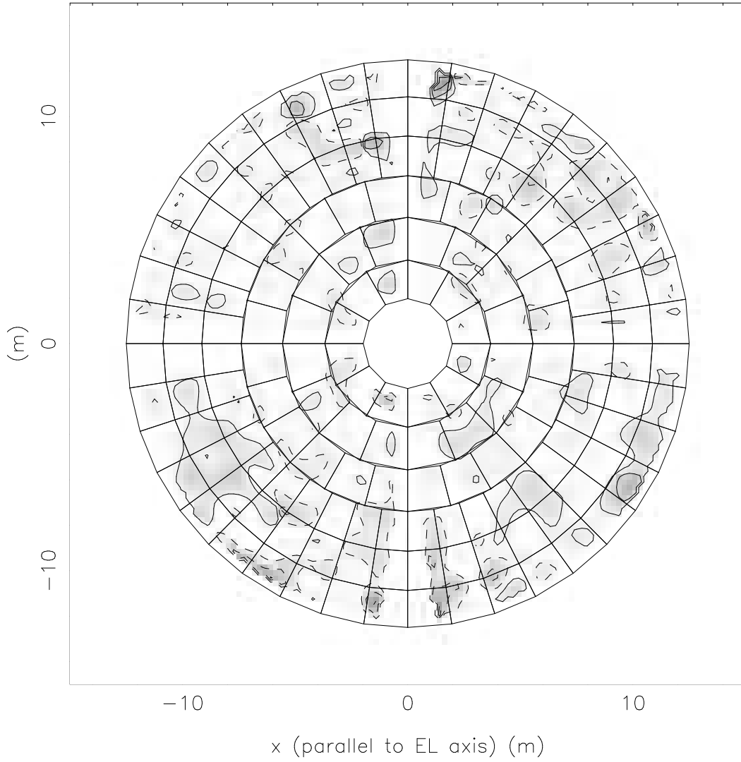
Figure 6: Antenna 6
