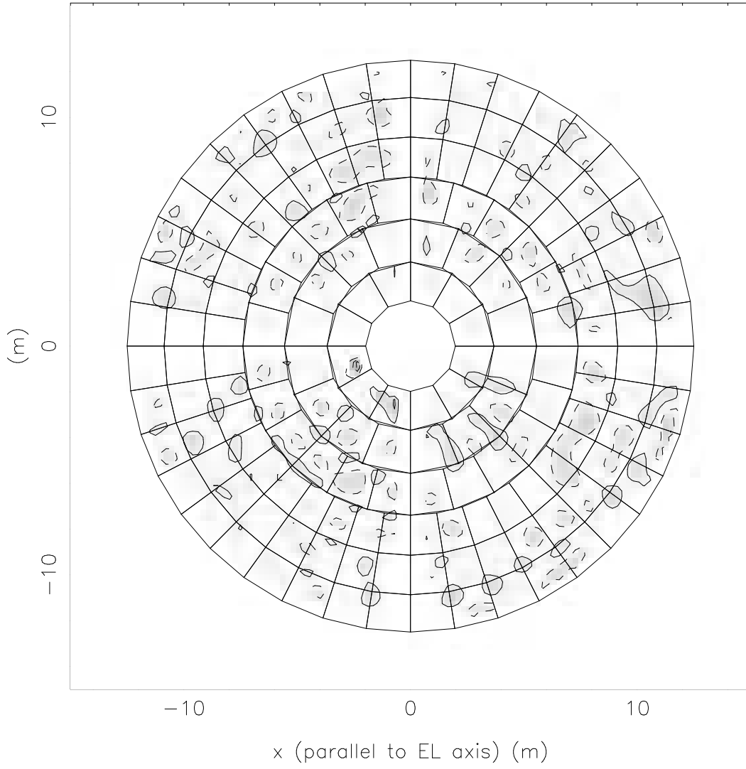
Figure 15: Antenna 15
