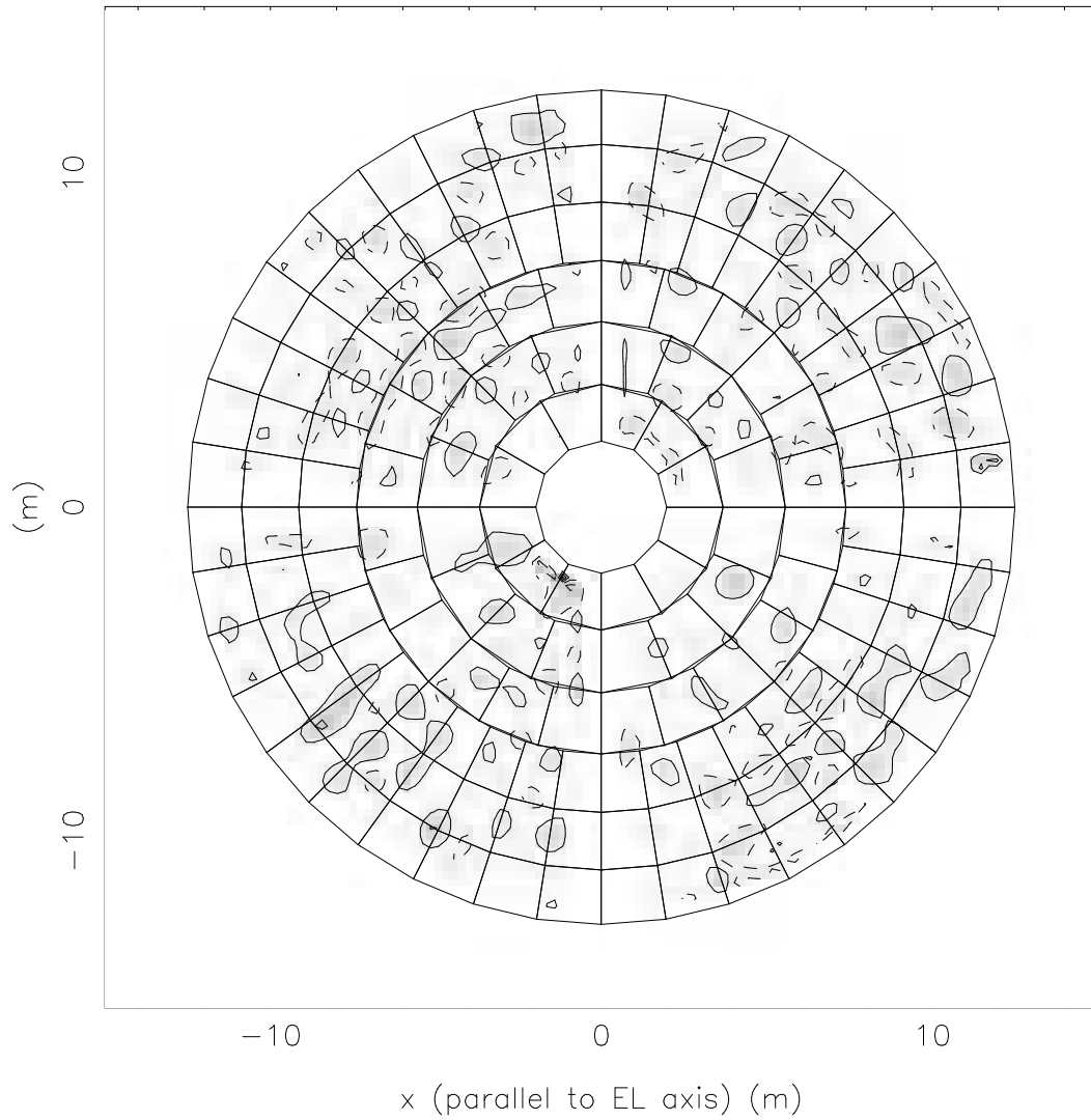
Figure 1: Antenna 1 – The antenna surface deviations based on 43 GHz holography. The date of the measurement is give in column 4 of Table 1. Contours are: -3.25, -2.75, -2.25, -1.75, -1.25, -0.75, -0.25, 0.25, 0.75, 1.25, 1.75, 2.25, 2.75, 3.25mm. Negative contours are dashed.
