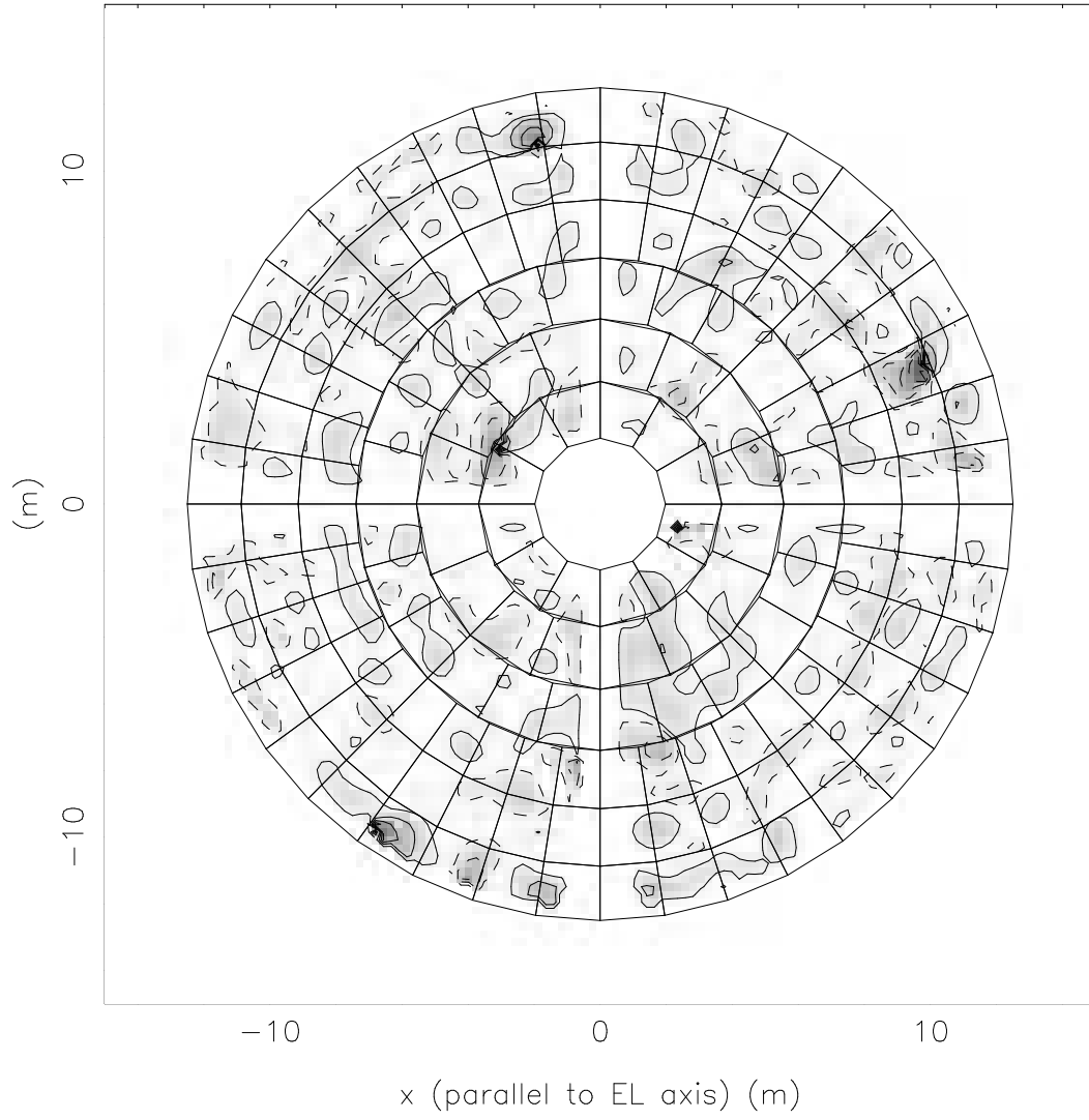
Figure 5: Antenna 5
