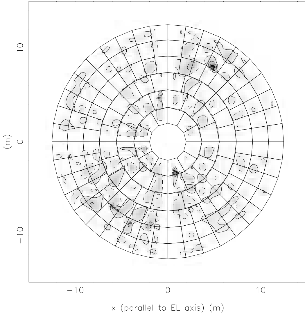
Figure 10: Antenna 10
