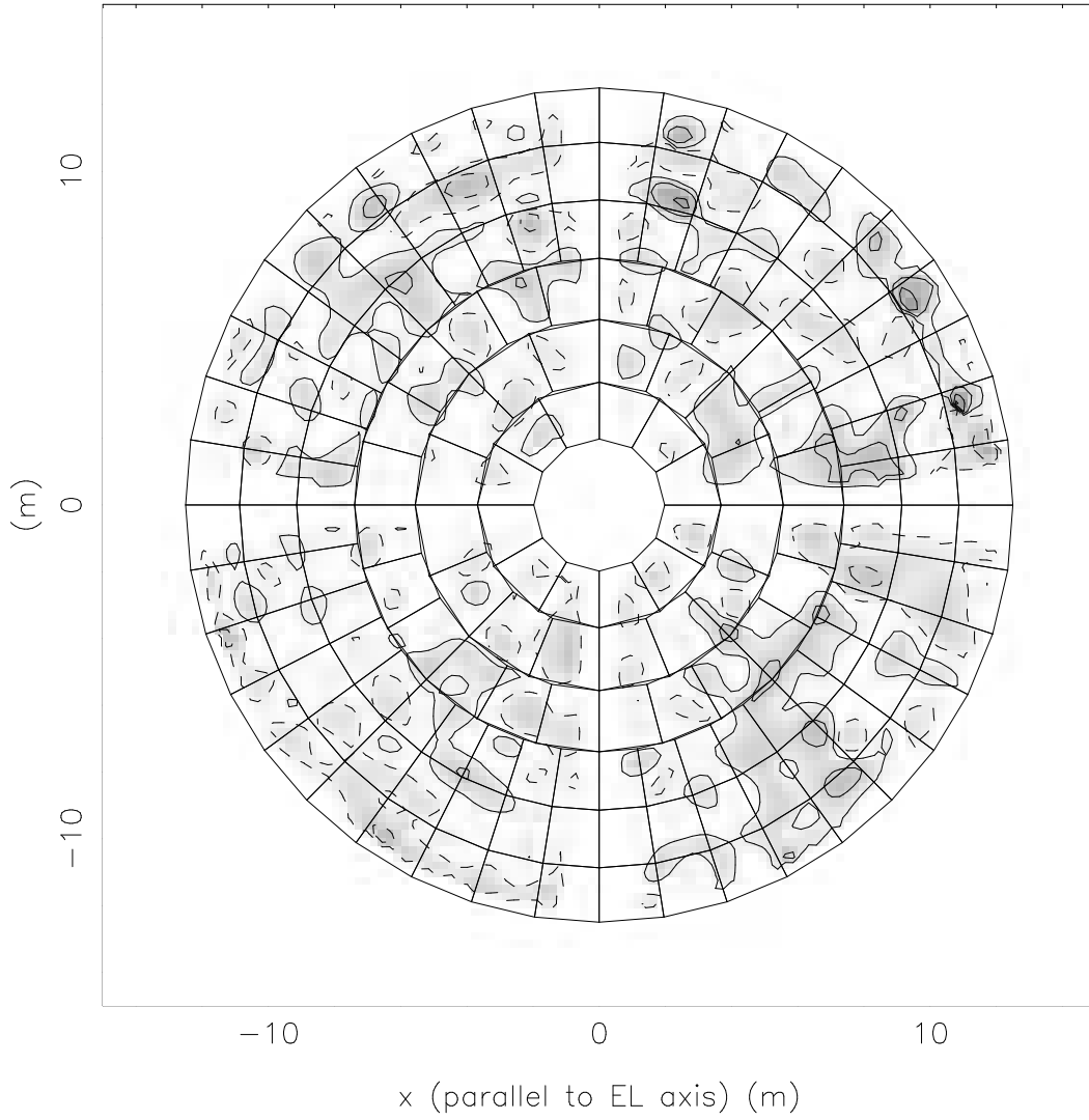
Figure 27: Antenna 27
