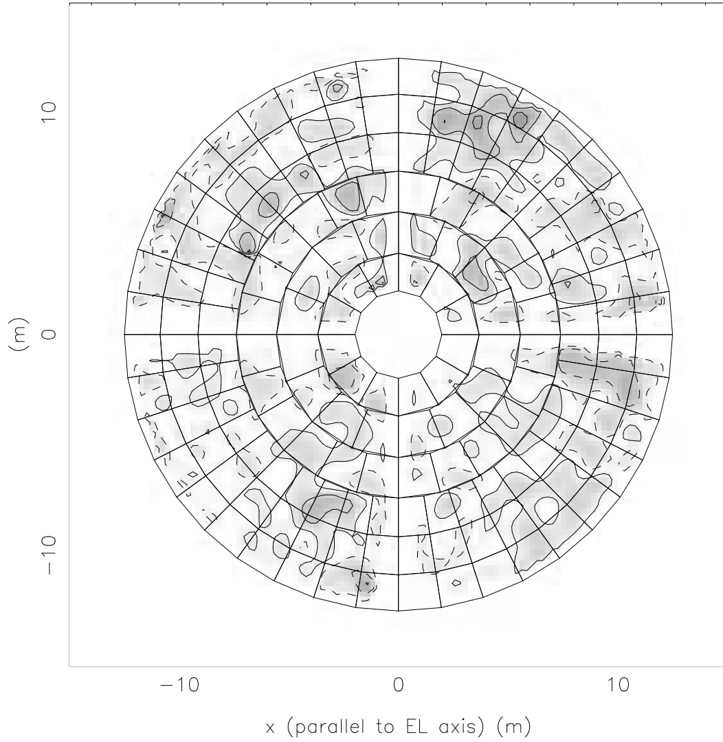
Figure 8: Antenna 8
