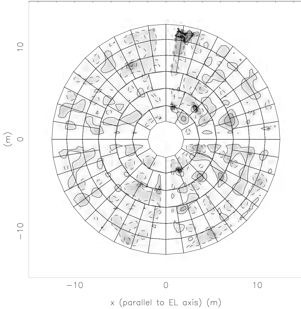
Figure 21: Antenna 21
