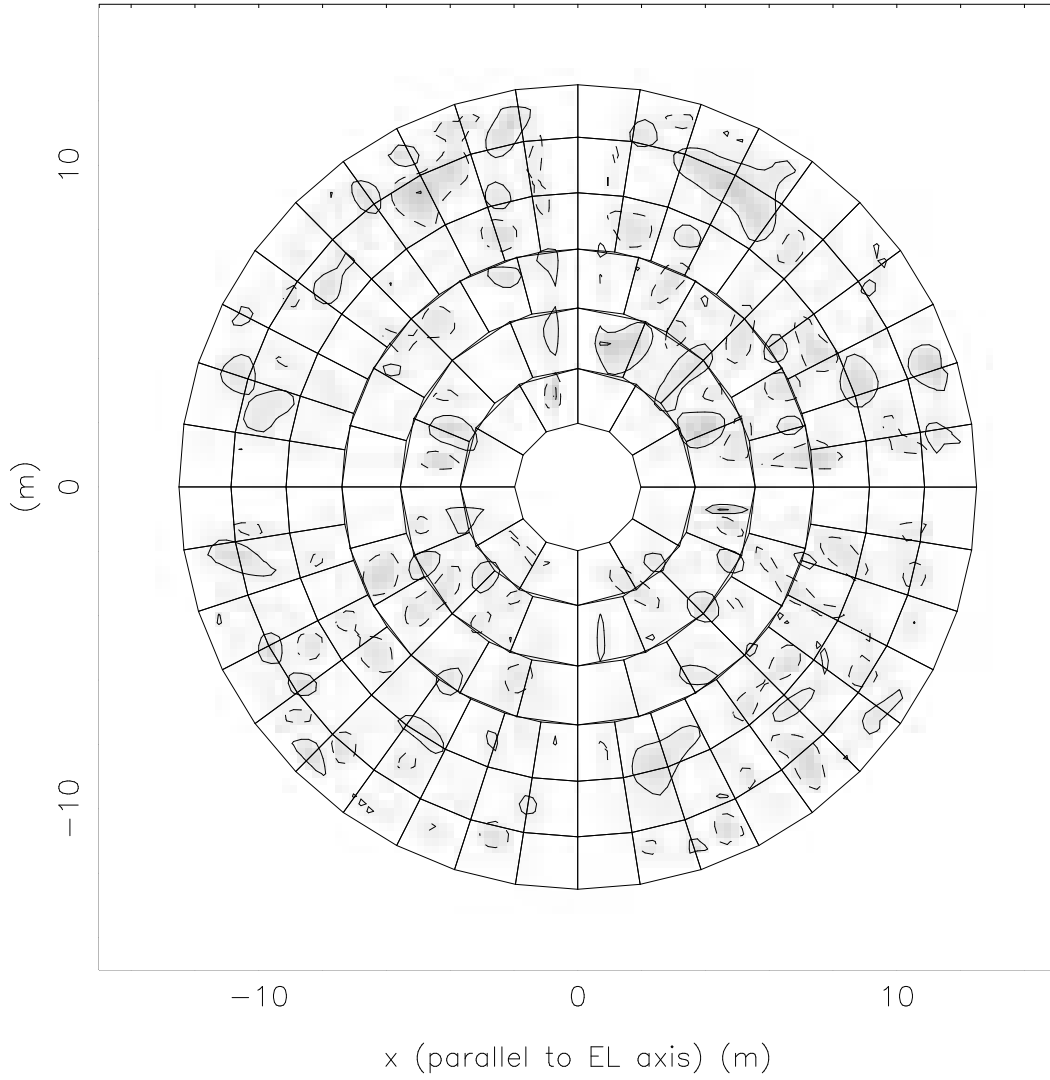
Figure 11: Antenna 11
