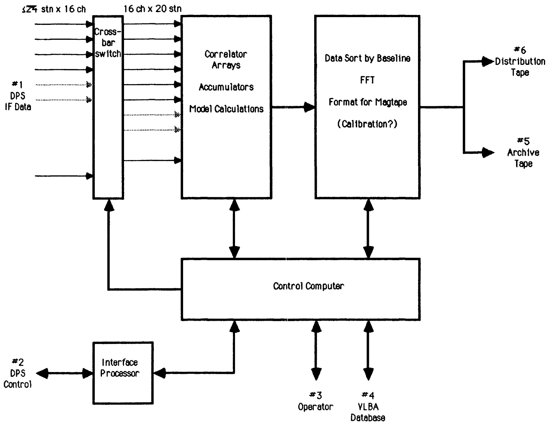
Level 1 VLBA Correlator Functional Block Diagram 3/7/85 MSE
