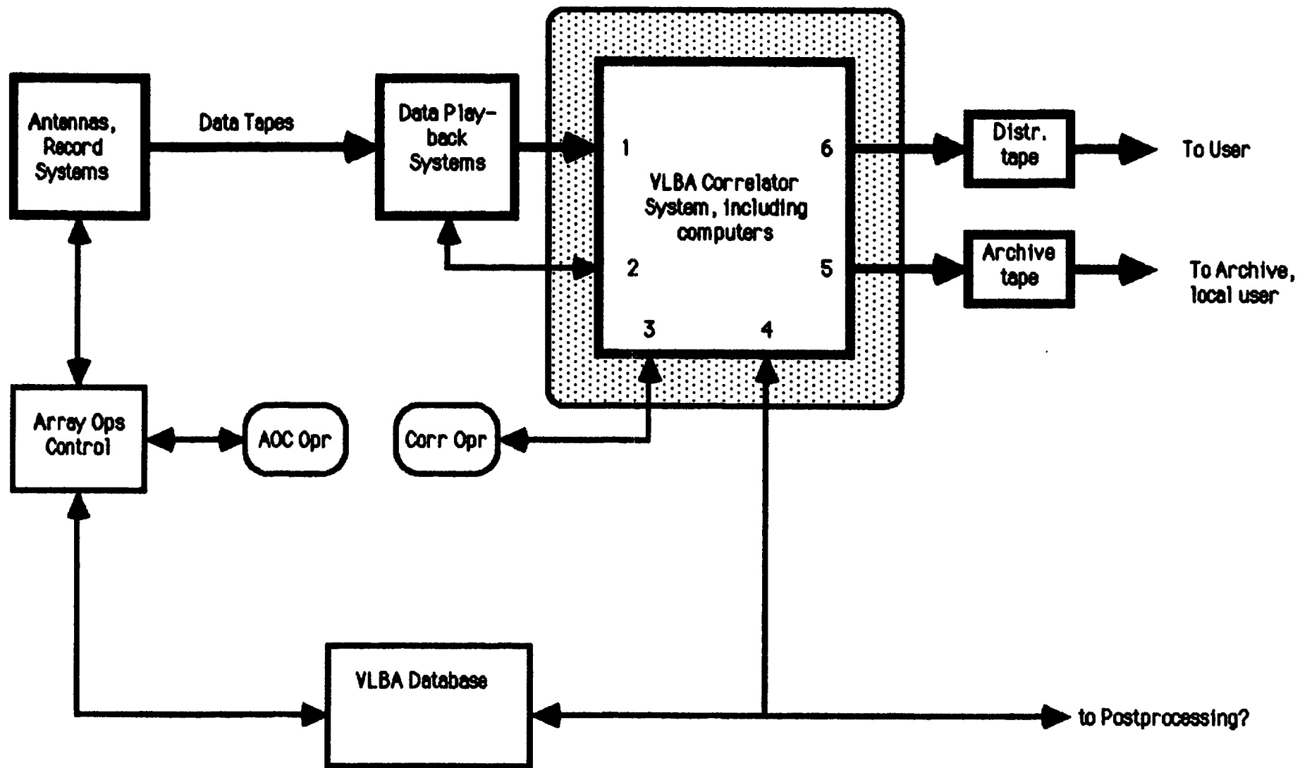
Level 0 VLBA Functional Block Diagram with Correlator Interfaces 3/7/85 MSE
