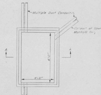
MULTIPLE DUCT CONDUIT MANHOLE PLAN VIEW SCALE: 1" = 2'
