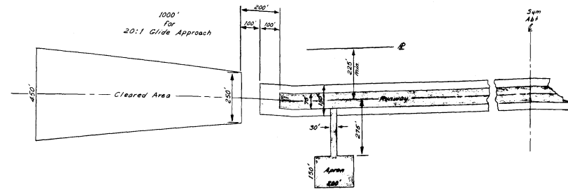
AIRSTRIP PLAN TYPICAL SCALE: 1" = 200'
