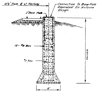
OBSERVATION STATION FOUNDATION TYPICAL SECTION (NOT TO SCALE)
