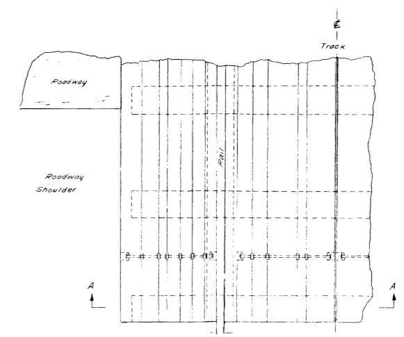
PREFABRICATED SECTIONAL TREATED TIMBER RAILWAY CROSSING (NOT TO SCALE)
