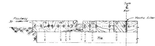
RAILWAY CROSSING SECTION A-A
