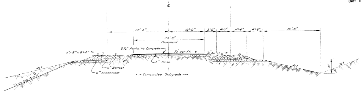
RAILWAY TYPICAL SECTION SCALE: 1" = 5' ALTERNATE I
