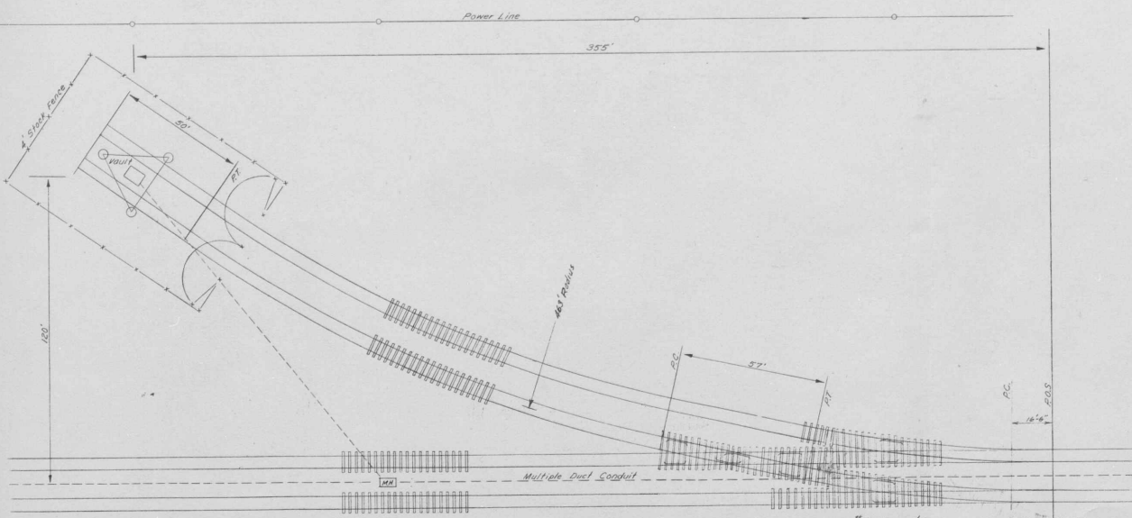
TYPICAL SPUR PLAN SCALE: 1" = 20'
