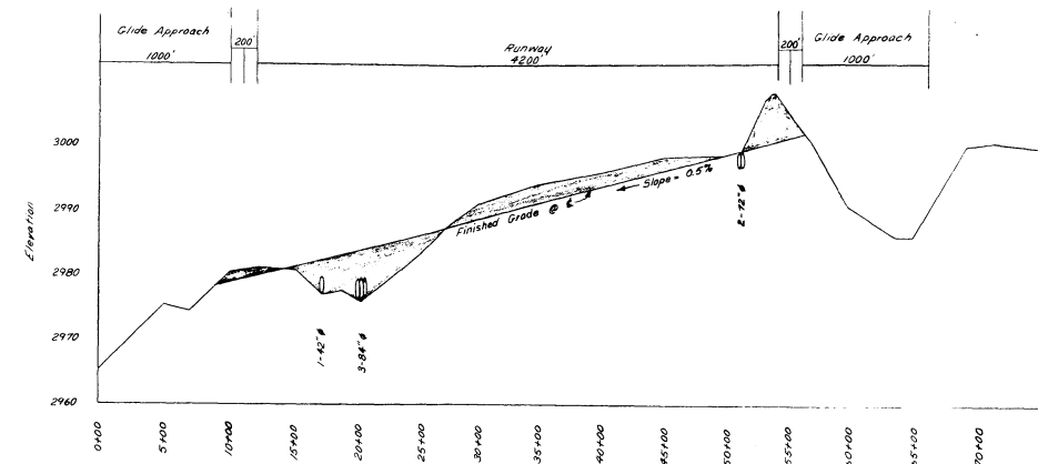
Y23 AIRSTRIP PROFILE
