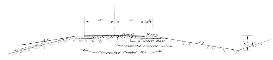
ACCESS ROAD TYPICAL SECTION (NOT TO SCALE)
