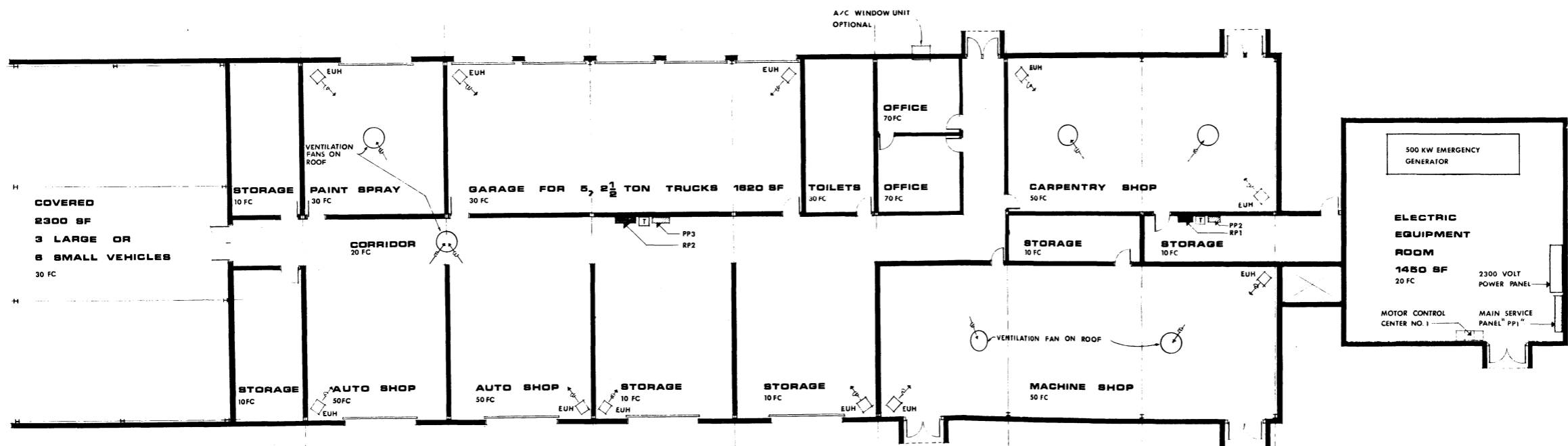
FLOOR PLAN 13670 SF
