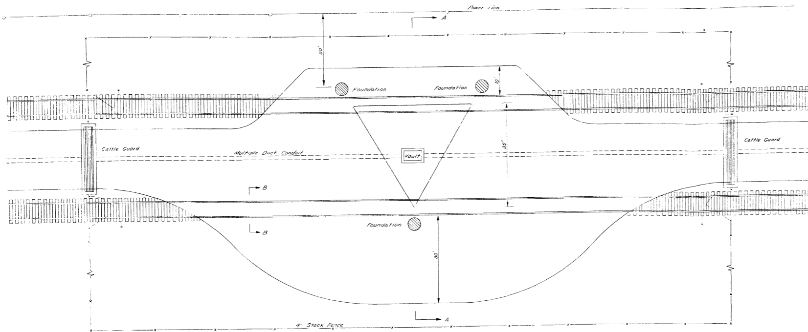
OBSERVATION STATION TYPICAL PLAN SCALE: 1" = 10' ALTERNATE I
