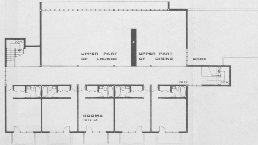
UPPER FLOOR PLAN 2800 SF
