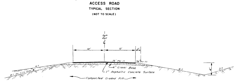
ENTRANCE ROAD TYPICAL SECTION (NOT TO SCALE)
