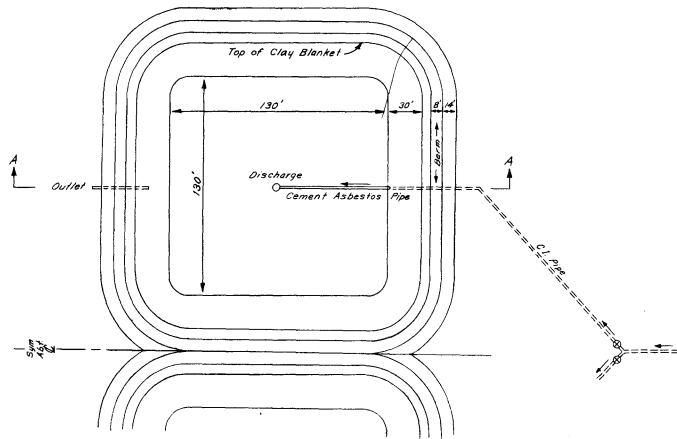
SEWAGE LAGOONS PLAN (NOT TO SCALE)
