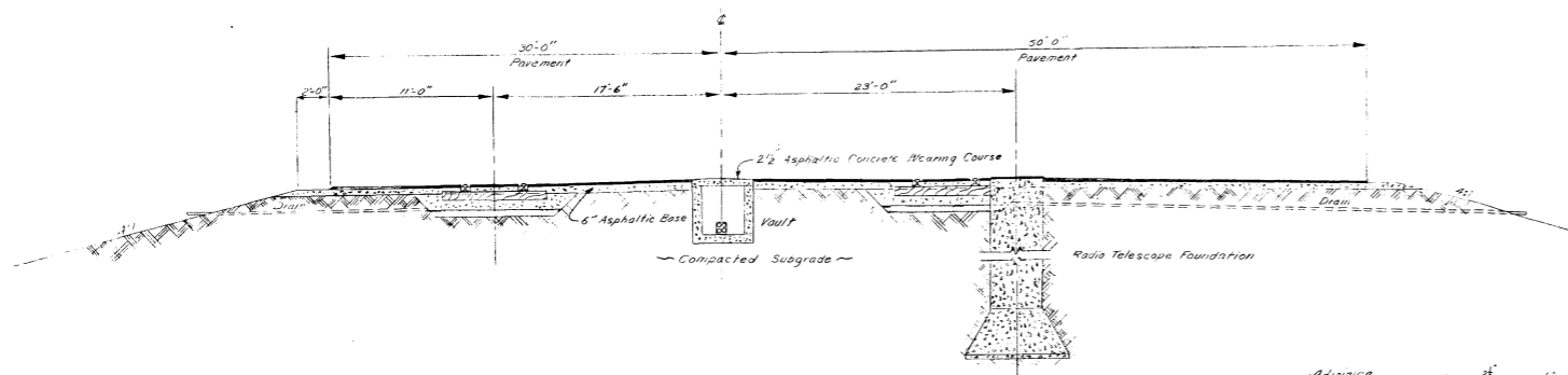
OBSERVATION STATION SECTION A-A SCALE: 1" = 5' ALTERNATE I
