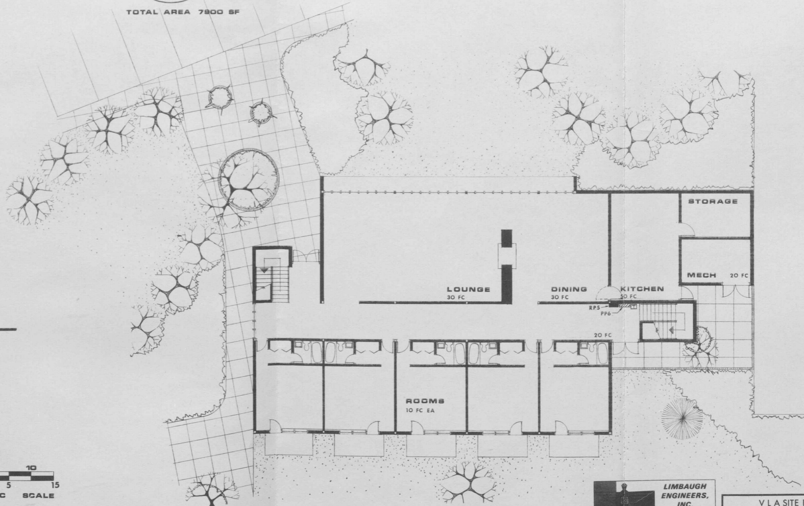
GROUND FLOOR PLAN 5100 SF
