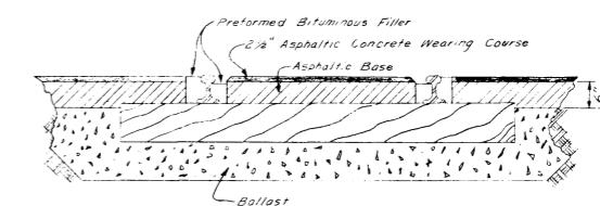
OBSERVATION STATION SECTION B-B (NOT TO SCALE) ALTERNATE I
