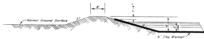
LAGOON BERM TYPICAL SECTION (NOT TO SCALE)
