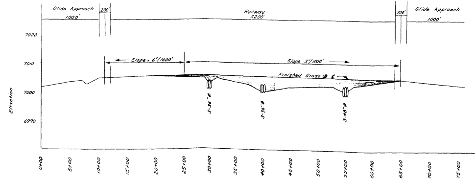
Y15 AIRSTRIP PROFILE
