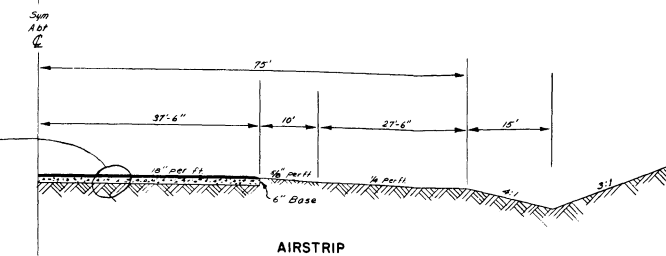
AIRSTRIP TYPICAL SECTION SCALE: 1" = 10'
