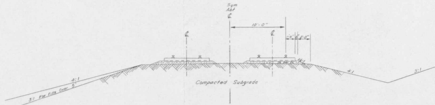
RAILWAY TYPICAL SECTION SCALE: 1" = 5'
