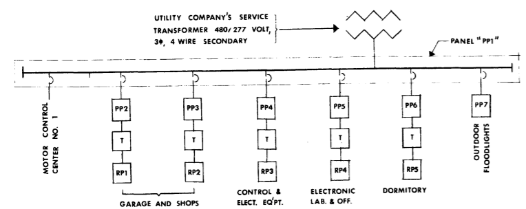
ELECTRIC DIAGRAM
