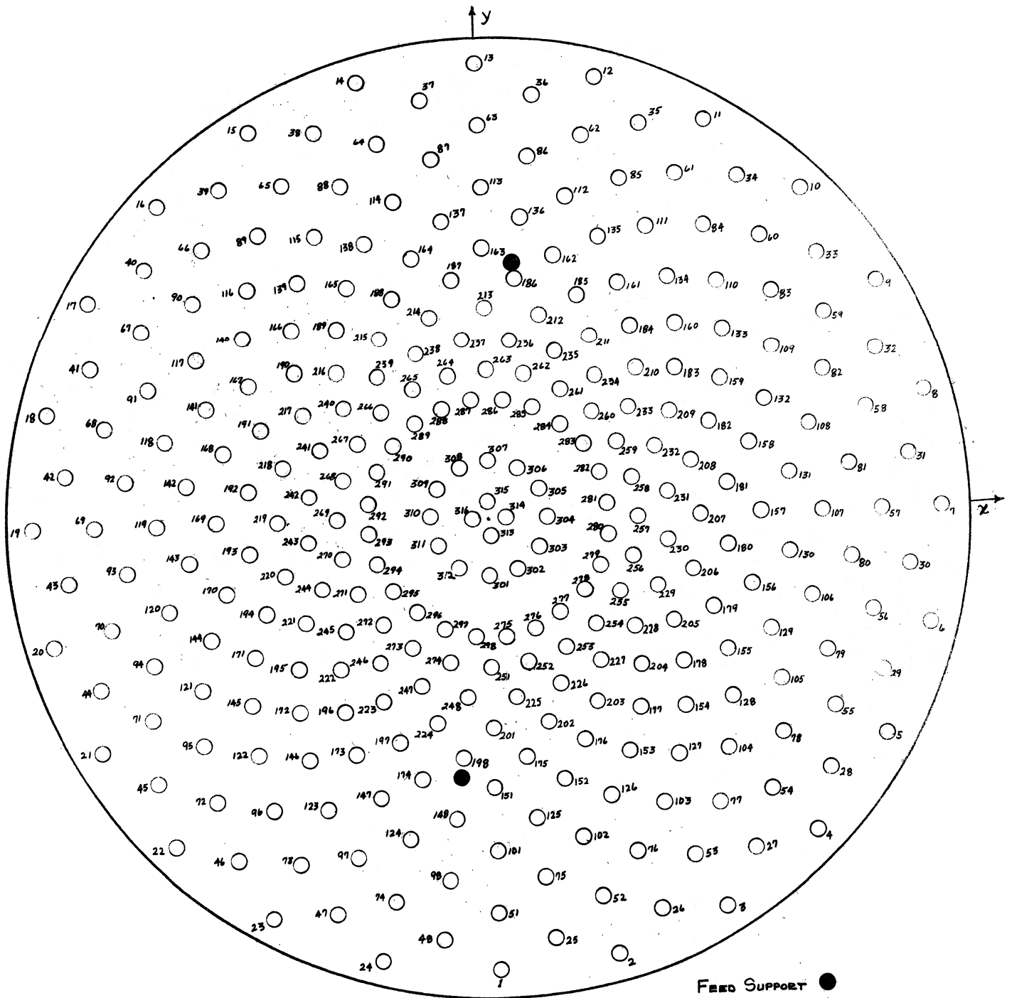
FIGURE 4. POSITION AND IDENTIFICATION OF TARGET POINTS
