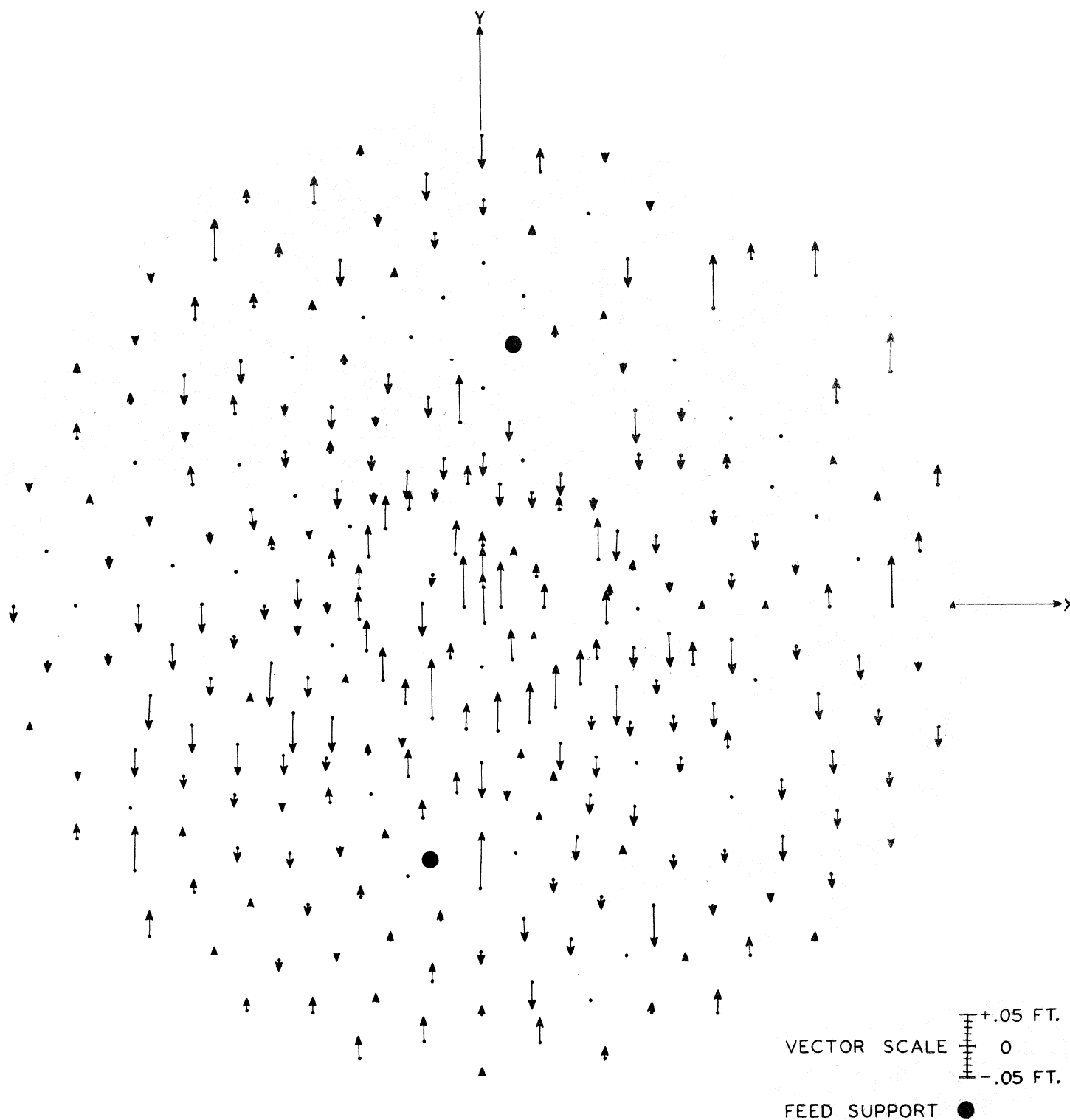
FIGURE 5. Plot of Perpendicular Departures of Photogrammetrically Triangulated Target Points from Best Fitting Paraboloid of Revolution. Positive Departures indicated by Upward Arrows, Negative Departures by Downward Arrows.
