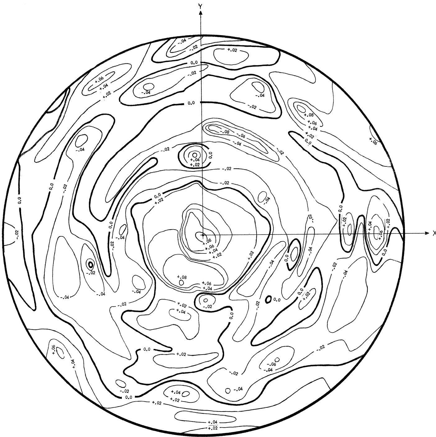
FIGURE 6. Contours of Error Surface of 300-Foot Antenna (0.02 ft. Contour Intervals)
