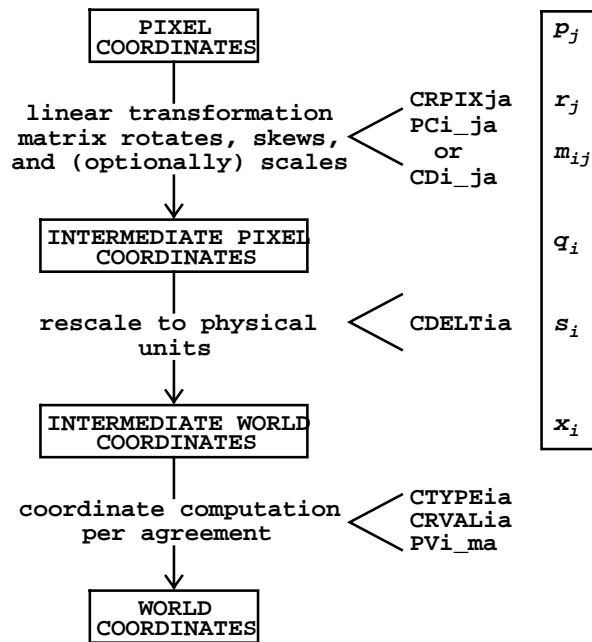
Figure 1: Schematic process for computing world coordinates from pixel coordinates.
