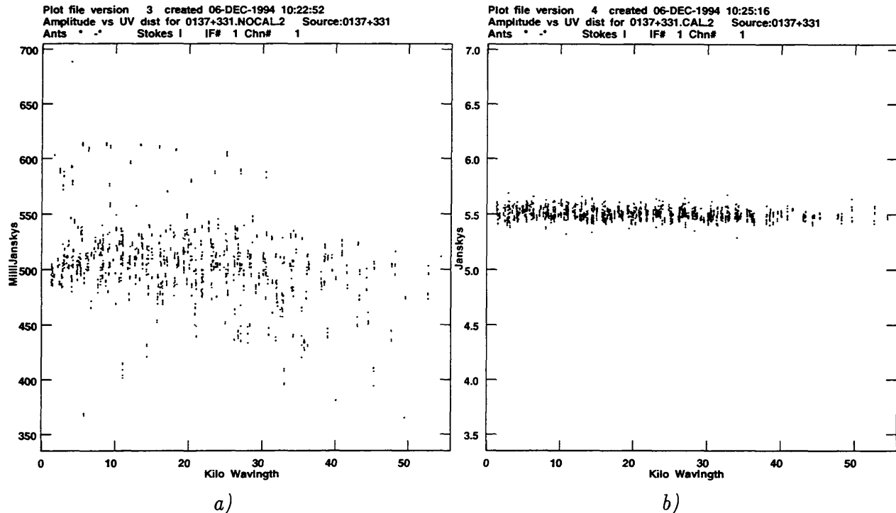
Figure: a) Un-calibrated uv -data and b) calibrated uv -data from a C-band snapshot of 3C48. Default VLA gains are a tenth of the actual gains and can show significant scatter. Only wild uv points \sim 50\% greater than the average can be detected before calibration.
