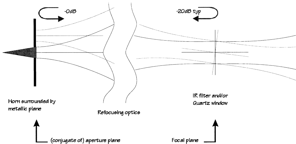
Figure 1. Explanatory sketch for sidelobe formation. See text.
