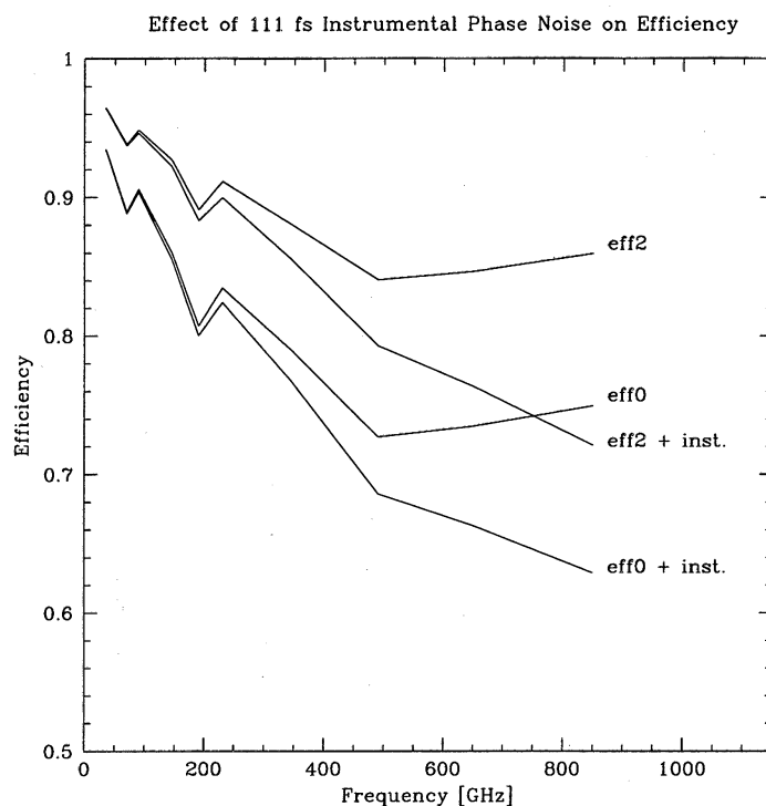
Figure 7: The affect of 111 fs instrumental delay jitter on the efficiency due to decorrelation only (eff2) and the total efficiency (eff0). The values of eff2 and eff0 are taken straight from Tables 3-5 and show the effect of the residual atmosphere and the inefficiencies of the calibration process, but no instrumental delay errors. The curves labeled “+ inst” indicate how the efficiencies are degraded when adding the 111 fs delay jitter.
