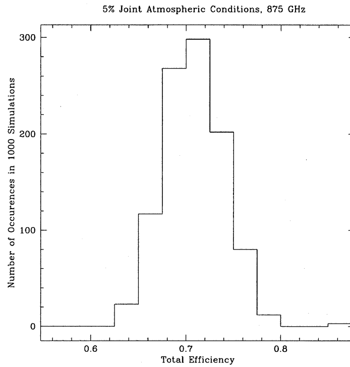
Figure 6: Histogram of the overall efficiency for the simulations reported on in Table 6 at 875 GHz.
