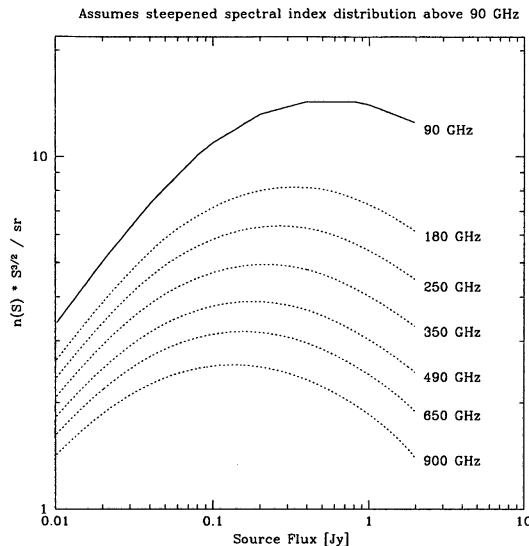
Figure 4: These are the integral source counts of flat spectrum quasars at various ALMA frequencies. The counts at 90 GHz will be fairly accurate, but we are guessing at the spectral index distribution for higher frequencies: to estimate the higher frequency source counts, we are taking the measured 8-90 GHz spectral index distribution and steepening it by 0.5, resulting in a median spectral index of 0.8 above 90 GHz.
