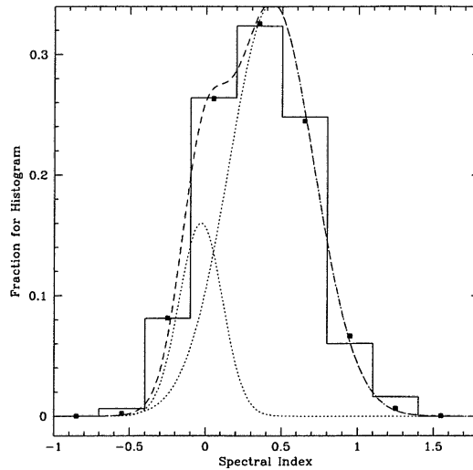
Figure 3: The seven bin histogram is the spectral index ( S(\nu) \propto \nu^{-\alpha} ) distribution from 8 GHz to 90 GHz for the 367 flat spectrum quasars observed by Holdaway, Owen, and Rupen (1994). See the text if you want to know about the Gaussians and filled squares.
