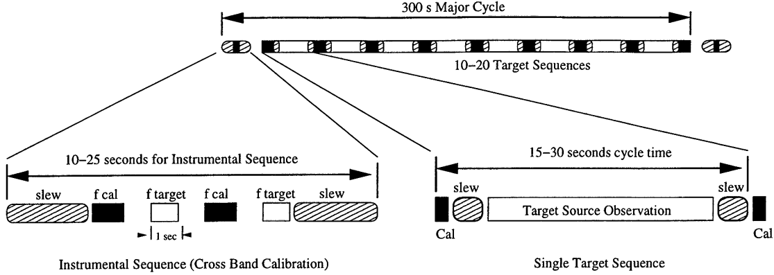
Figure 1: Overview of fast switching, showing both the target sequence and the instrumental sequence. The calibrator for the target sequence will typically be within 2 deg of the target source, while the calibrator used in the instrumental sequence will be up to 15 deg away from the target source.
