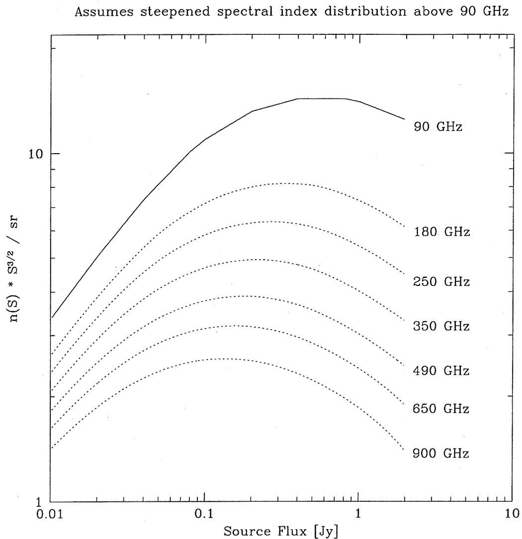
Figure 1: Quasar source count estimates for 90 GHz from Holdaway, Owen, and Rupen (1994), and extrapolations to higher frequencies, assuming a spectral steepening of +0.5 above 90 GHz.
