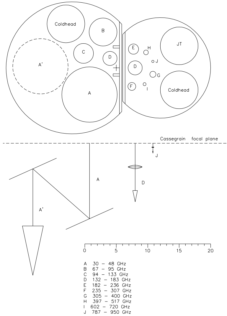
Figure 1: (top) A possible scheme for placing receivers for 10 frequency bands in 2 dewars: a 12 K dewar for low frequency (30 to 133 GHz) HEMT front ends and a 4 K dewar for SIS (133 to 950 GHz) front ends. (bottom) The optical paths for the 30 - 48 GHz, 132 - 183 GHz, and 787 - 950 GHz bands are shown from the Cassegrain focal plane to the horns. The lowest frequency band uses a pair of mirrors to re-image the telescope aperture at the horn aperture; the higher frequency bands are shown with re-imaging lenses which can also serve as radiation shields.
