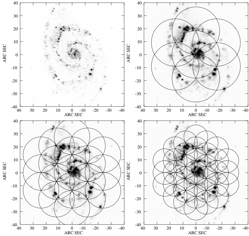
Figure 2: Model image and the mosaic footprints. A greyscale image of the raw model image is shown on top left. The mosaic footprint for the 6m (top right), 8m (bottom left), and 12m (bottom right) array are shown over the greyscale image of the model image convolved to 1'' resolution.
