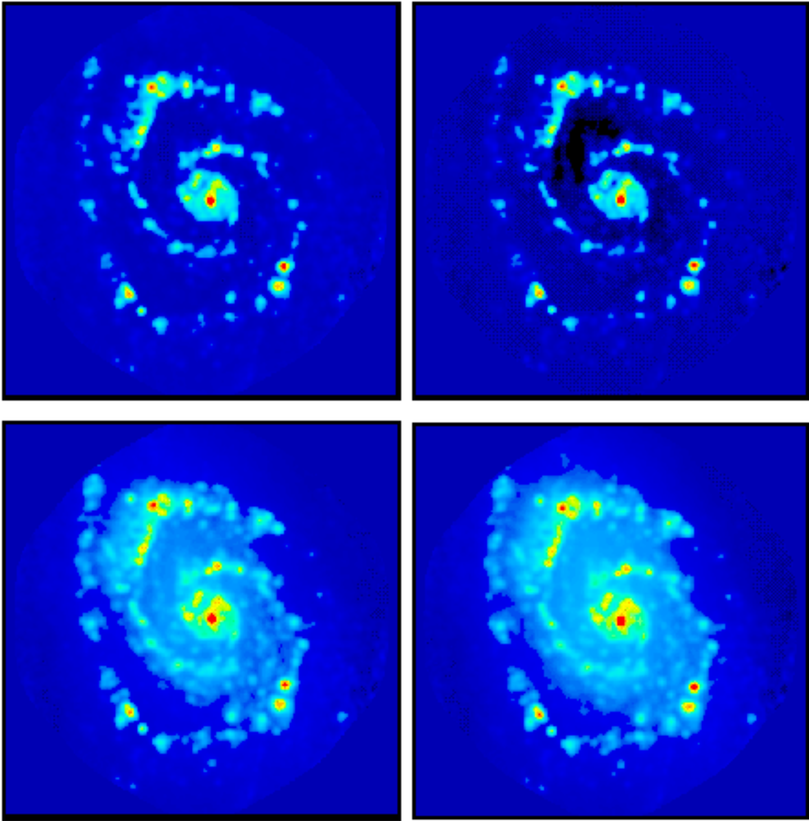
Figure 9: Simulated observations with a combined 13 x 8m ACA and 64 x 12m array. See Figure 3 caption for the description of each panels. The range of amplitude plotted is identical to Figure 7.
