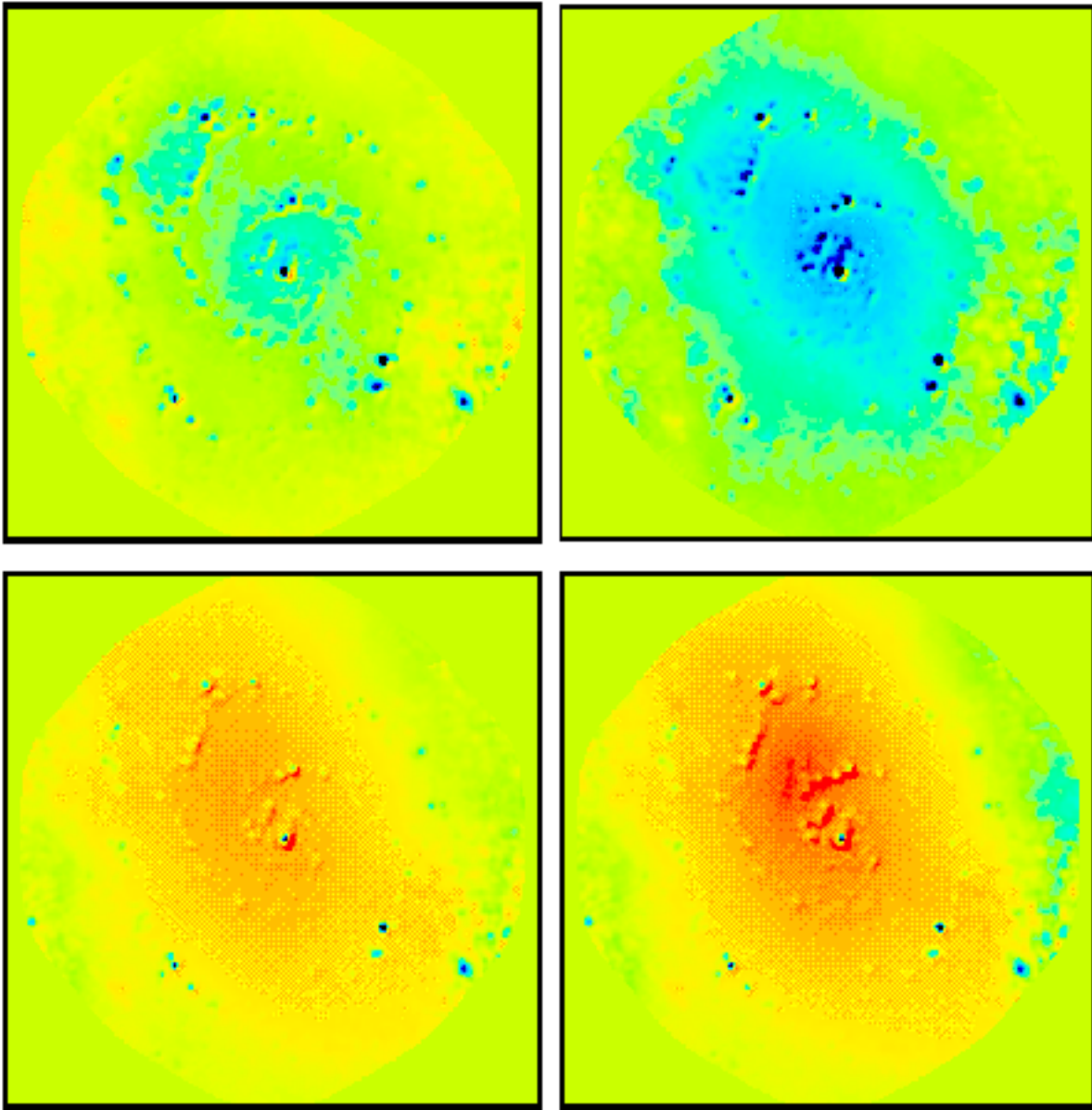
Figure 8: Difference images between the simulated observations using a combined 19 x 6m ACA and 64 x 12m array and the input model image convolved to the match resolution ( 1'' ). See Figure 4 caption for the description of each panels. The range of amplitude plotted are from -30 (black) to +30 (red).
