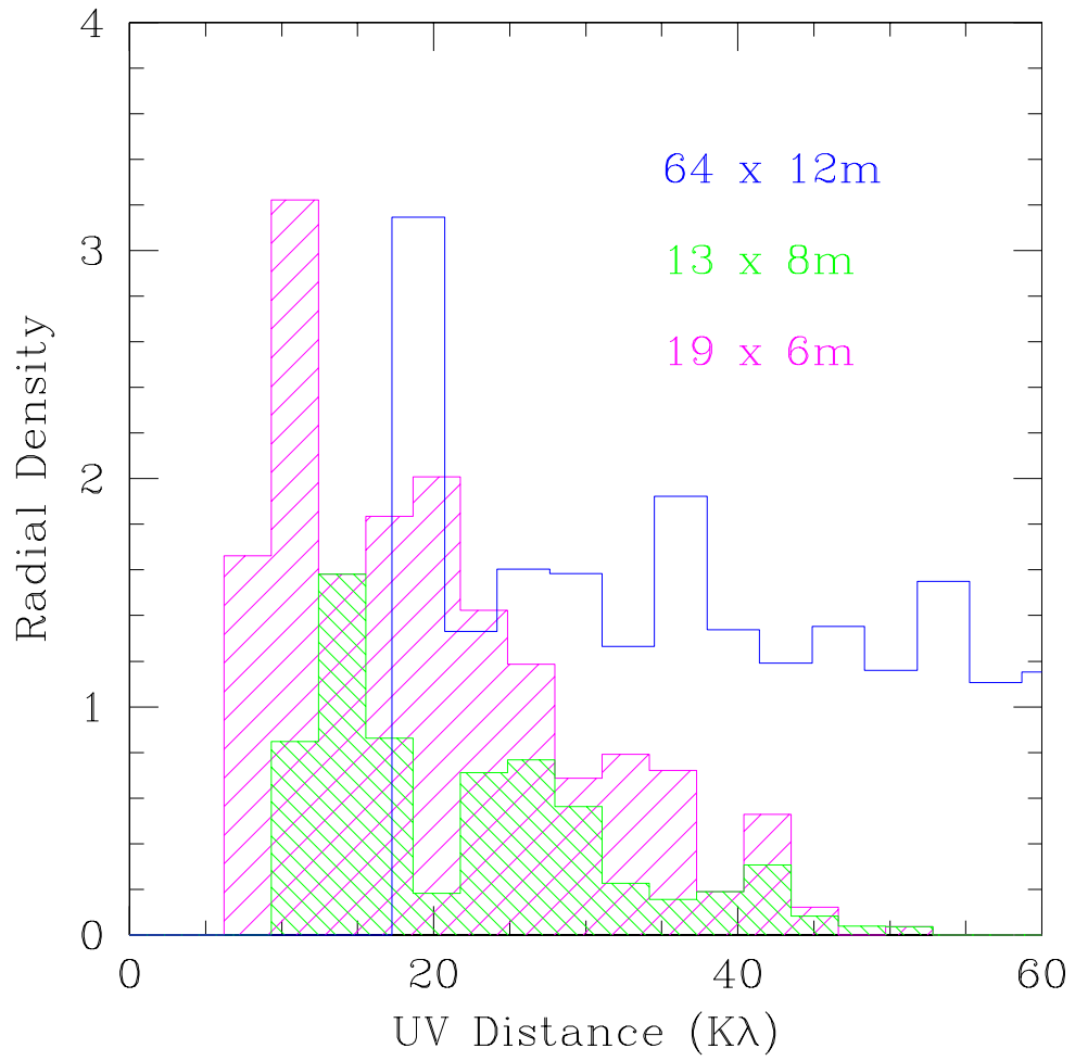
Figure 12: Plot of radial density distribution for the 6m, 8m, and 12m arrays. 10 k\lambda corresponds to about 8m at 345 GHz.
