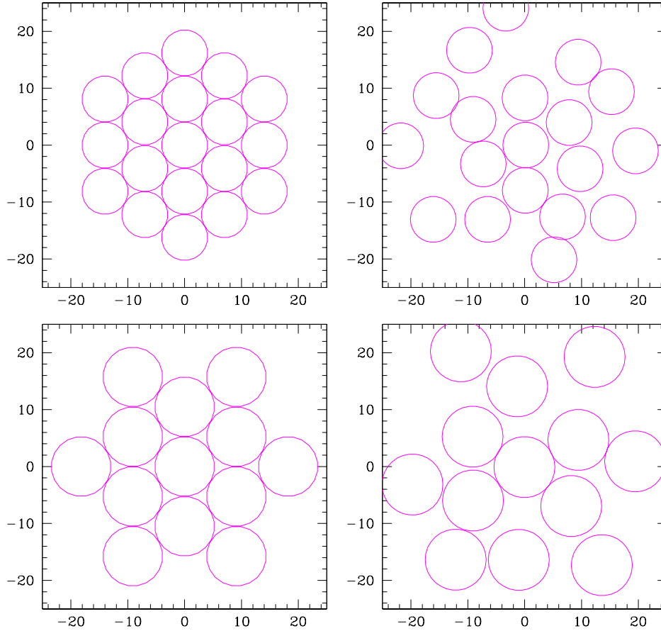
Figure 1: The ACA design layouts. The 19 \times 6m array is shown on top, and the 13 \times 8m array is shown at the bottom. The fully packed design (left) is modified for better imaging performance using the Kogan (1998) minimum sidelobe algorithm (right). Each circle represents 1.3D of the antennas. Axis labels are in units of meters.
