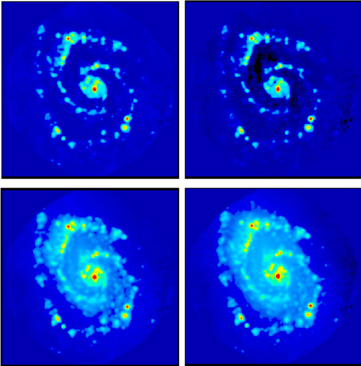
Figure 7: Simulated observations with a combined 19 x 6m ACA and 64 x 12m array. See Figure 3 caption for the description of each panels. The range of amplitude plotted are from -50 (black) to +350 (red).
