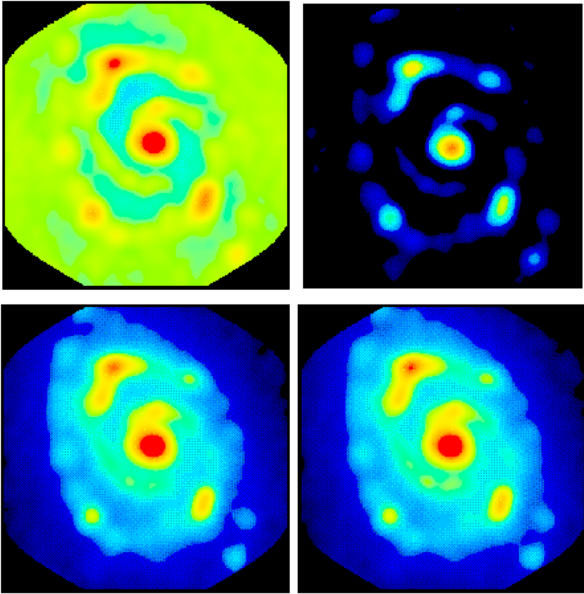
Figure 5: Simulated observations with a 13 x 8m Array alone. See Figure 3 caption for the description of each panels. The range of amplitude plotted is also identical to Figure 3.
