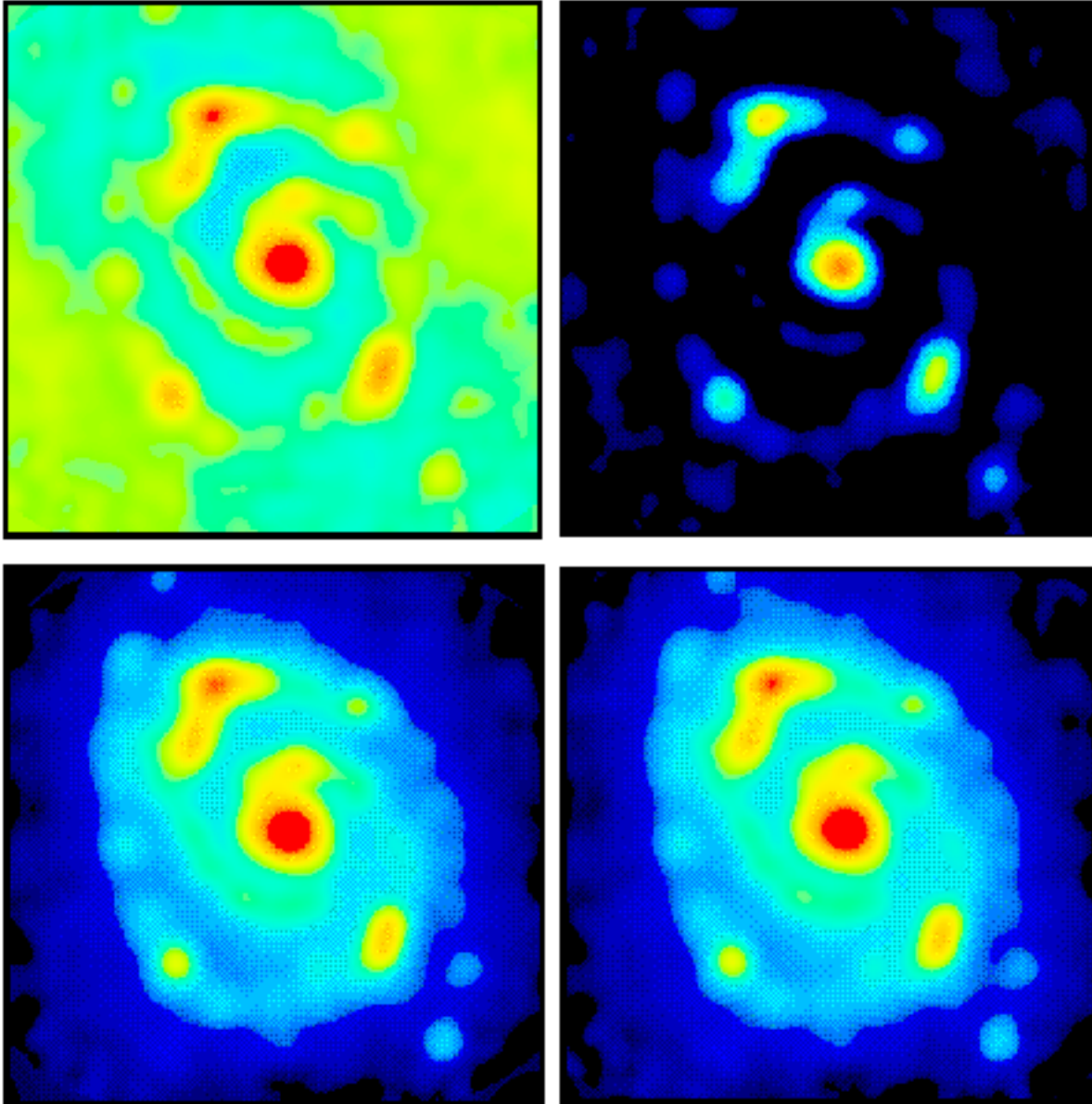
Figure 3: Simulated observations with a 19 x 6m Array alone. The top row of images are produced using only the cross-correlation data only while the bottom row images include the total power data as well. The left panel images are produced using AIPS task VTESS (“maximum entropy”) while the right panel images are produced using AIPS task UTESS (“maximum emptiness”). The range of amplitude plotted are from 0 (black) to +1500 (red).
