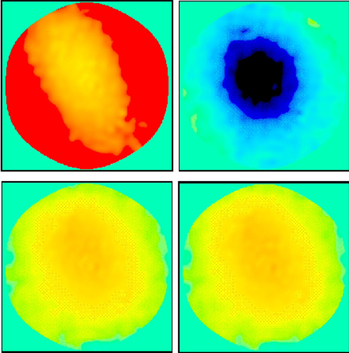
Figure 4: Difference images between the simulated observations using a 19 x 6m Array alone and the input model image convolved to the matching resolution ( 4'' ). The four panels correspond exactly to the images shown in Figure 3. The range of amplitude plotted are from -300 (black) to +500 (red).
