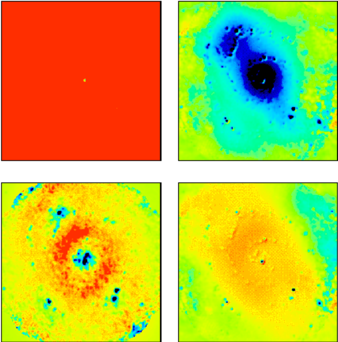
Figure 14: Difference images between the simulated observations using a 64 x 12m Array alone and the input model image convolved to the match resolution ( 1'' ). See Figure 4 caption for the description of each panels. The range of amplitude plotted is identical to Figure 8.
