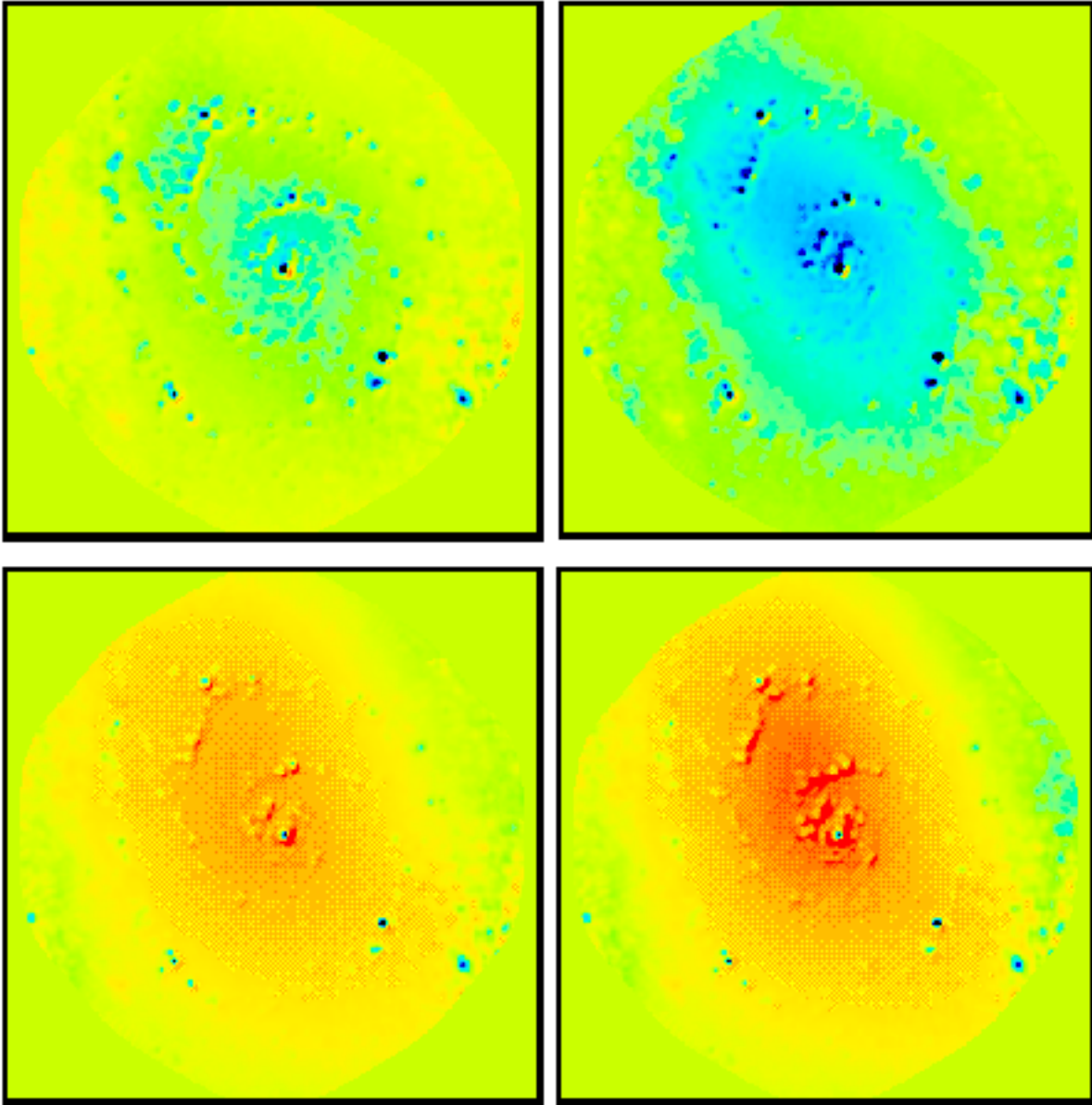
Figure 10: Difference images between the simulated observations using a combined 13 x 8m ACA and 64 x 12m array and the input model image convolved to the match resolution ( 1'' ). See Figure 4 caption for the description of each panels. The range of amplitude plotted is identical to Figure 8.
