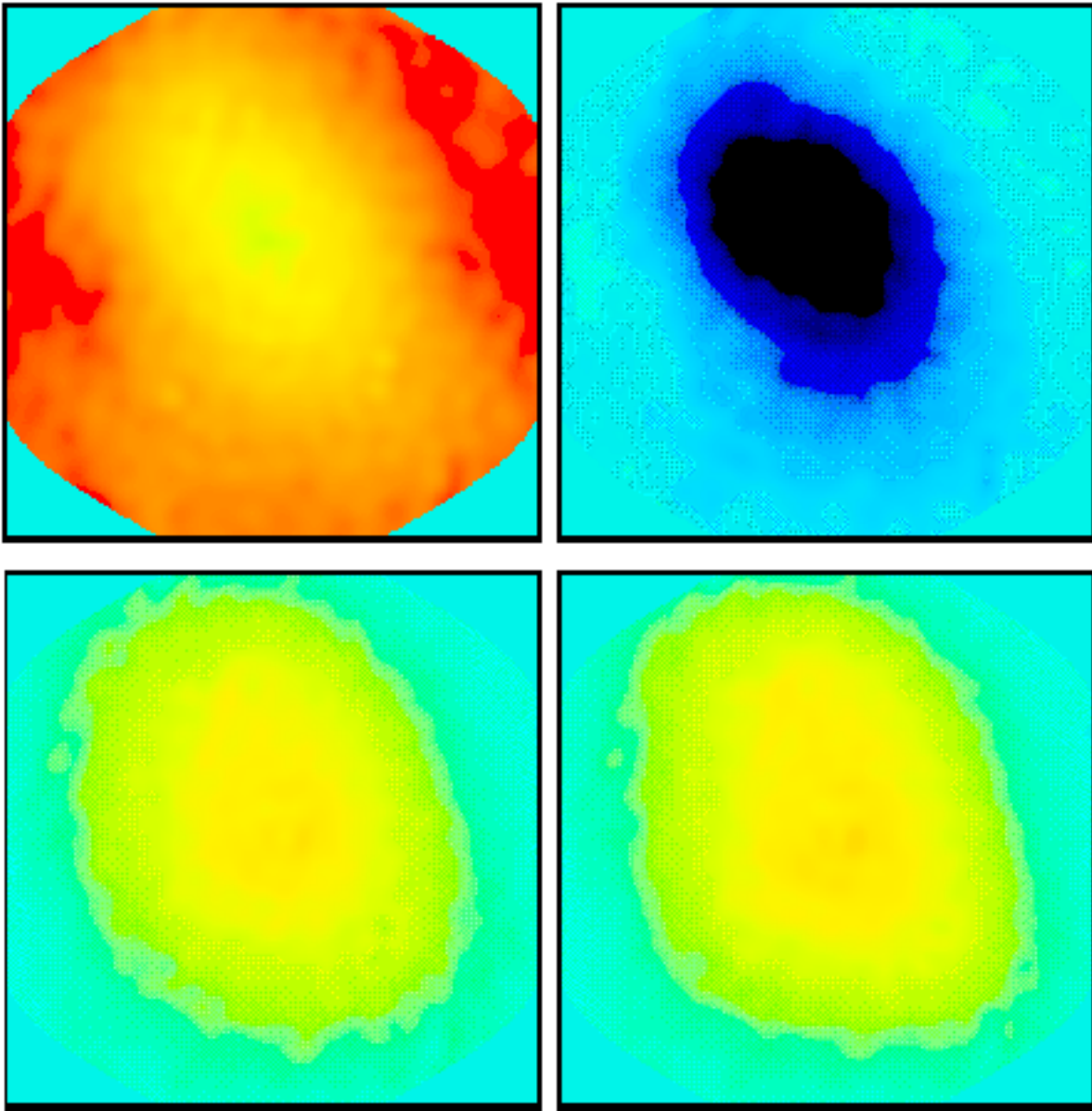
Figure 6: Difference images between the simulated observations using a 13 x 8m Array alone and the input model image convolved to the match resolution ( 4'' ). See Figure 3 caption for the description of each panels. The range of amplitude plotted is also identical to Figure 4.
