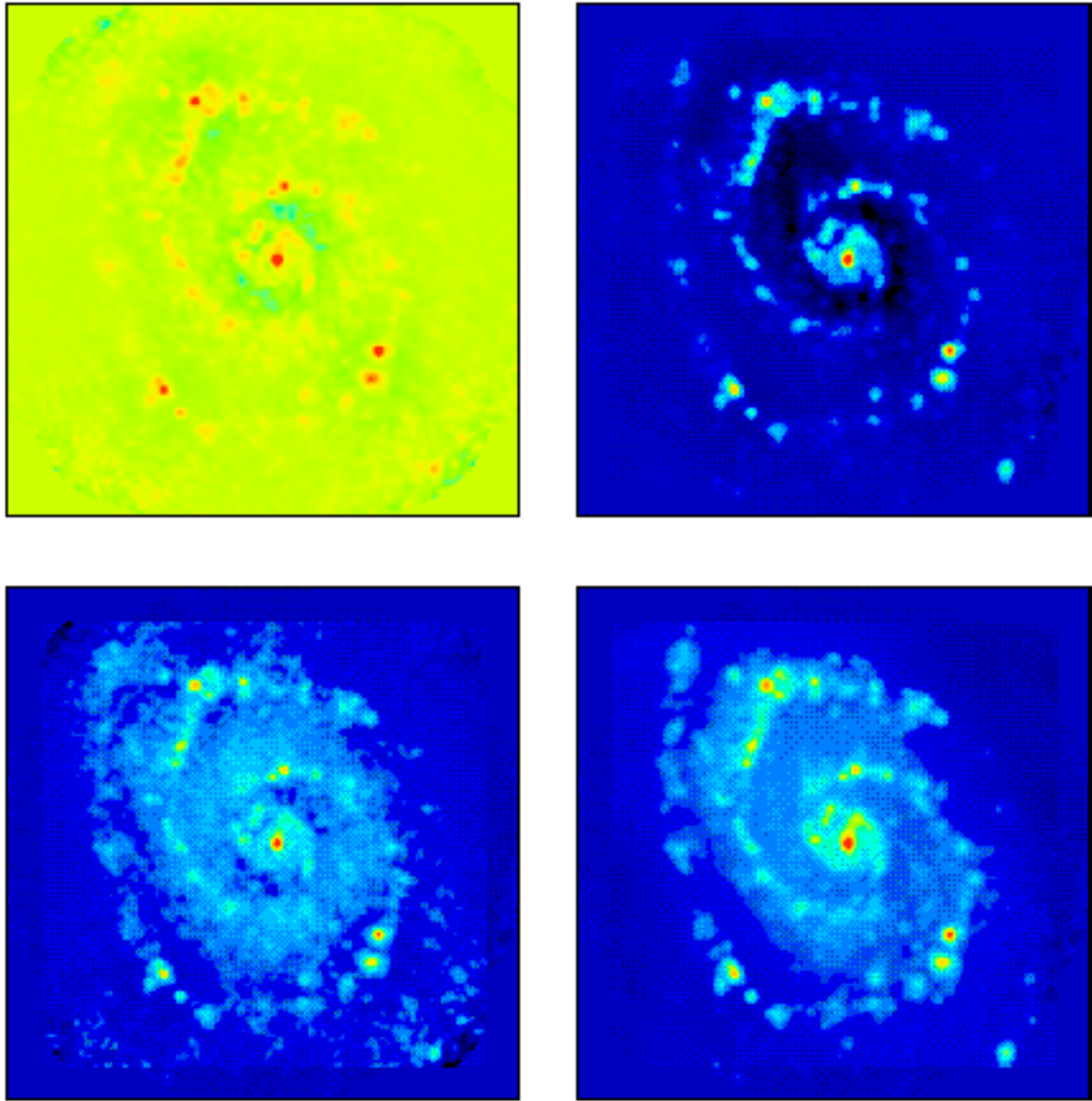
Figure 13: Simulated observations with a 64 x 12m Array alone. See Figure 3 caption for the description of each panels. The range of amplitude plotted is identical to Figure 7.
