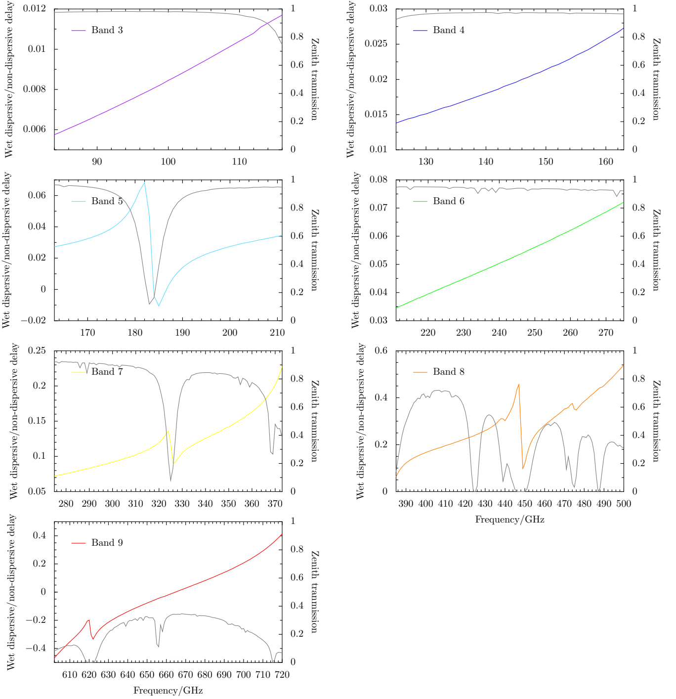
Figure 2. Ratio of the wet dispersive to wet non-dispersive delay for the construction ALMA observing bands, listed in Tab. 2 . Also plotted (grey) is the atmospheric zenith transmission at the same frequency. The ratio rises continually with frequency and becomes particularly significant in the submillimetre bands (Bands 7, 8 & 9).
