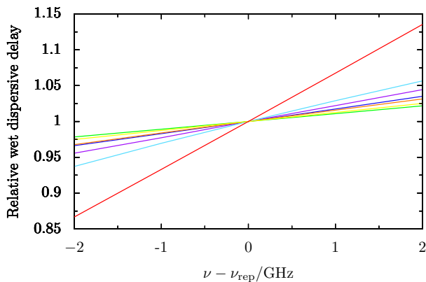
Figure 3. Variation in wet dispersive path delay for the construction ALMA bands, which were listed in Tab. 2. The lines use the same colours as Fig. 2 for the different bands: 3 (purple), 4 (dark blue), 5 (light blue), 6 (green), 7 (yellow), 8 (orange), 9 (red). The delays are plotted for frequencies in a 4-GHz portion around the bands’ representative frequencies (listed in Tab. 2, typically the band centres). This portion represents half of the instantaneous contiguous bandwidth (either the upper or lower sideband) for the ALMA 2SB mixers. Each measurement is divided by the value at the representative frequency and all the computations are for the median atmosphere specified in Tab. 1. The Band 9 receivers are DSB and therefore provide 8-GHz contiguous bandwidth (not plotted), which results in about a 30 per cent variation in the dispersive path delay towards the band edges compared with the representative frequency.
