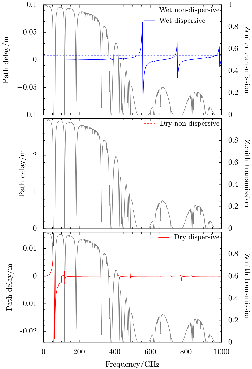
Figure 1. Wet non-dispersive ( top panel, dashed blue ) and dispersive ( top panel, solid blue ) path delays alongside the dry non-dispersive ( middle panel, dashed red ) and dispersive ( bottom panel, solid red ) path delays calculated by \Delta TM for the AOS model atmosphere with standard parameters as listed in Tab. 1 , including a 1.22 mm column of water. Overlaid in grey on all three panels is the corresponding zenith atmospheric transmission, calculated from the total opacity, \tau (as e^{-\tau} ).
