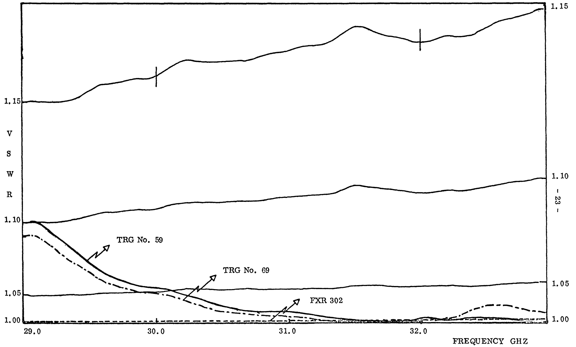
FIG. 13 - VSWR OF COMMERCIAL FIXED LOADS
