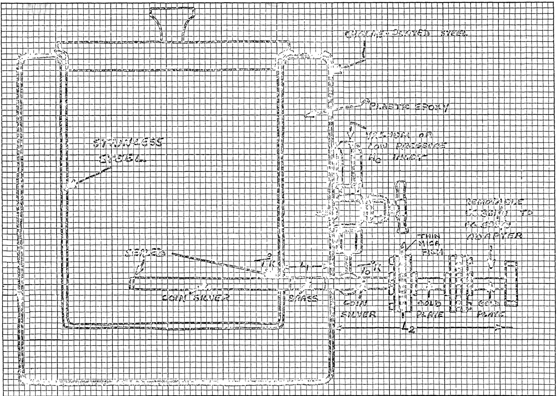
FIG. 4 - ADVANCED TECHNOLOGY, LIQUID NITROGEN LOAD (LN-96)
