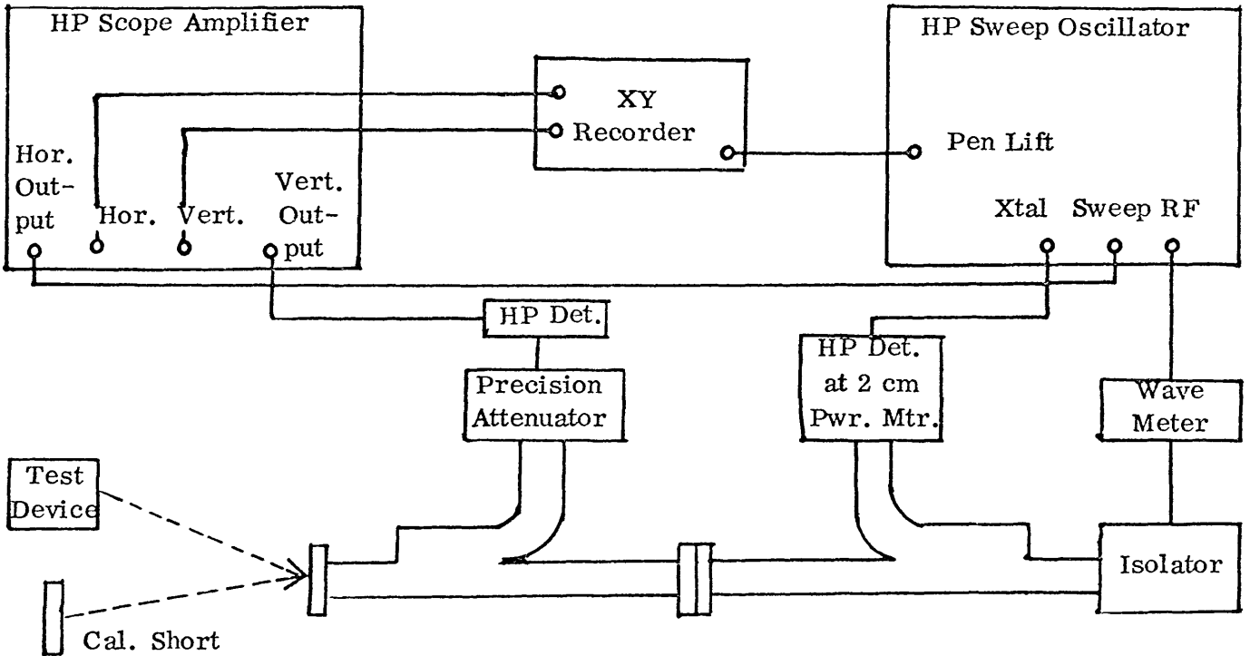
I. TEST SET UP FOR RETURN LOSS MEASUREMENTS
