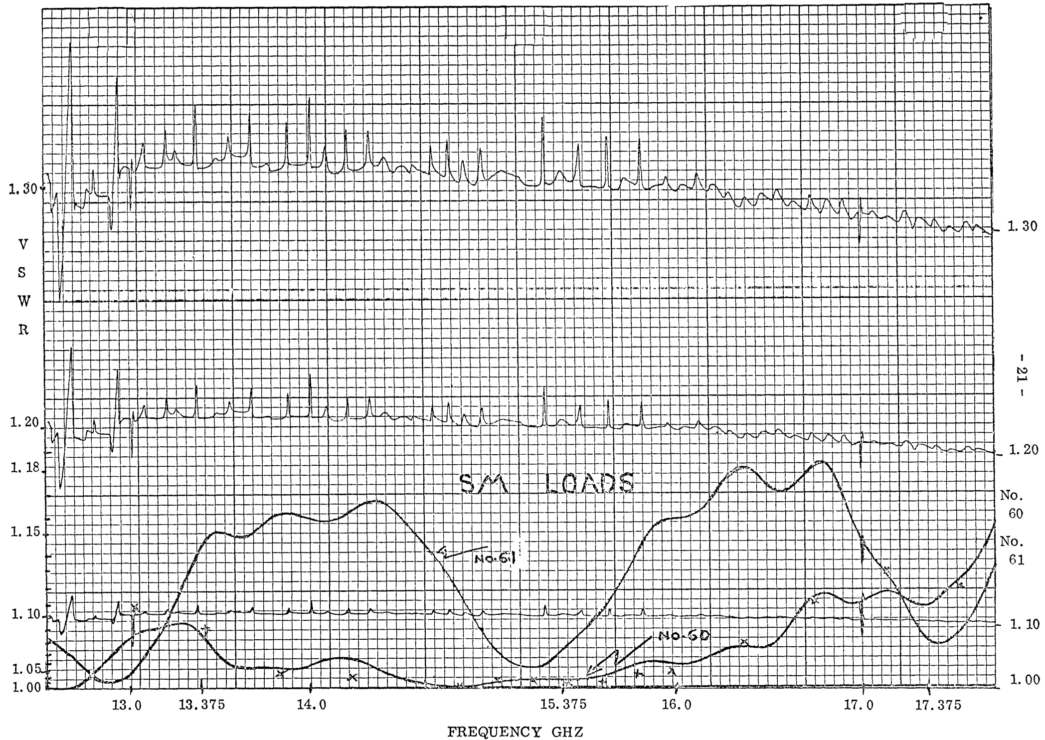
FIG. 11 - VSWR OF SM LOADS
