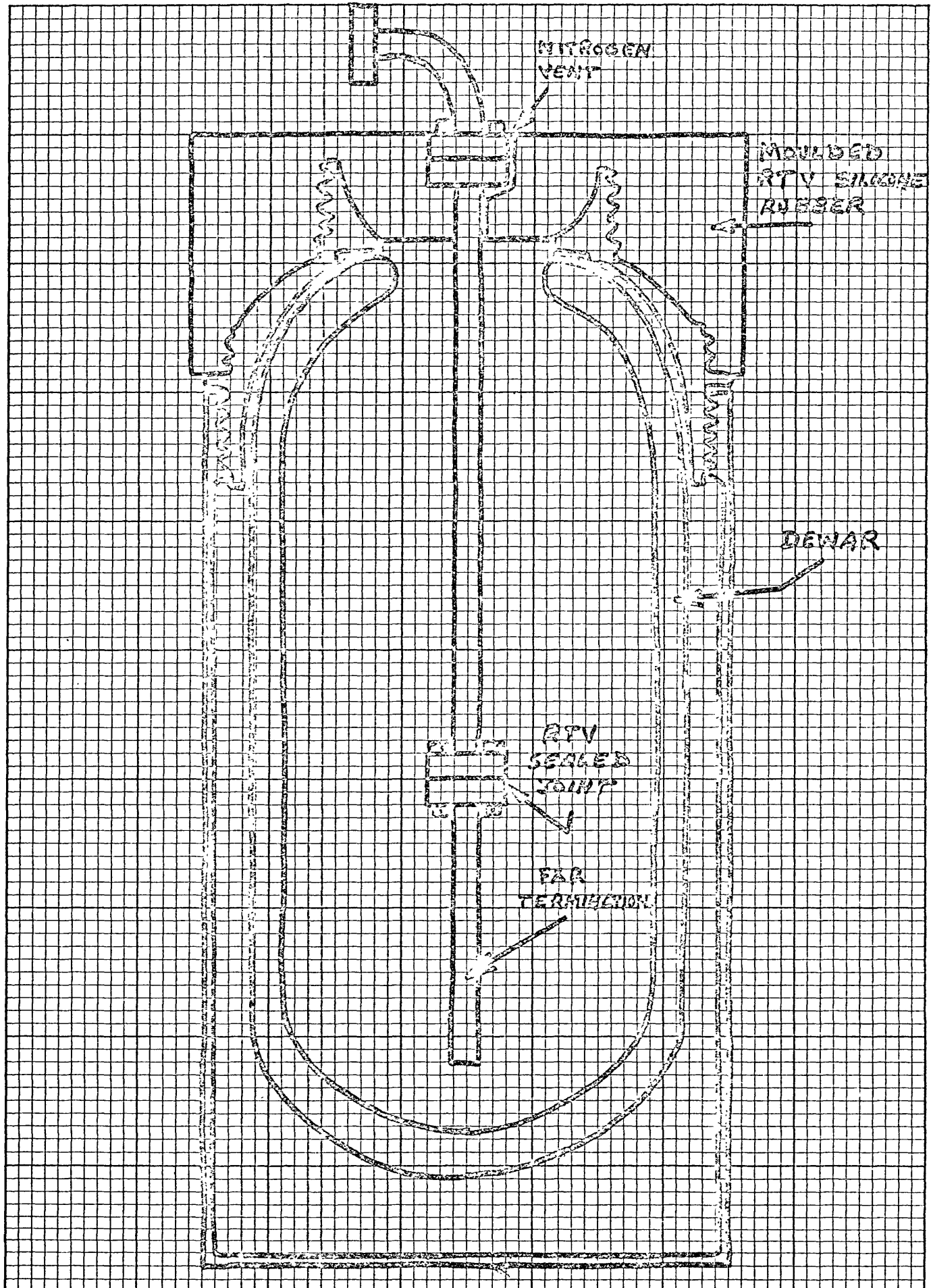
FIG. 3 - LABORATORY ASSEMBLED 9.5 mm LOAD
