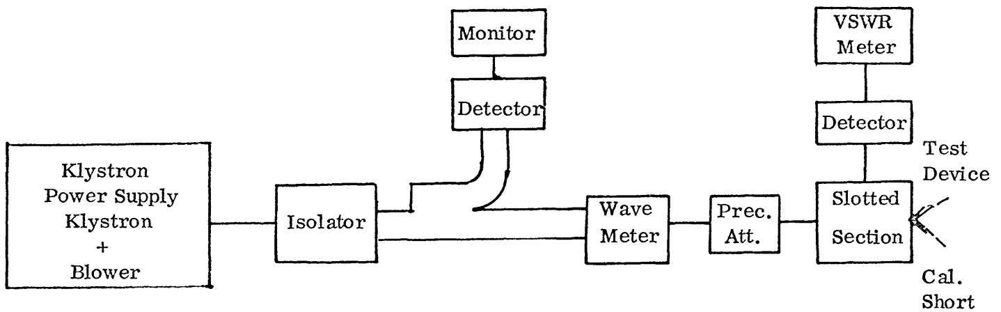
II. TEST SET UP FOR VSWR MEASUREMENTS
