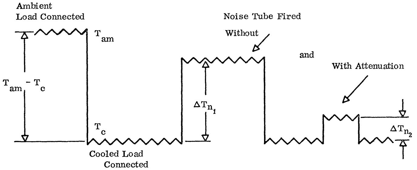
FIG. 2 - TYPICAL CALIBRATION CHART (NOT TO SCALE)
