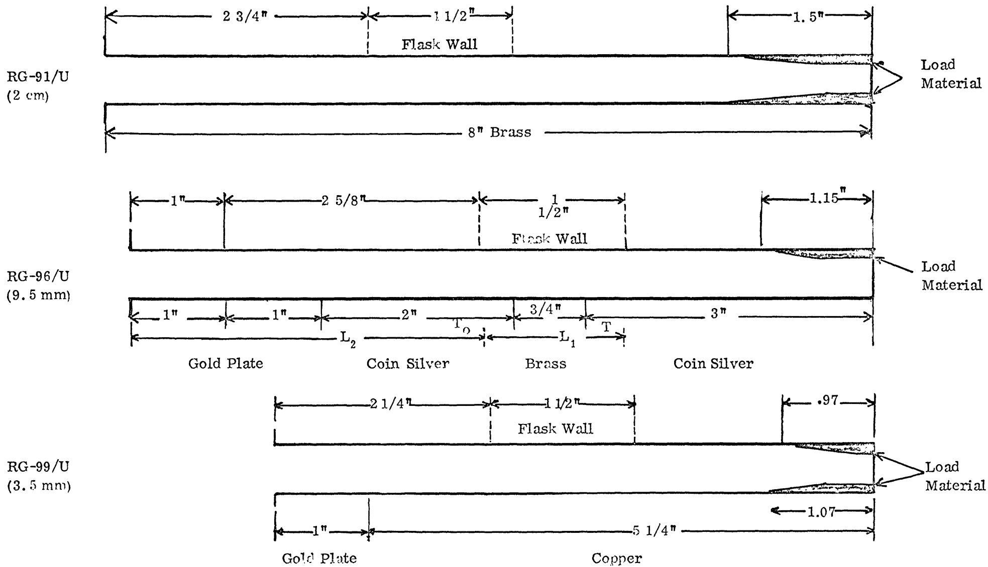
FIG. 8 - ADTECH LIQUID NITROGEN LOAD CONFIGURATION
