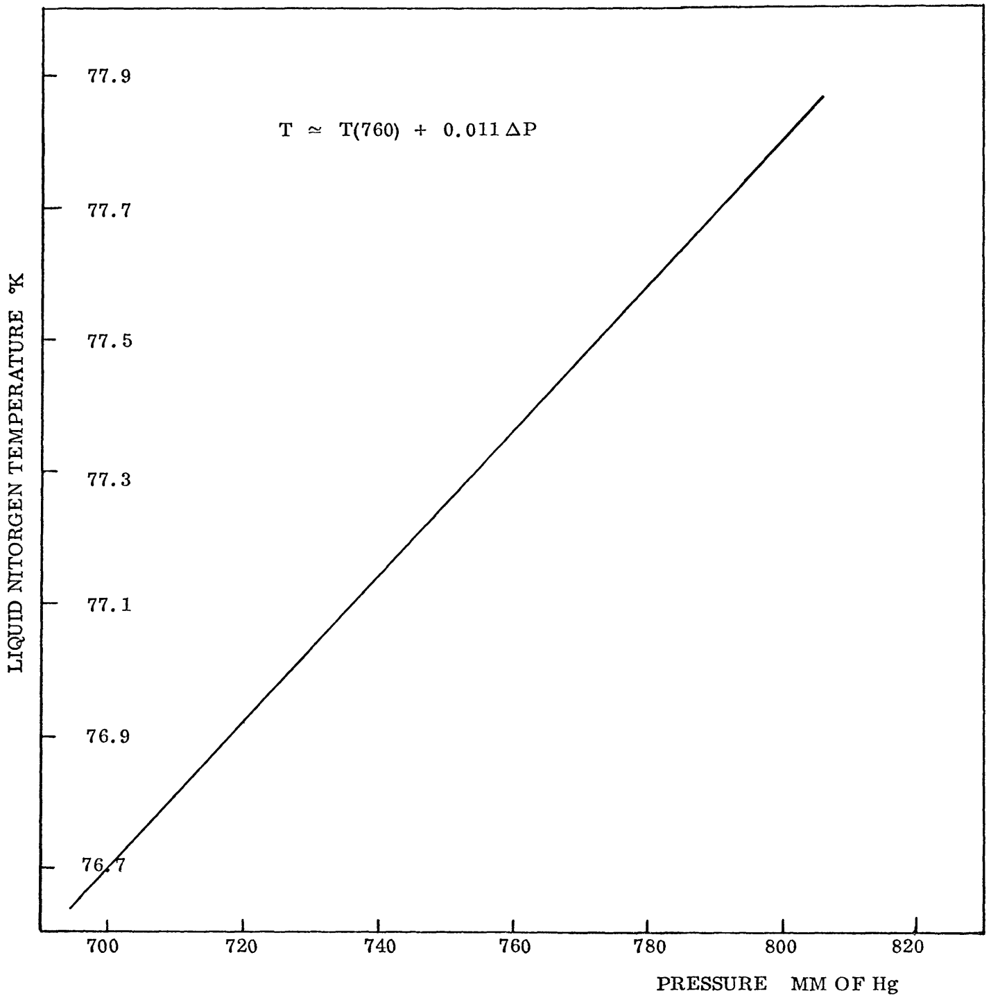
FIG. 7 — LIQUID NITROGEN TEMPERATURE VERSUS VAPOR PRESSURE
