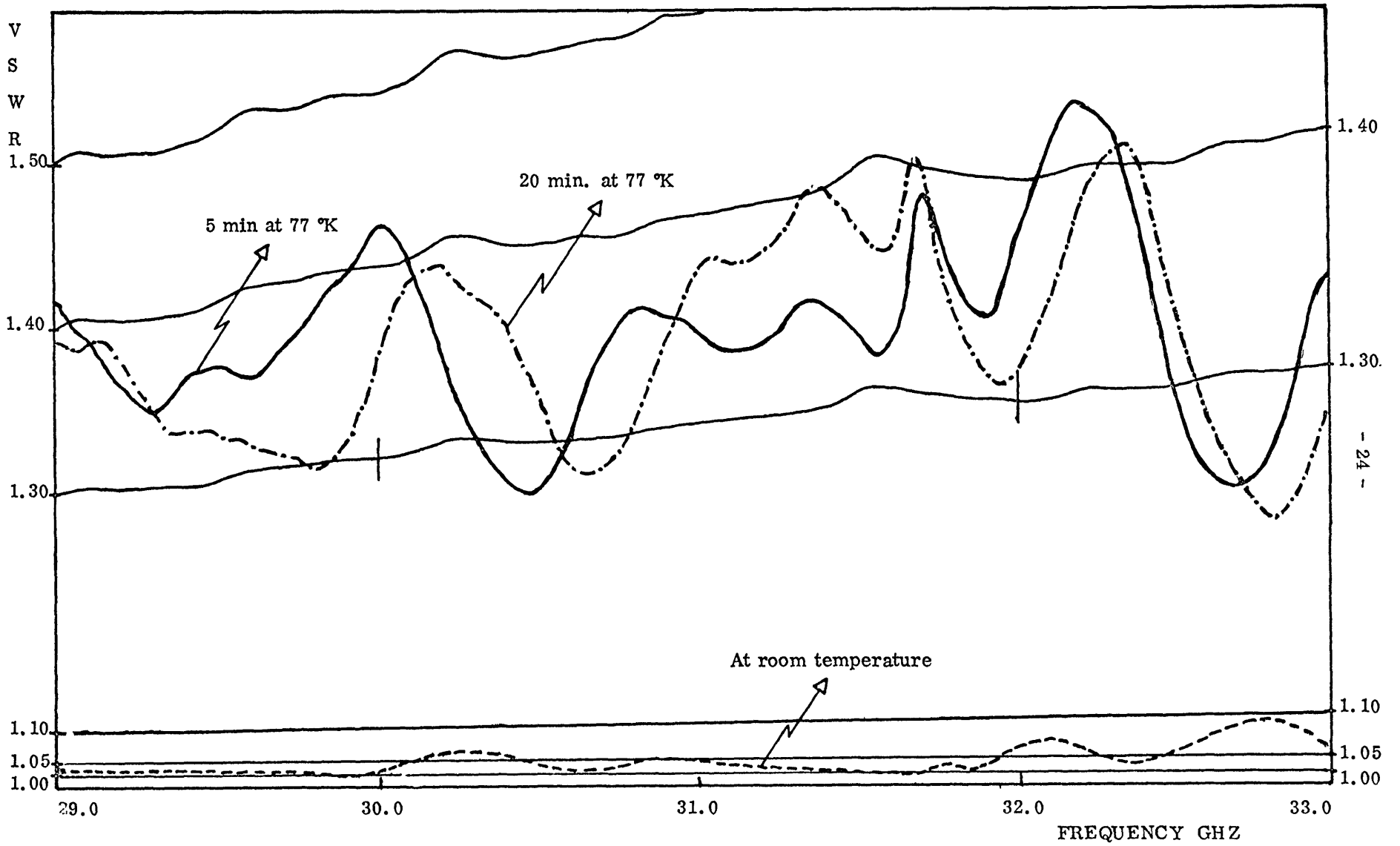
FIG. 14 - VSWR OF LABORATORY ASSEMBLED LIQUID NITROGEN LOAD
