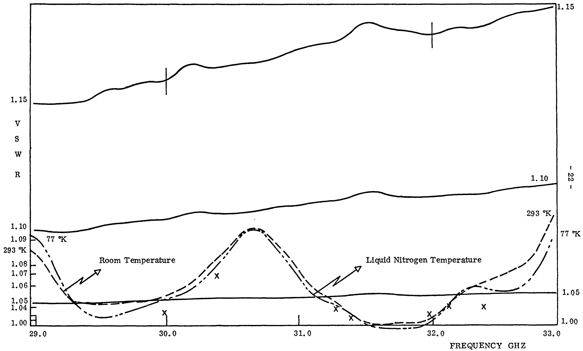
FIG. 12 - VSWR OF ADTECH LN-96 CALIBRATION LOAD
