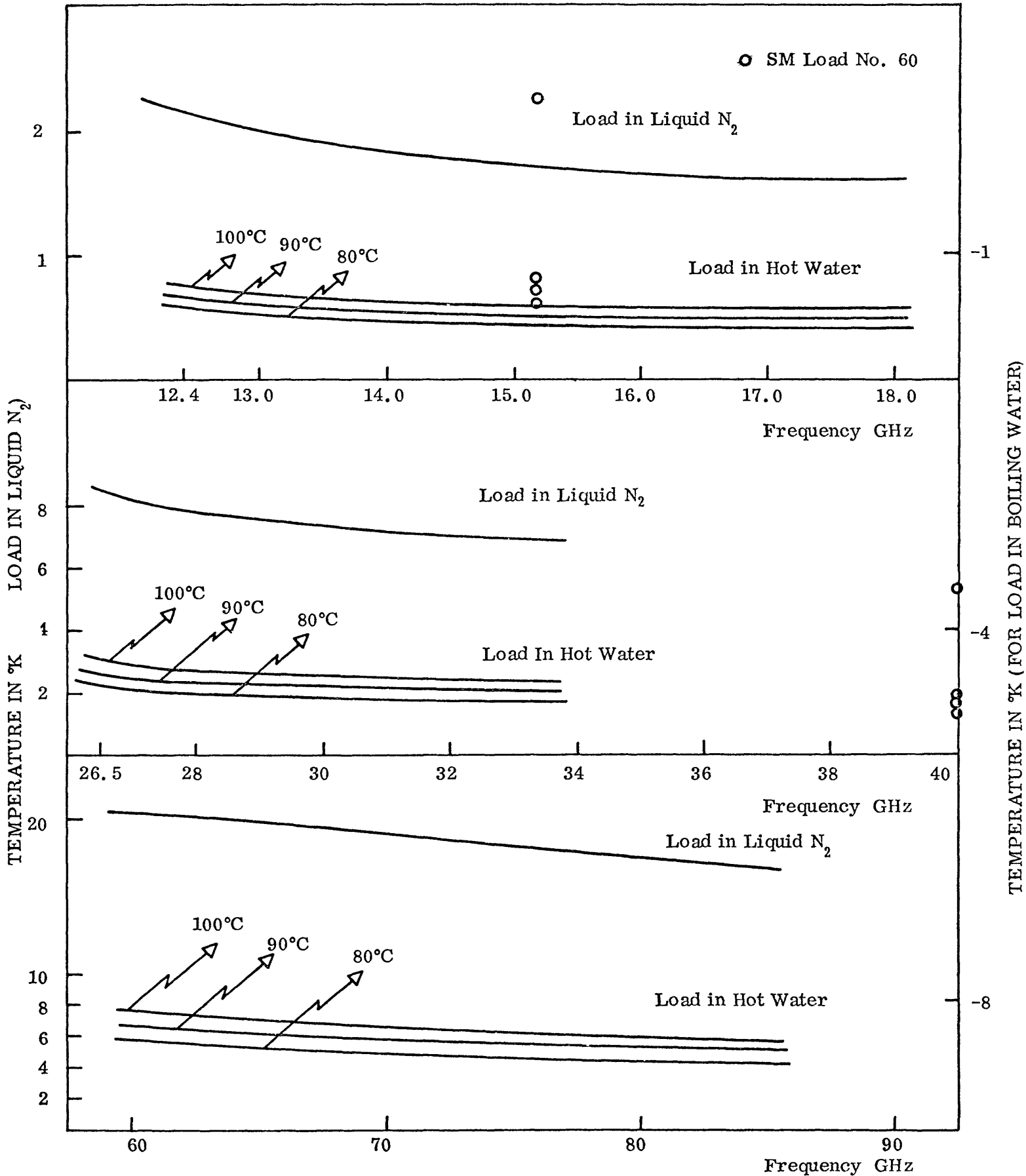
FIG. 6 — TEMPERATURE CORRECTIONS DUE TO OHMIC LOSSES IN ADTECH LOADS
