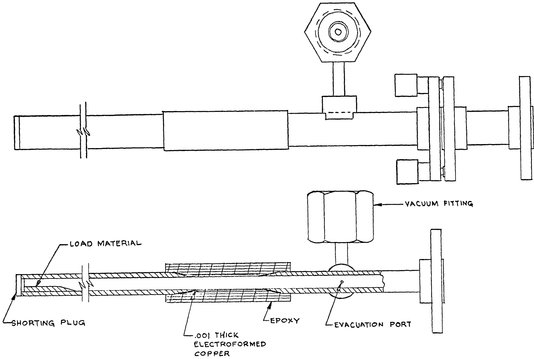
FIG. 5 - WAVEGUIDE LOAD WITH THERMAL ISOLATION SECTION
