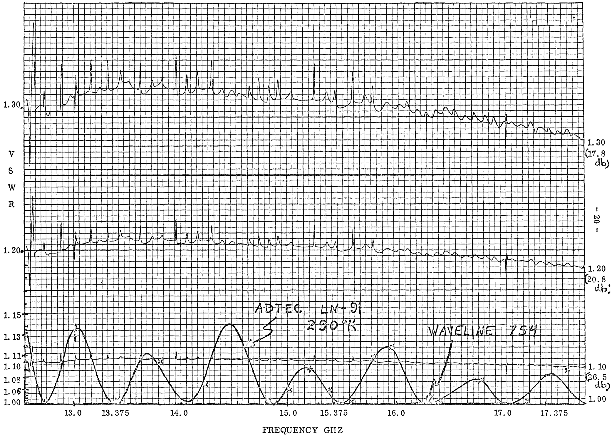
FIG. 10— VSWR OF ADVANCED TECHNOLOGY LN-91 CALIBRATION LOAD
