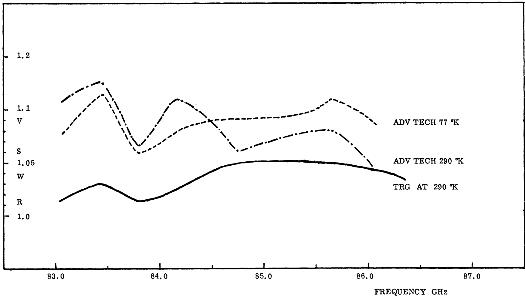
FIG. 15 - VSWR OF ADTECH LN-99 CALIBRATION LOAD
