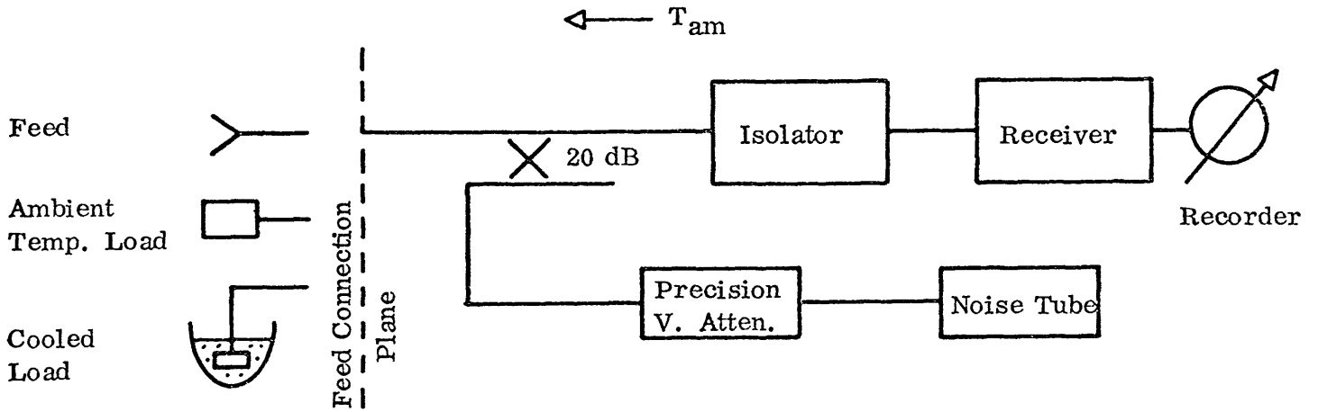
FIG. 1 - BLOCK DIAGRAM OF BASIC RADIOMETER
