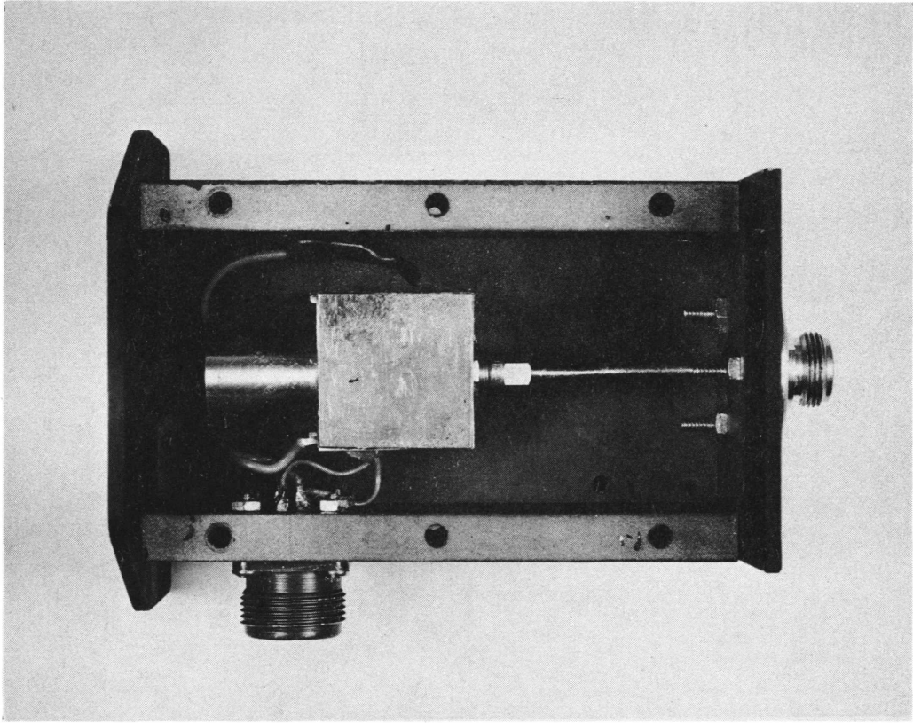
RF Load Housing with Top Heat Sink and Insulating Material Removed
