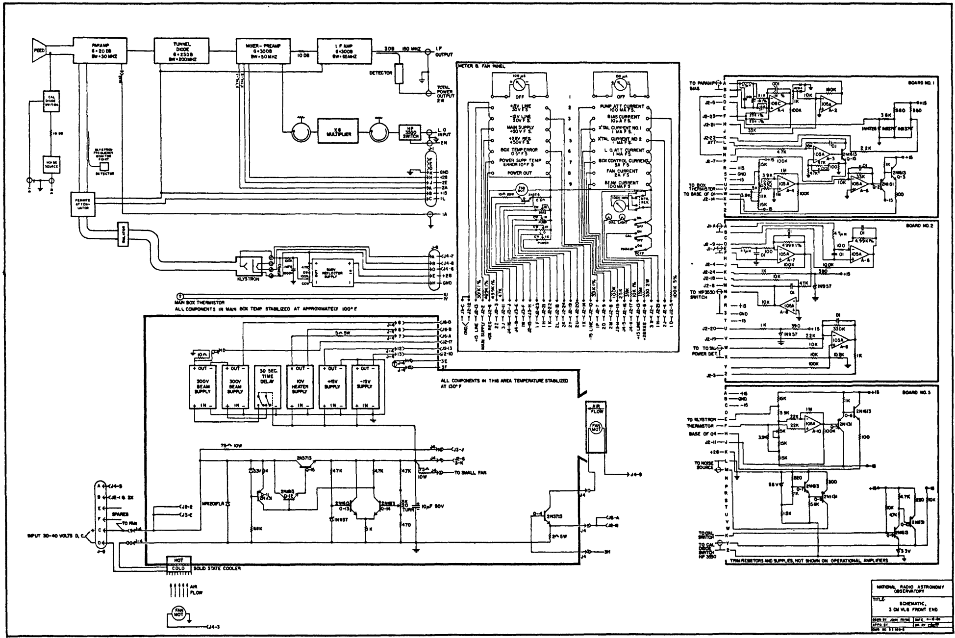
Figure 6 Circuit Diagram of 3 cm VLB Front End
