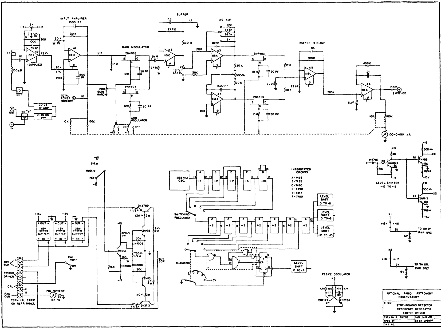
Figure 7 Circuit Diagram of Switch Driver and Gain Modulator
