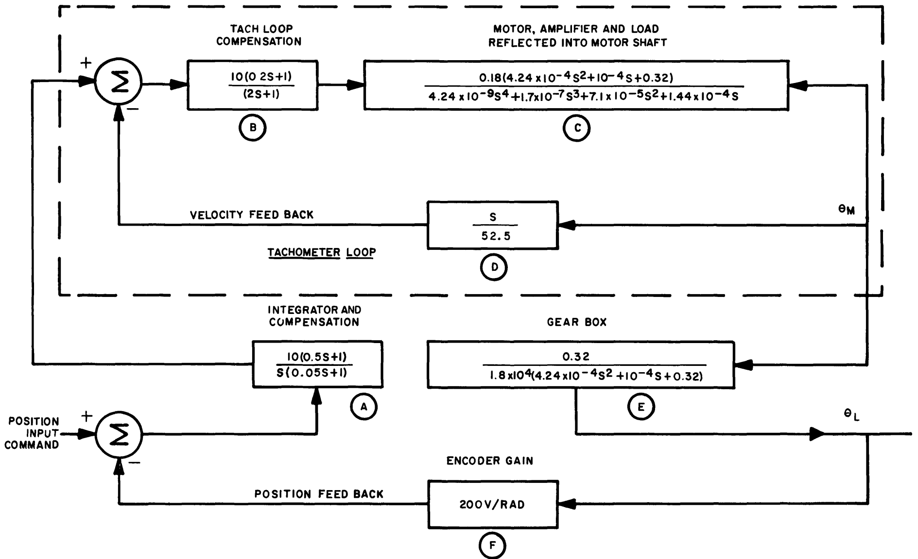
BLOCK DIAGRAM OF SERVO SYSTEM FIG. 7
