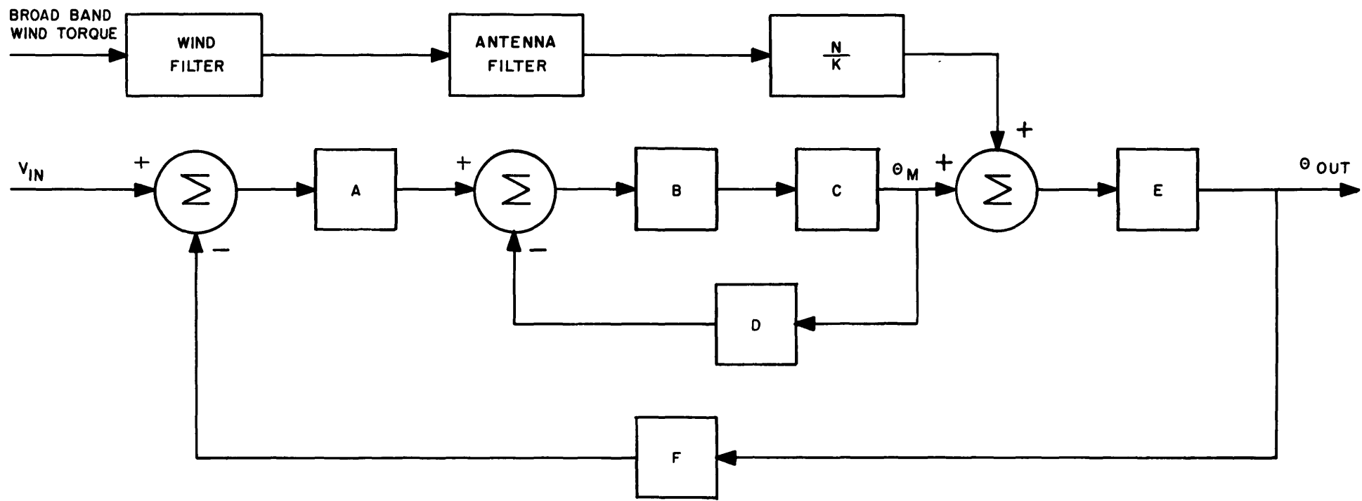
POSITION LOOP SUBJECTED TO WIND TORQUES FIG. 14
