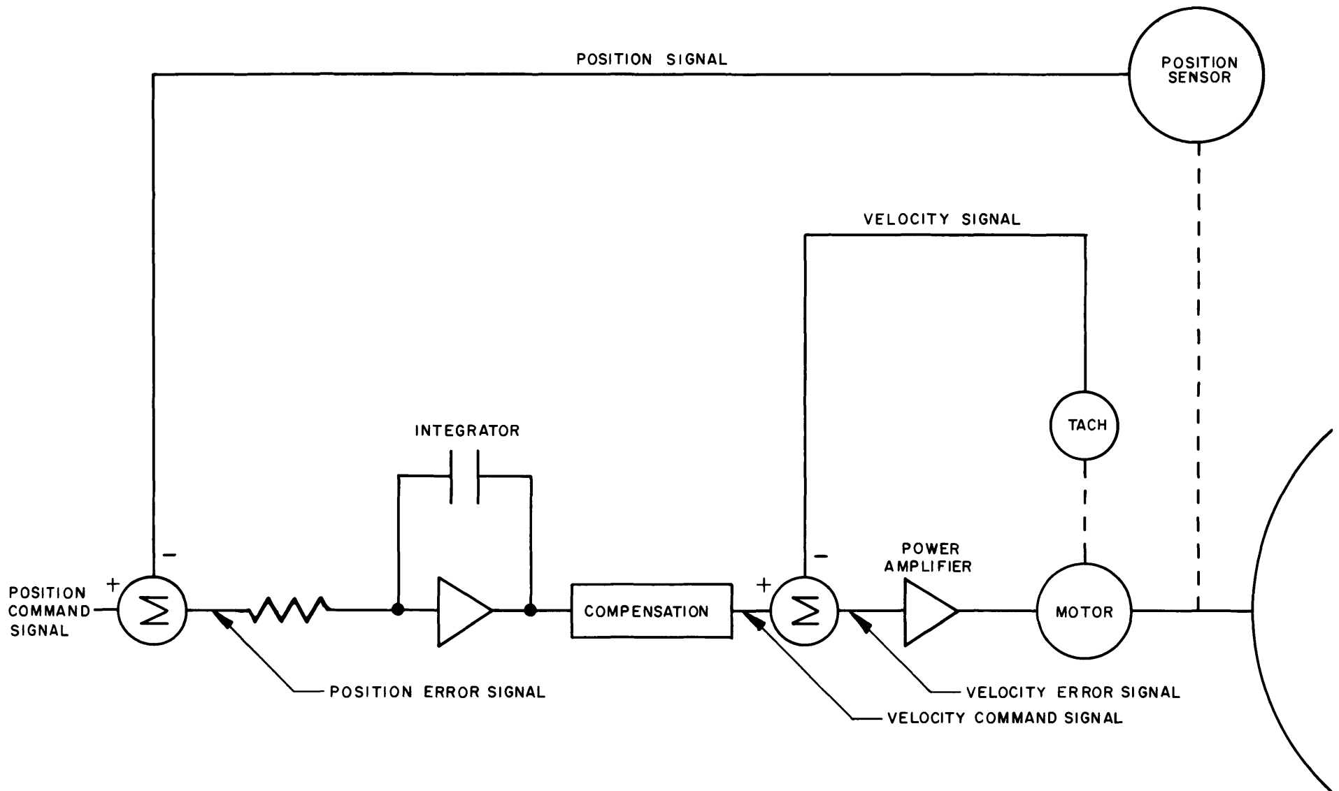
SIMPLIFIED SERVO BLOCK DIAGRAM FIG. 2
