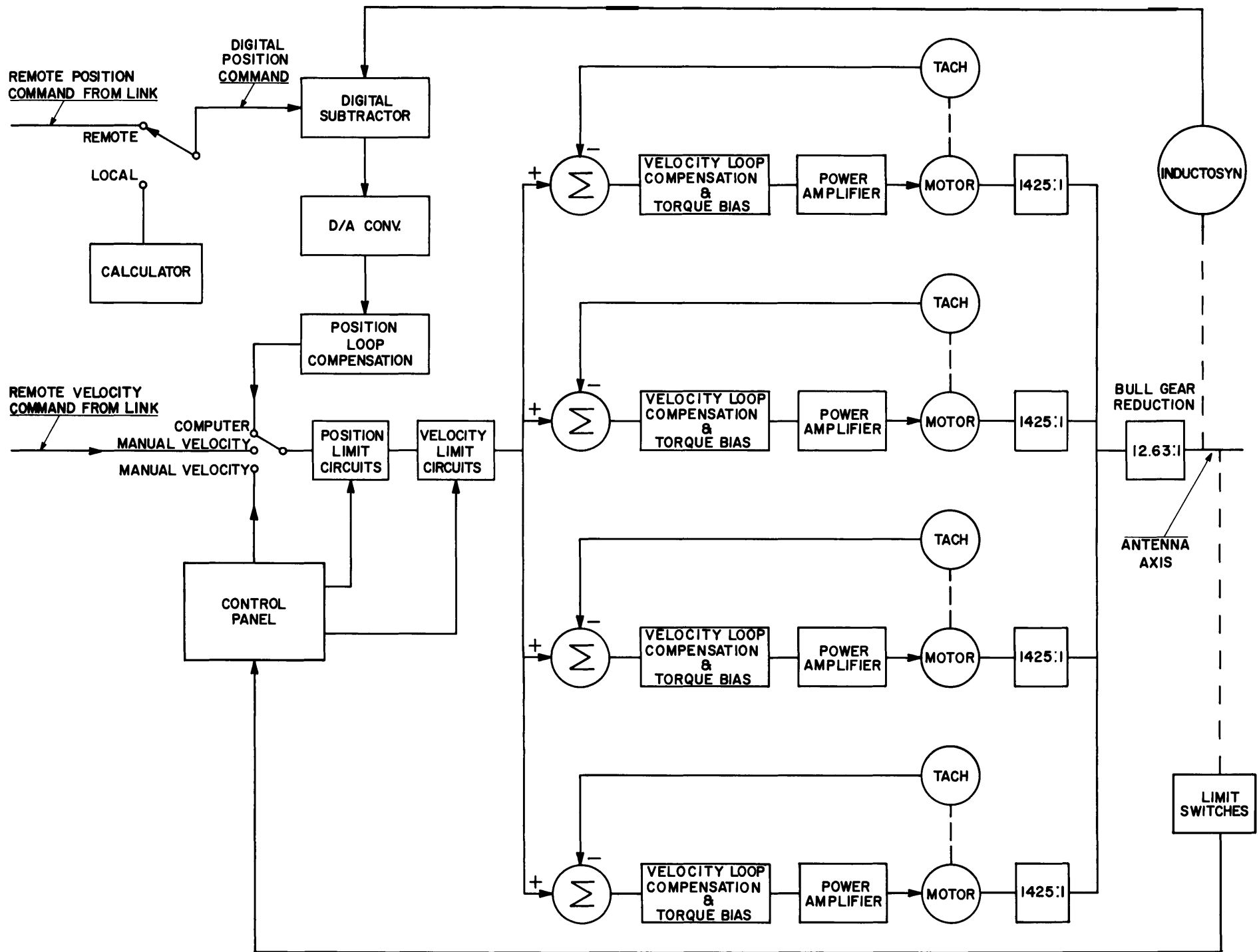
BLOCK DIAGRAM OF ONE AXIS OF CONTROL SYSTEM FIG. 1
