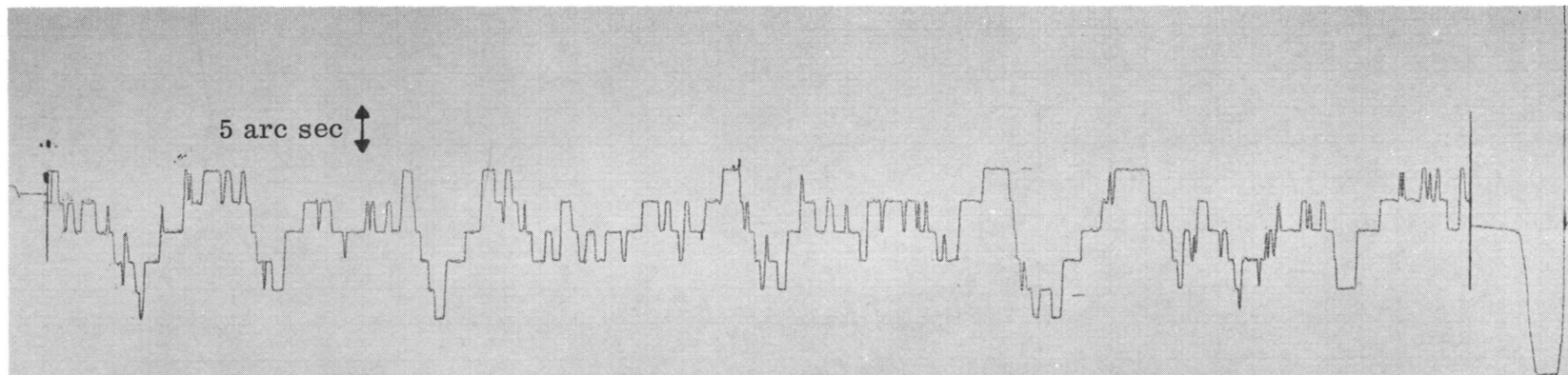
Figure 18 — Elevation Error Signal during Tracking. 1 \sigma RMS 5.5 arc sec.
