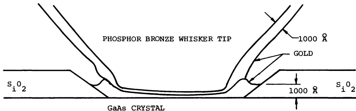
Figure 5. Plastically Deformed Whisker Tip
