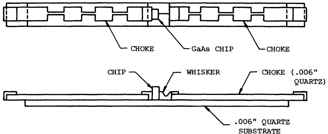
Figure 1. Diode-Choke Subassembly
