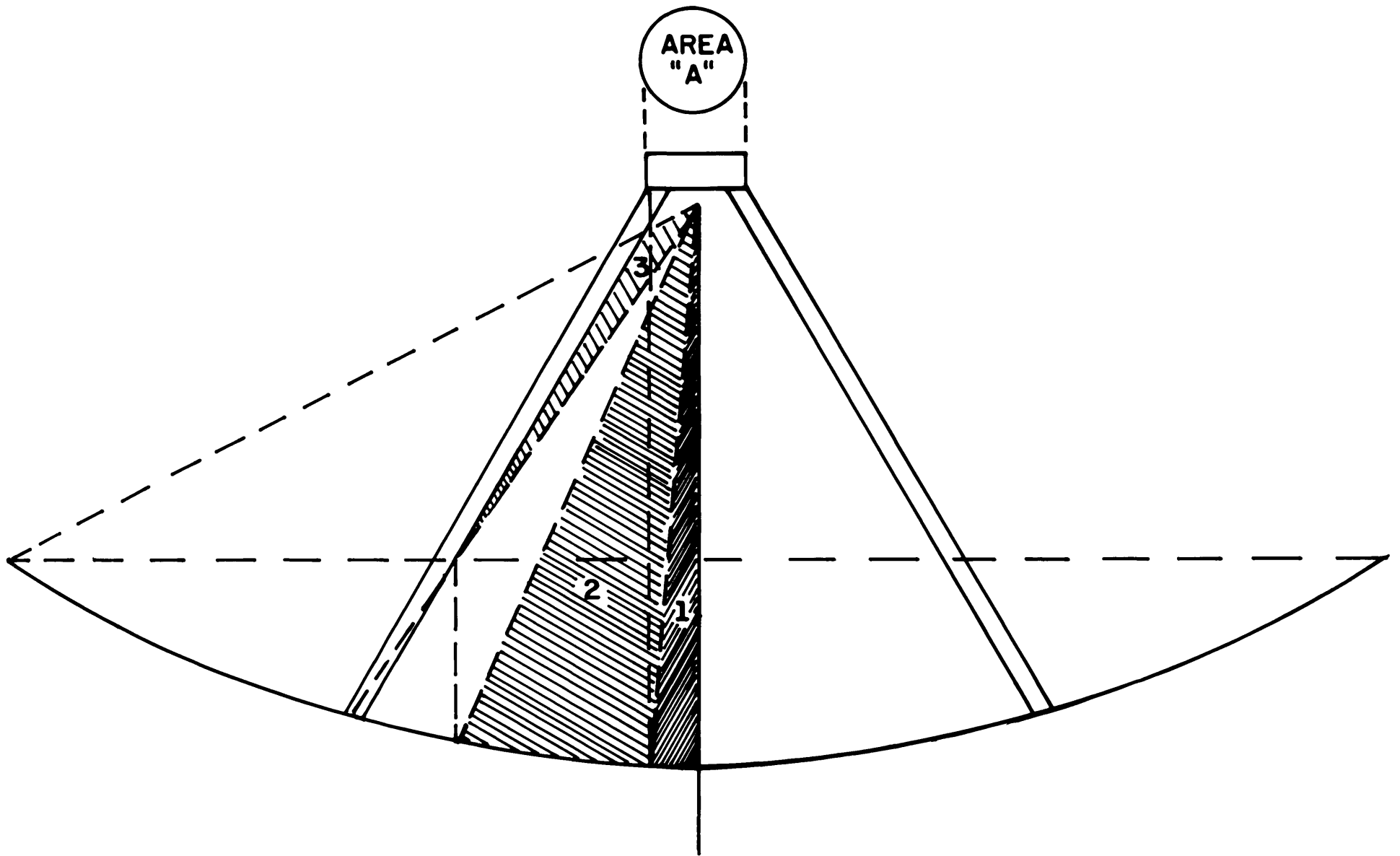
FIGURE 2. AREAS OF INTEREST IN GROUND RADIATION SCATTERING INTEGRALS.
