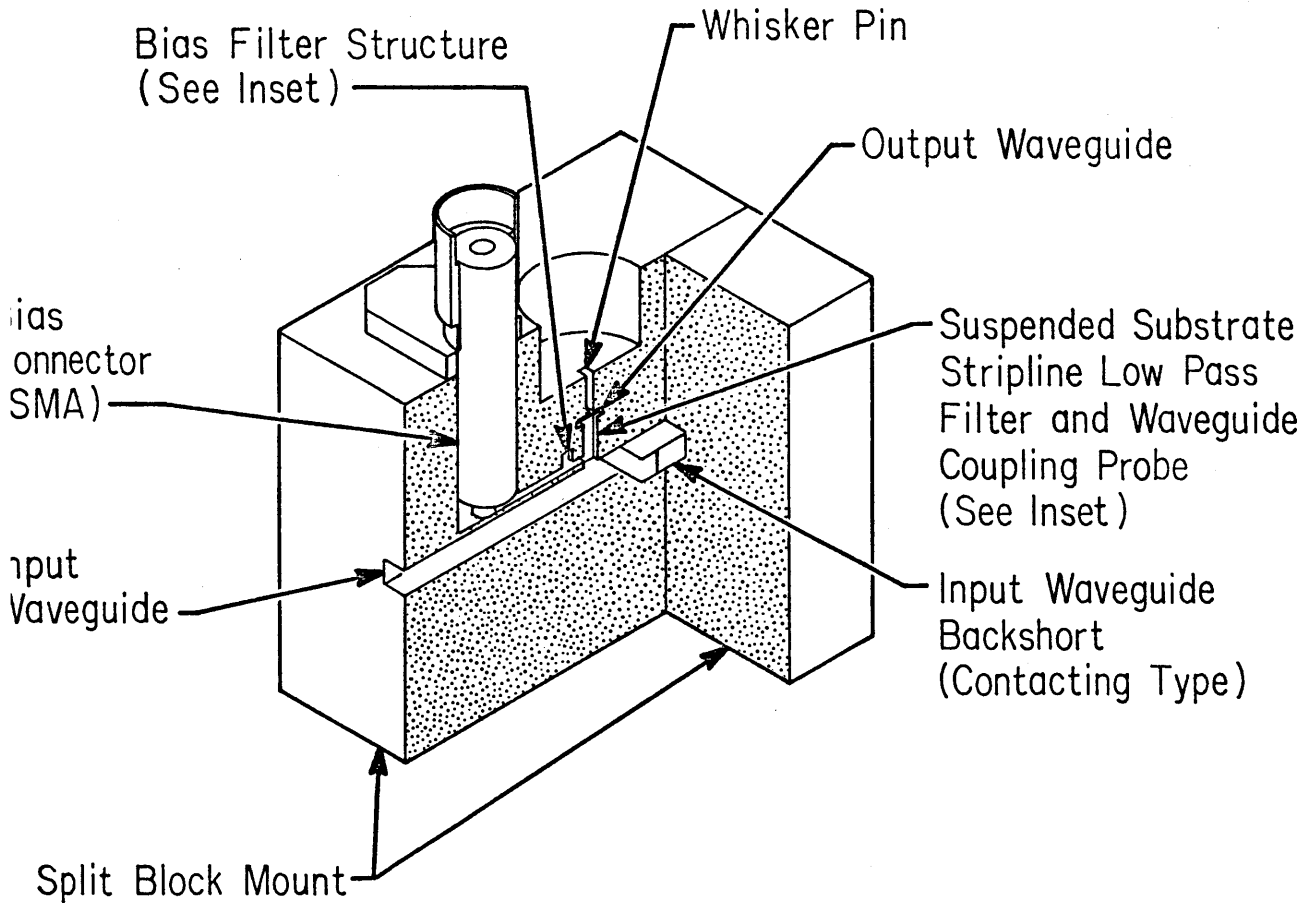
Figure 1: The NRAO crossed waveguide frequency multiplier mount.
