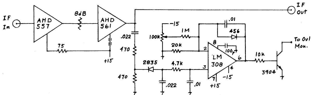
IF AMPLIFIER & OVERLOAD DETECTOR
