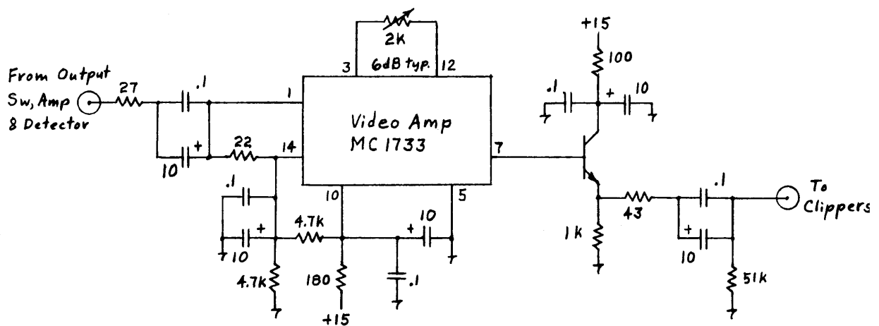
OUTPUT AMPLIFIER
