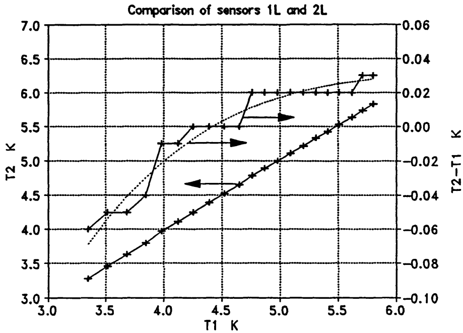
Fig. 1. The reading T2 of sensor #2L vs. the reading T1 of sensor #1L. The difference (T2-T1) is shown on the right scale. Also shown is the expression TOS = 0.03 + 0.009x + 0.004x^2 , where x = T1 - 6 (right scale).
