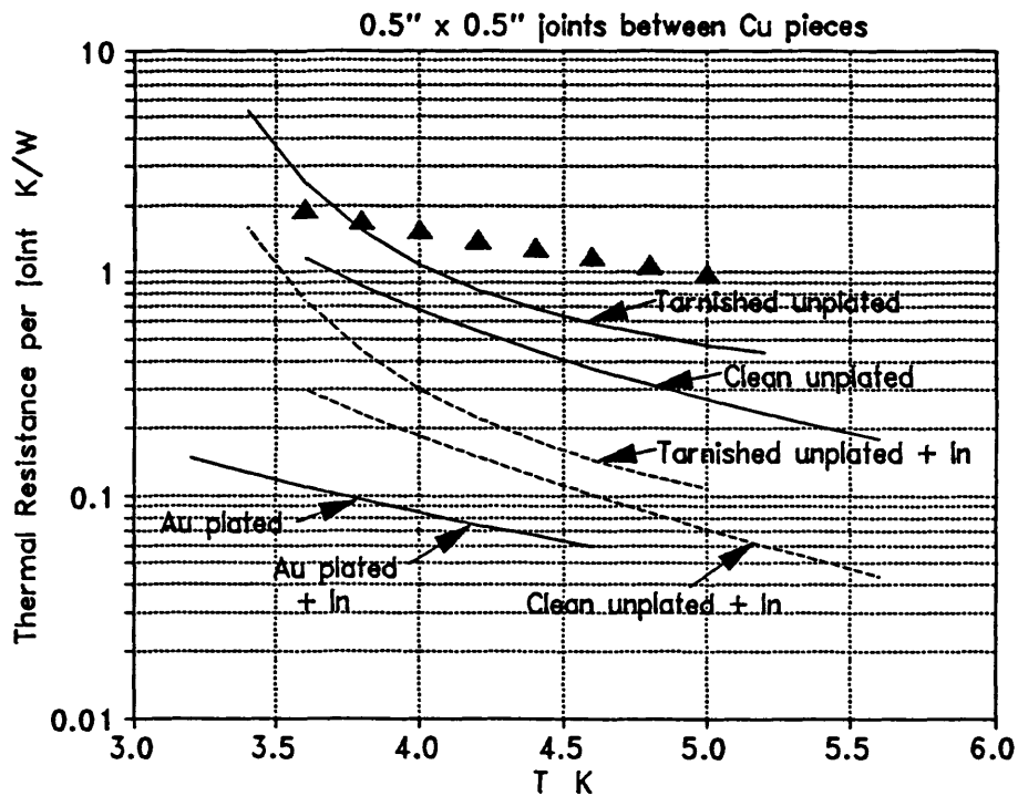
Fig. 6. Thermal resistance (per joint) of various 0.5" x 0.5" joints. Note that no significant difference was observed between gold-plated joints with or without indium. The points marked ▲ indicate the thermal resistance of an annealed high purity copper strip 3" long x 0.5" x 0.094", shown for comparison.
