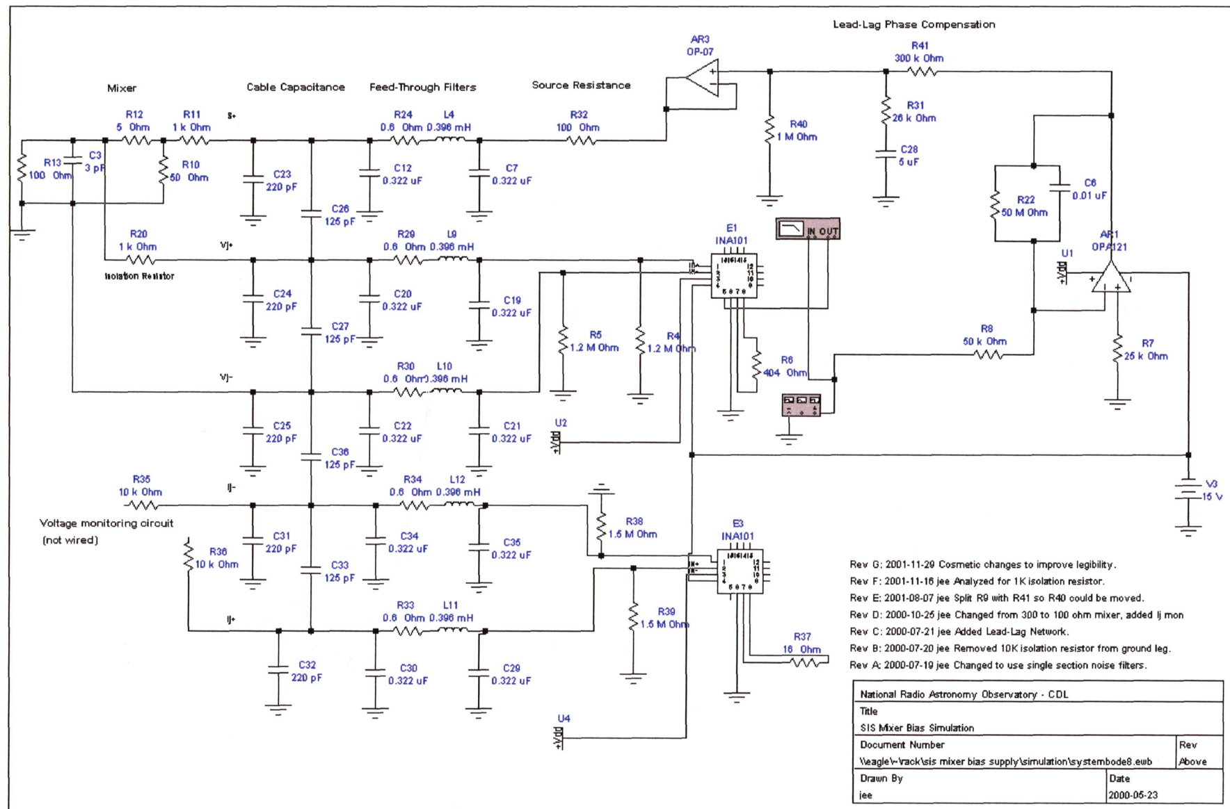
Figure 2: Circuit Analyzed by Electronics Workbench 5.12
