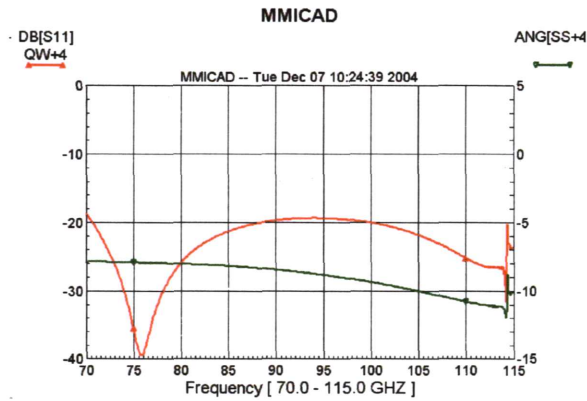
Fig. 2. Bottom block half +4 mils.
