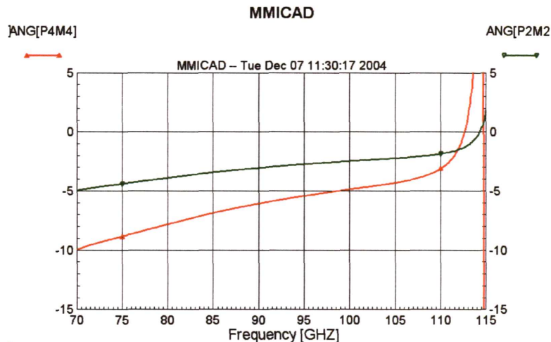
Fig. 7. Transmission phase difference for pairs of WR-10 transducers with +4 and -4 mils misalignment (red curve), and with +2 and -2 mils misalignment (green curve).
