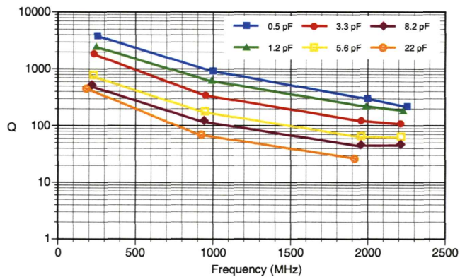
Q vs Frequency: 0201/R05L
