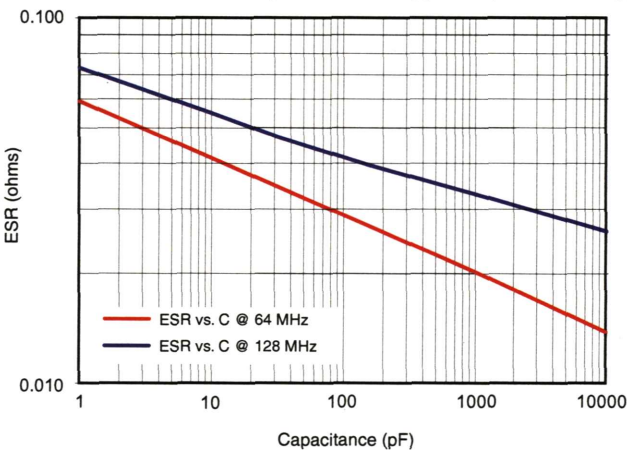
S48E ESR vs. Capacitance, Typical (Preliminary)
