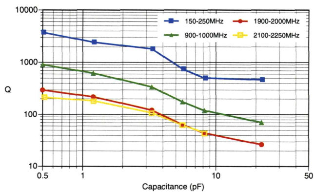
Q vs Capacitance: 0201/R05L
