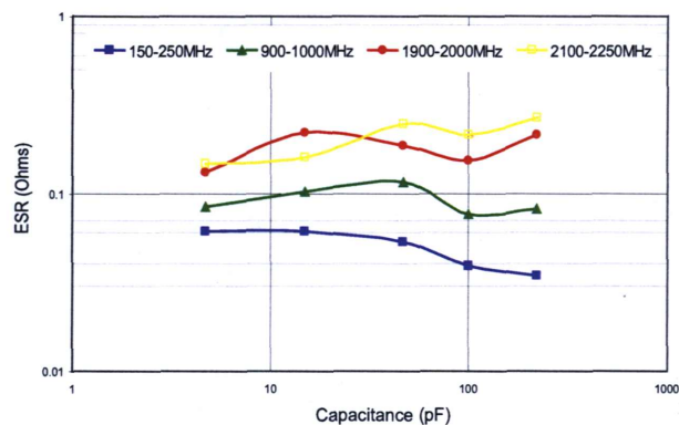
Equivalent Series Resistance: 0805/R15S
