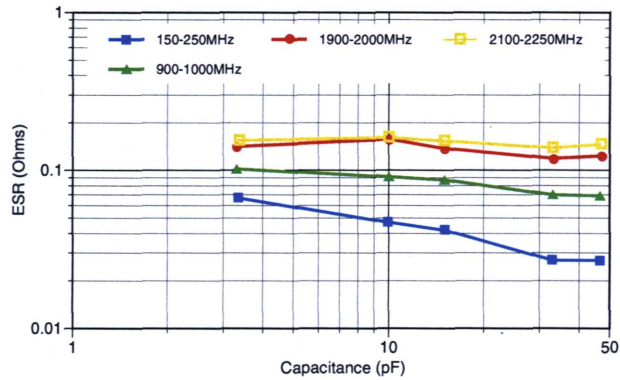
Equivalent Series Resistance: 0603/R14S
