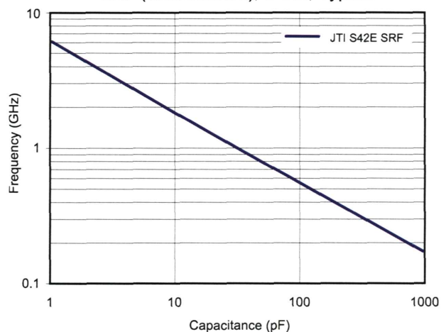
SRF (Shunt Mount), S42E, Typical
