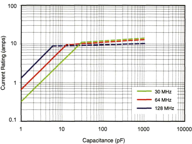
Current Rating vs. Capacitance, S48E, Typical (Preliminary)
