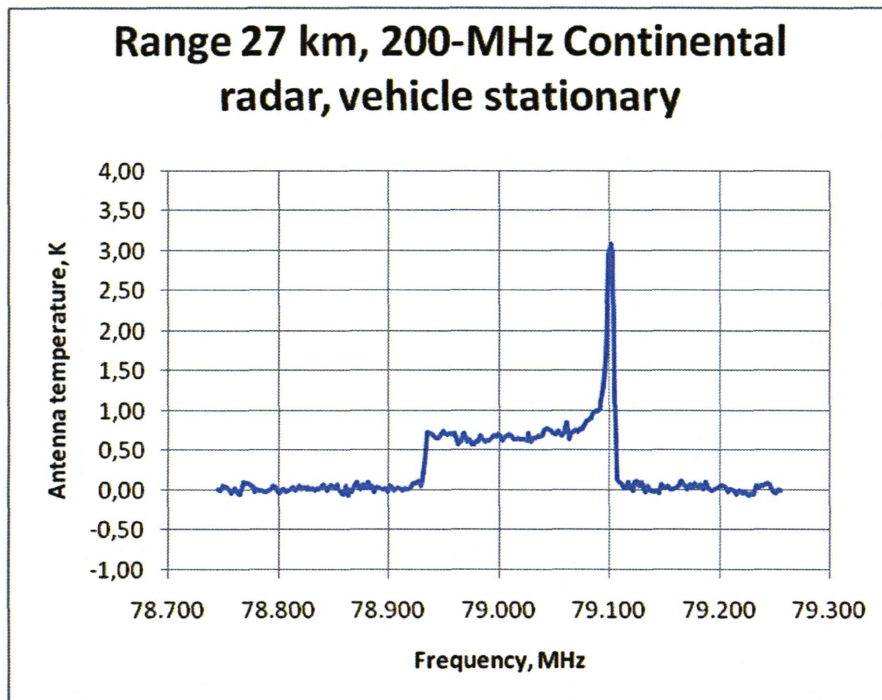
Figure 6 At a range of 26.9 km, this is the emission seen from the Continental 200-MHz radar, with the vehicle stationary. The average plateau of emission has a brightness of 0.68 K, while the high frequency spike is 3.08 K. The noise in the spectrum on either side of the emission is 0.038 K, close to the theoretical receiver noise of 0.036 K.
