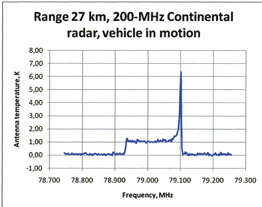
Figure 7 At a range of 26.9 km, the emission from the Continental 200-MHz radar, with the vehicle in motion. The plateau of emission has a brightness of 1.07 K, and the high frequency spike 6.4 K. The receiver noise on either side of the emission is 0.053 K, very close to the theoretical receiver noise of 0.049 K.
