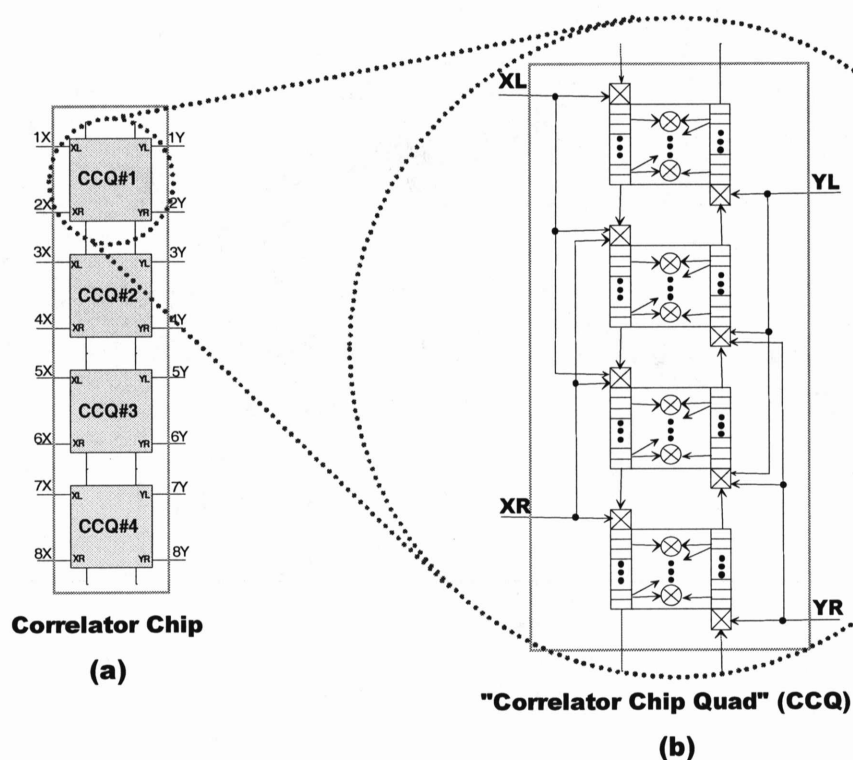
Figure 2 Correlator chip functional block diagram showing data routing paths. In (a) an overall diagram of the chip is shown. The chip contains 4 "Correlator Chip Quads" (CCQs)—each one containing 4, 128 complex-lag cross-correlators (b). The chip can accept data from up to 8 'X' and 'Y' basebands or 4 baseband pairs (or any combinations thereof) and perform all necessary cross-correlations. Correlators within CCQs can be concatenated and CCQs within a correlator chip can be concatenated for longer lag chains on fewer basebands.
