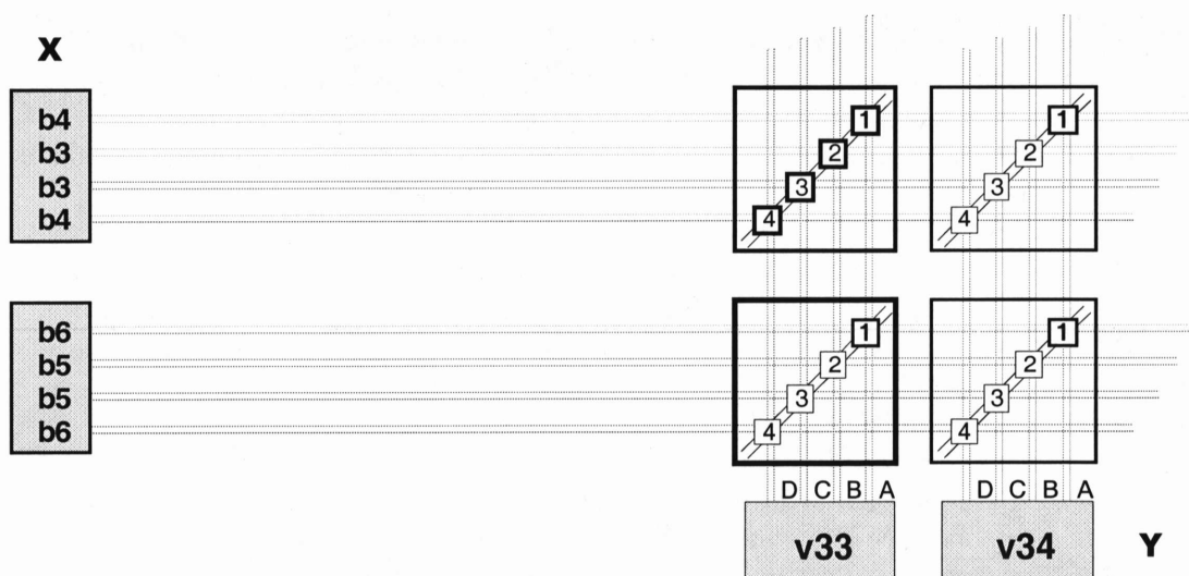
Figure 6 Portion of the Baseline Board of Figure 4 where we want to perform VLBA x VLA correlations.
