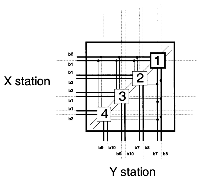
Figure 17 Correlator chip and 1 GHz station assignments for correlating all 8 baselines in the upper half of Figure 16. These are the assignments for 8 sub-band correlators—the other 8 sub-band correlators have different assignments to correlate the bottom 8 baselines.
