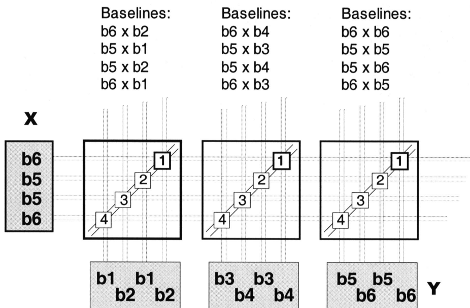
Figure 5 Close up of VLBA-only cross-correlations showing the X and Y station assignments that allow 4 baselines (2 x 2 parallelogram) to be correlated without any additional routing resources on the correlator chip or the Baseline Board.
