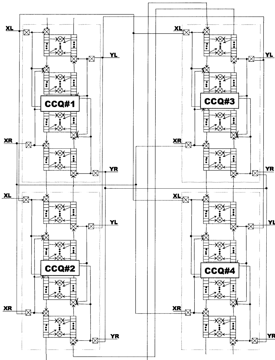
Figure 8 Block diagram of the modified correlator chip architecture which includes the minimum additional routing resources (highlighted in blue) to allow VLA x VLBA and VLBA x VLA (16 GHz with 4 GHz) correlations. Here, CCQ#1 can be thought of as the master, and CCQs 2 through 4 are the slaves that can either connect to their own data inputs or to the master's data inputs.
