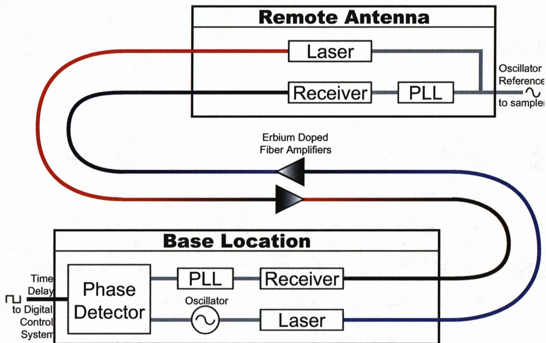
Figure 2: Double Fiber Synchronization System
