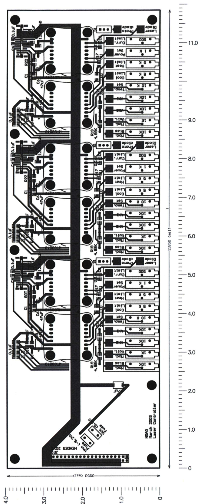
Figure 10: PCB layout, top side
