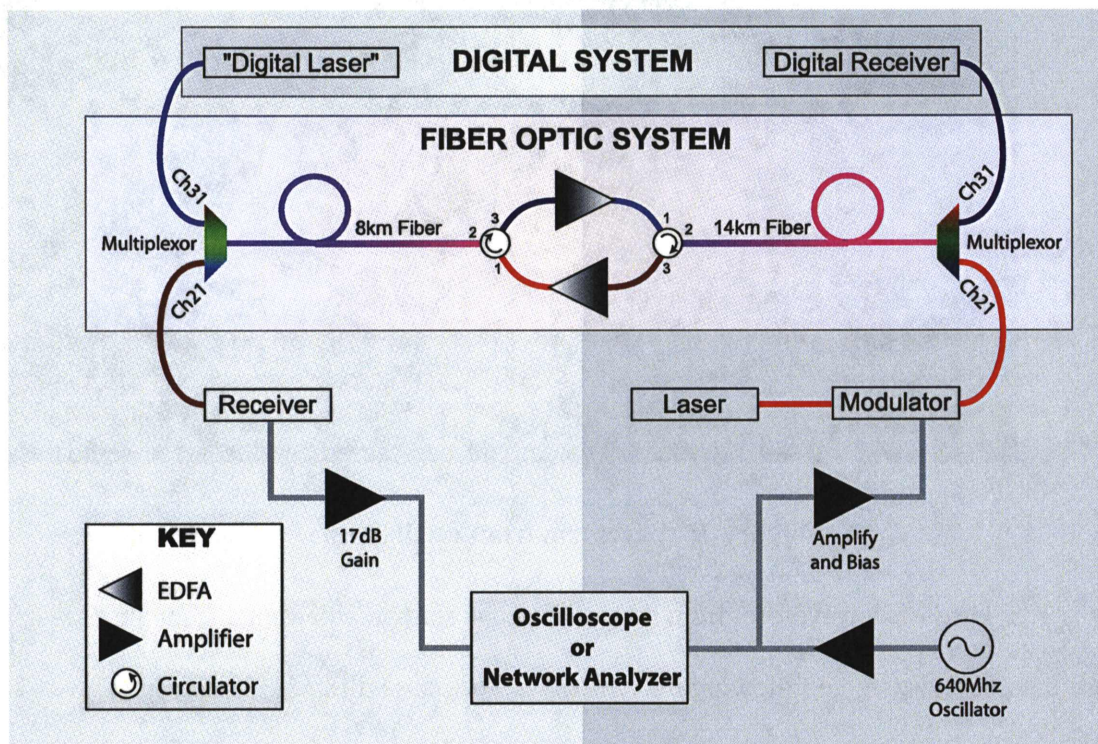
Figure 6: Experimental Setup
