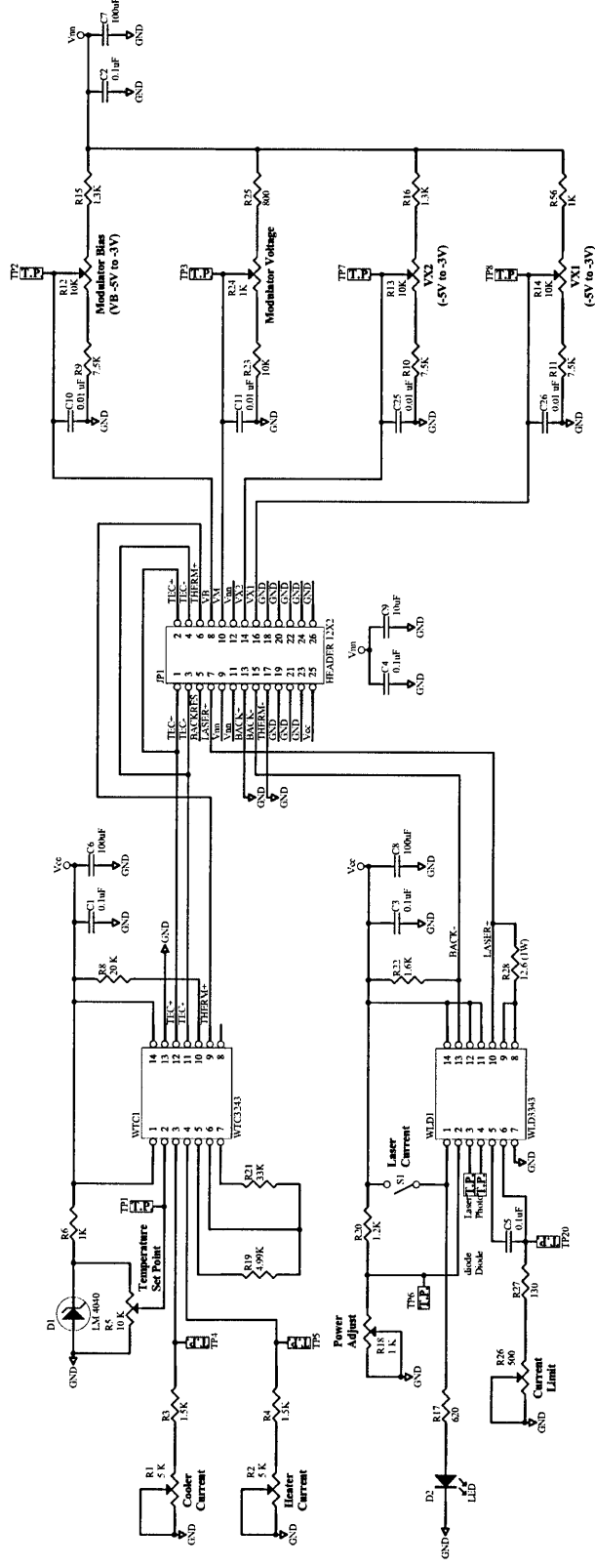
Figure 9: Laser controller schematic
