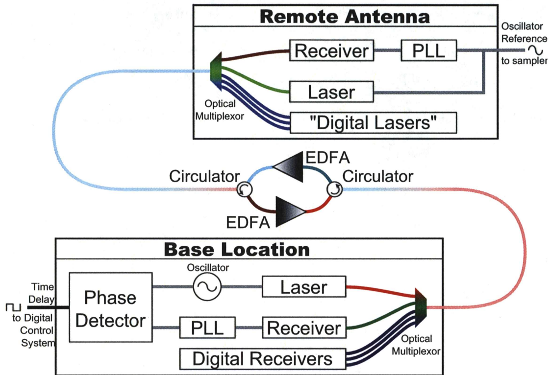
Figure 4: Overall System Design
