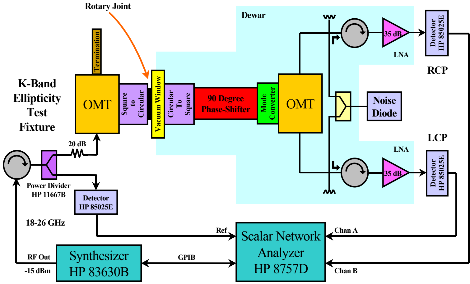
Figure 1 : K-Band Receiver and Ellipticity Test Fixture Block Diagram
