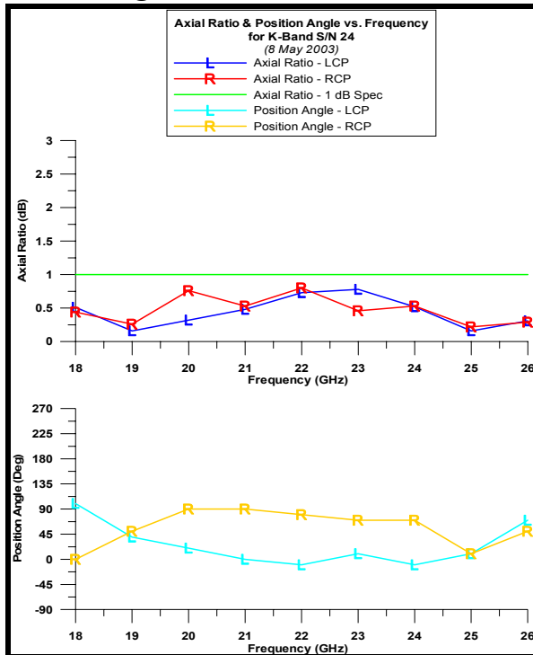
Figure 6a : K-Band S/N 24
