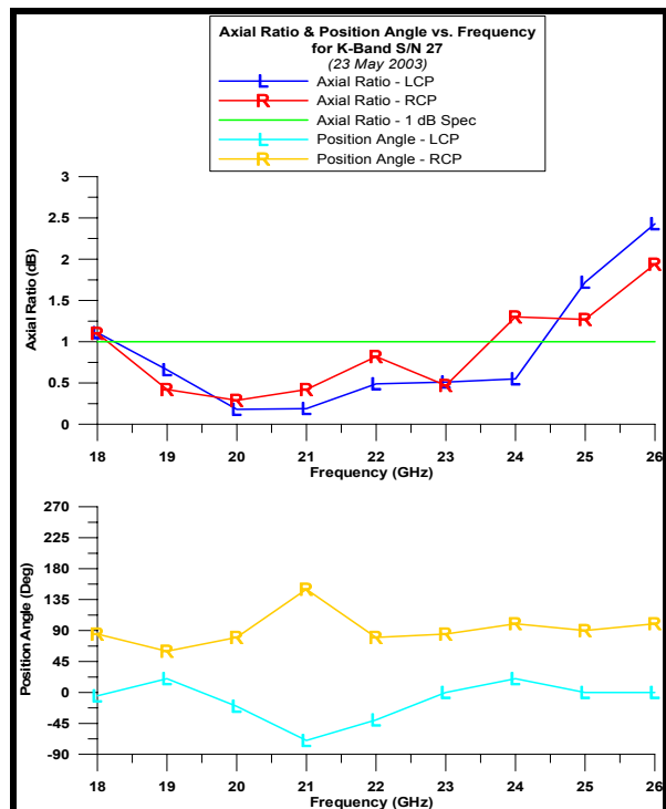
Figure 6d : K-Band S/N 27
