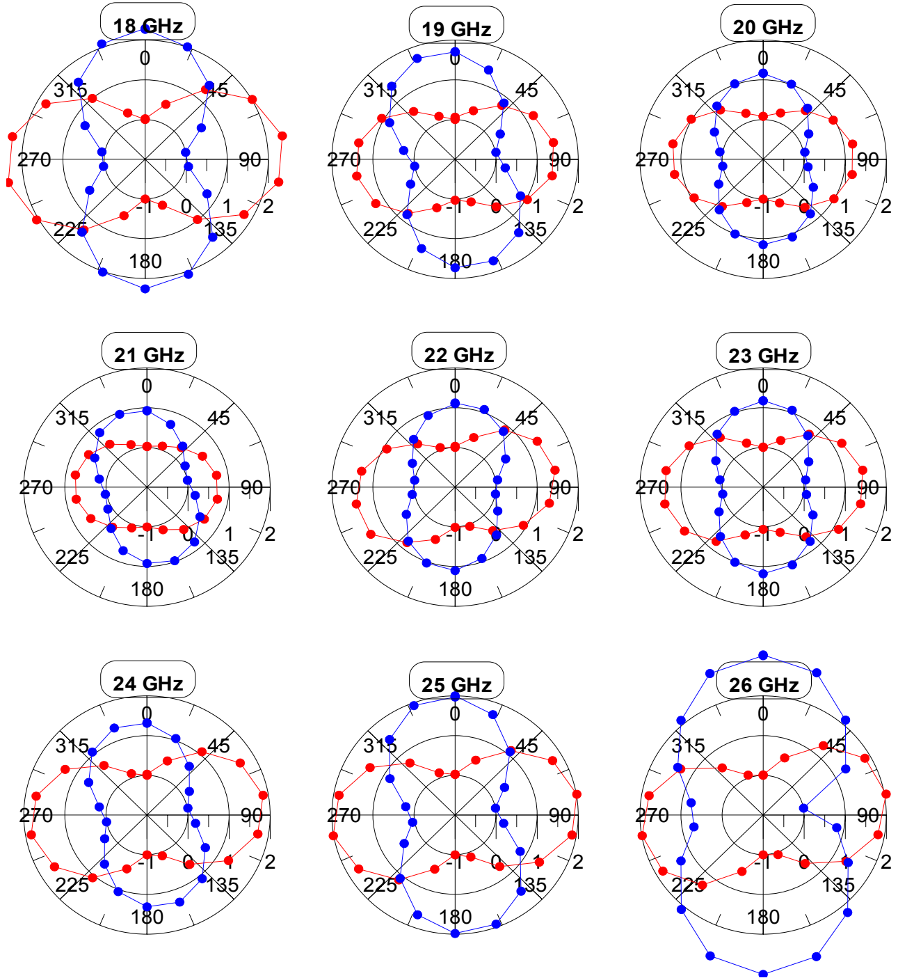
Figure 4 : K-Band S/N 26 Ellipticity Test Measurements
