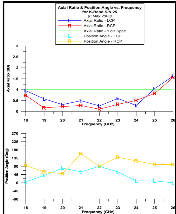
Figure 6b : K-Band S/N 25
