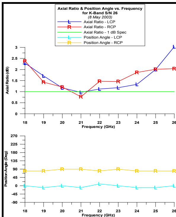
Figure 6c : K-Band S/N 26
