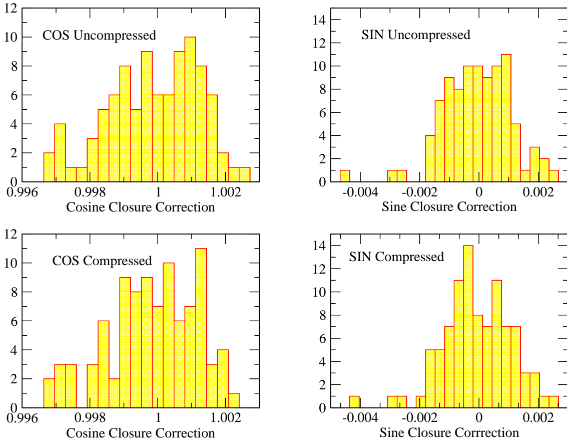
Figure 8: The closure corrections (averaged over the dataset) for the baselines utilizing antennas 1, 2, 22 and 28. The upper pair show the COS and SIN corrections for uncompressed data, the bottom pair for the compressed data. There is no statistical difference between these.
