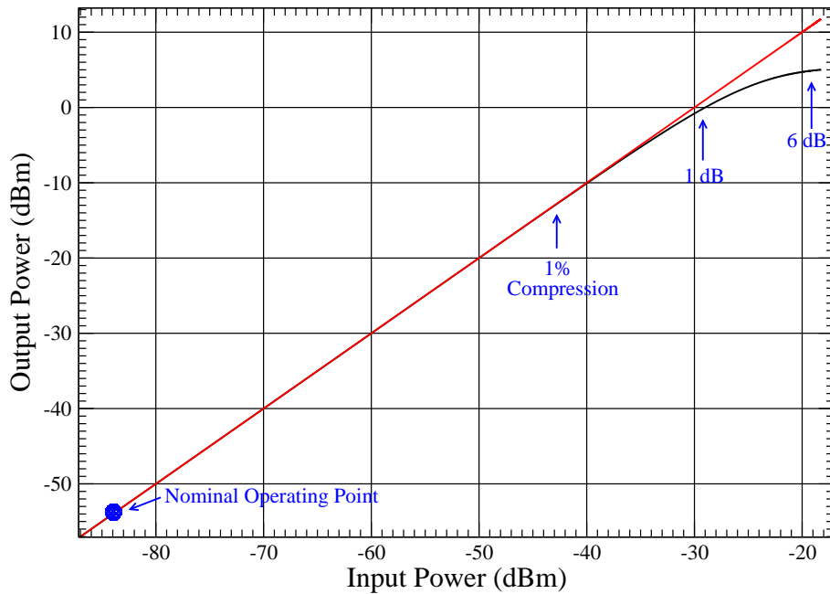
Figure 2: The approximate power response of the VLA C-band amplifiers. The power transfer curve is an approximation. The nominal operating point (defined by P = kT\Delta\nu , with \Delta\nu = 8 GHz), the 1%, 1dB, and 6dB compression points are marked.
