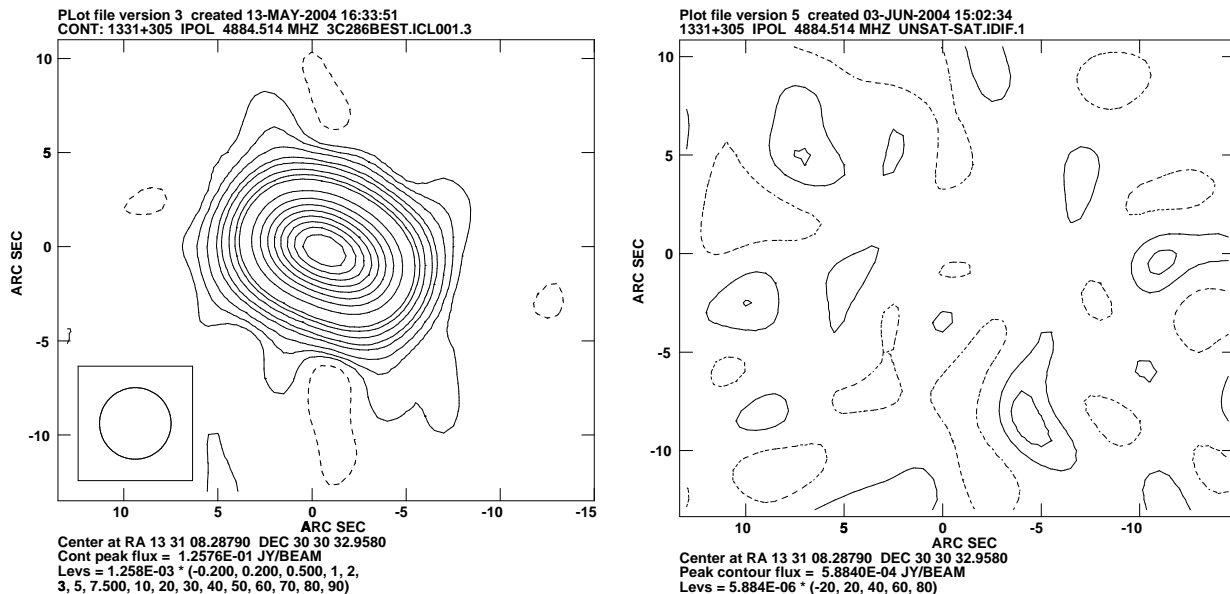
Figure 6: (Left Panel) The calibration source 3C286, at 6cm, with 3.8 arcseconds resolution. A 7.3 Jy point source has been removed from the (0,0) coordinate. This model of the source, made with the uncompressed data, was used for calibration of all data. (Right Panel) The difference image between the ‘compressed’ and ‘uncompressed’ images of 3C286. The rms noise is about 50 \mu\text{Jy}/\text{beam} . No measurable difference is seen.
