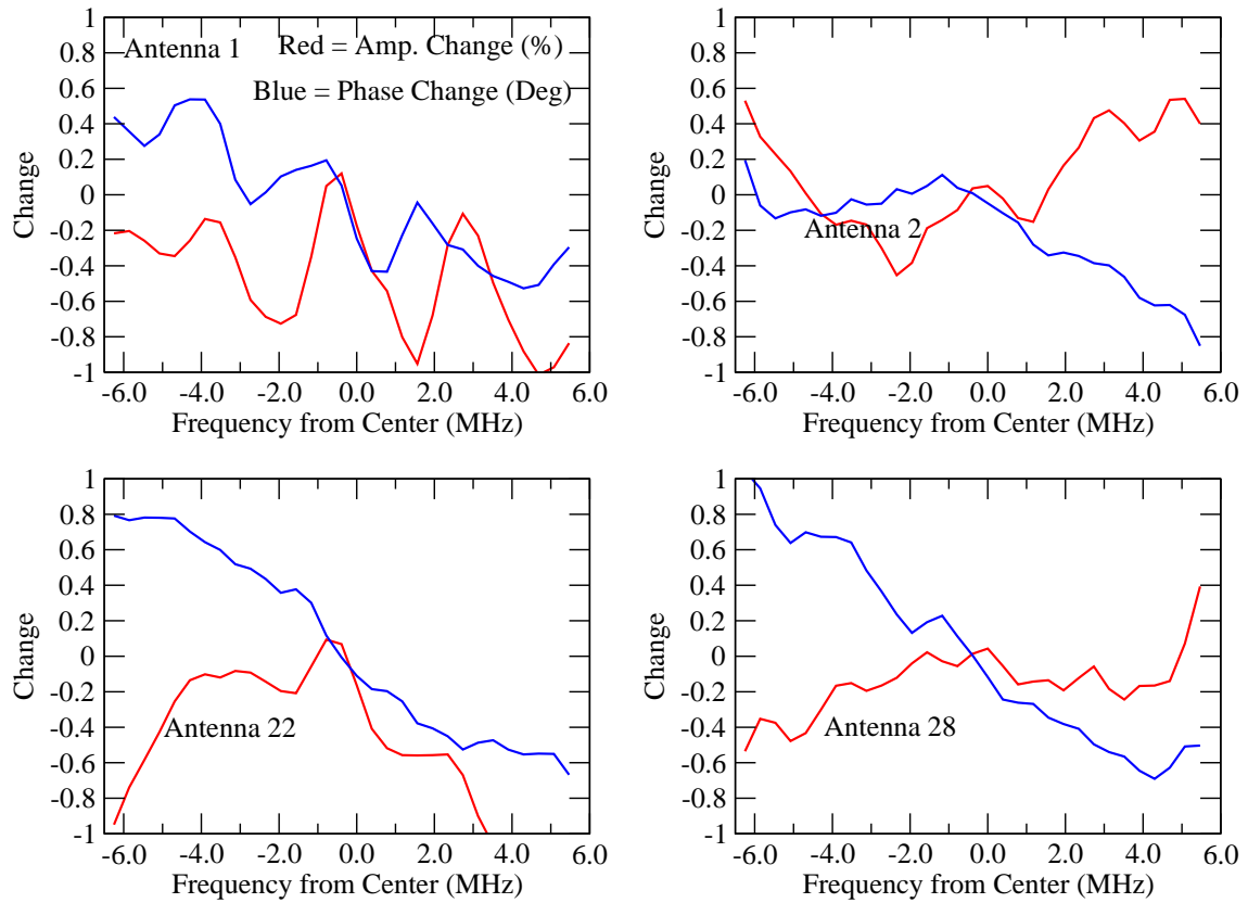
Figure 9: The difference in the bandpass amplitude (red) and phase (blue), for the four modified antennas, between the signal on and signal off states. The phase slope amounts to a \sim 0.25 nsec change in delay,
