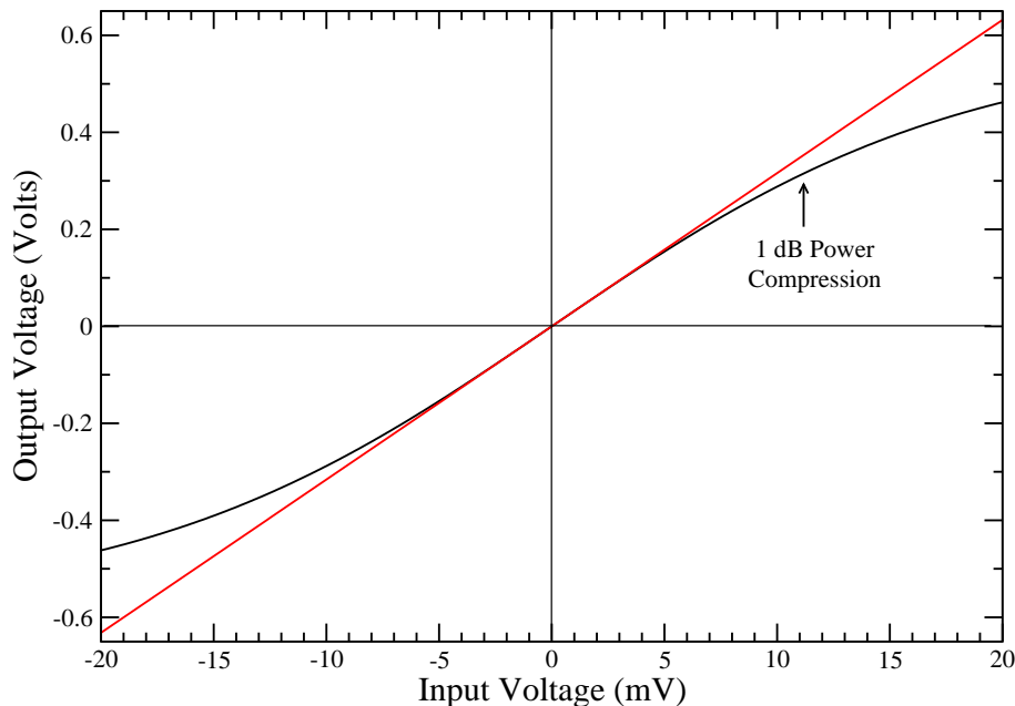
Figure 1: An amplifier model, believed to be a reasonable description of the C-band VLA system. The black line shows the actual relation between input and output voltages, the red line is the extrapolation of the low-voltage relation. The normal operating input voltage is typically a few microvolts. For comparison, the peak voltage of an input sinusoid sufficient to cause 1 dB power compression is marked.
