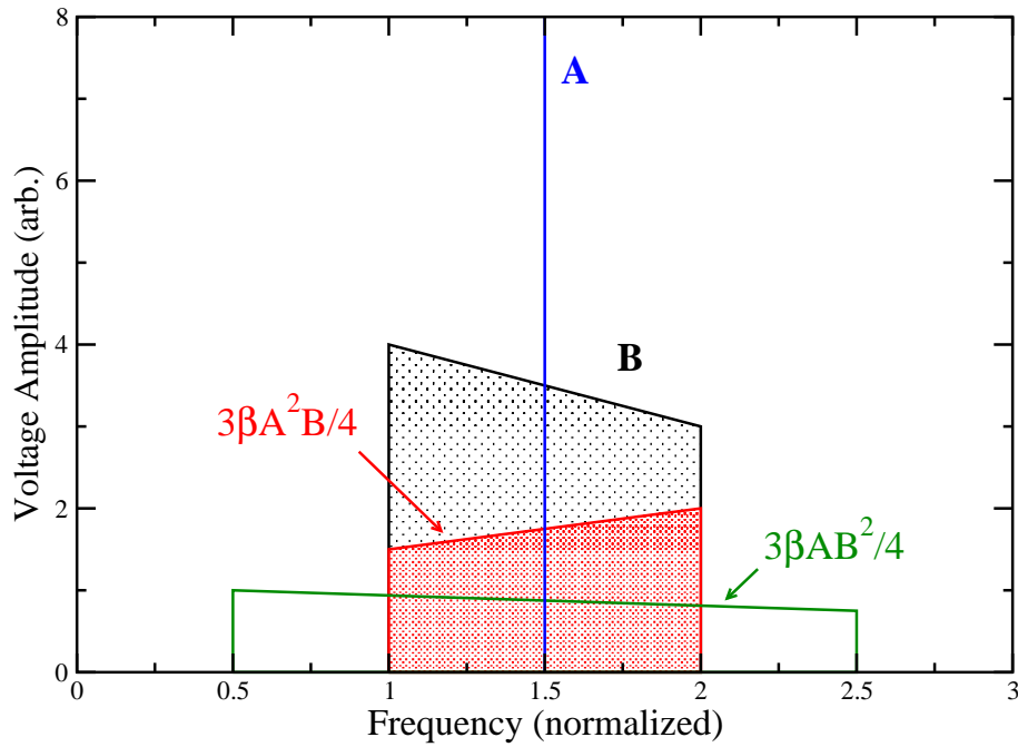
Figure 3: Showing the spectral relationships for a strong CW signal and broad-band noise power extending over a 2:1 frequency ratio. The blue spike ('A') represents the RFI tone. The black stippled area represents the actual noise at its true frequency. The red stippled area shows the stronger 'aliased' component, the green rectangle shows the weaker term.
