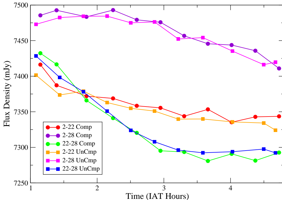
Figure 7: The calibrated visibilities for the three baselines with the maximum input signal power, with that power on and off. No significant difference is seen in these visibilities between the C and U states, indicating that any change in coherence closure caused by the high signal power level is less than 0.1%.
