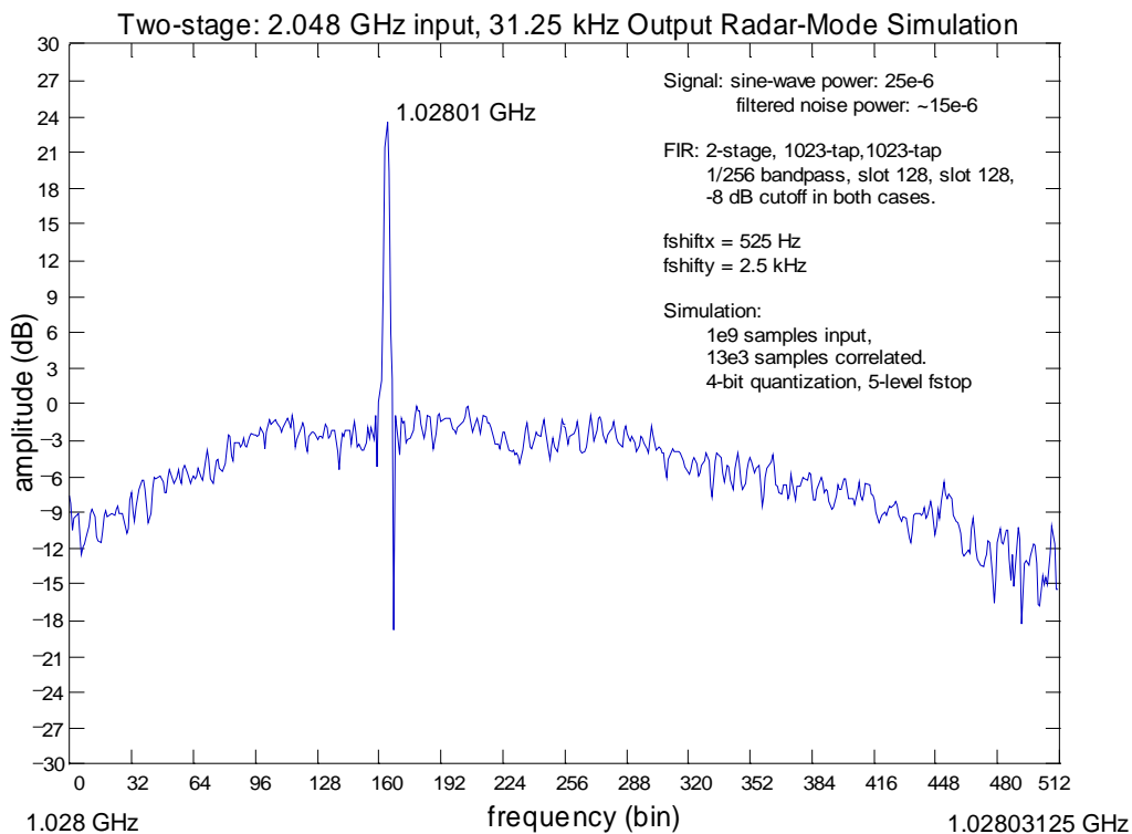
Figure 5 Simulation results with 2-stage filtering where each filter is 1/256 bandpass. The input bandwidth is 2.048 GHz and the output bandwidth is 31.25 kHz. Provided the narrowband signal is near the center of each filter's passband (or at least well enough away from the edge—see Figure 1), the total SNR degradation for a 4-bit system including fringe rotation loss is 6.5%.
