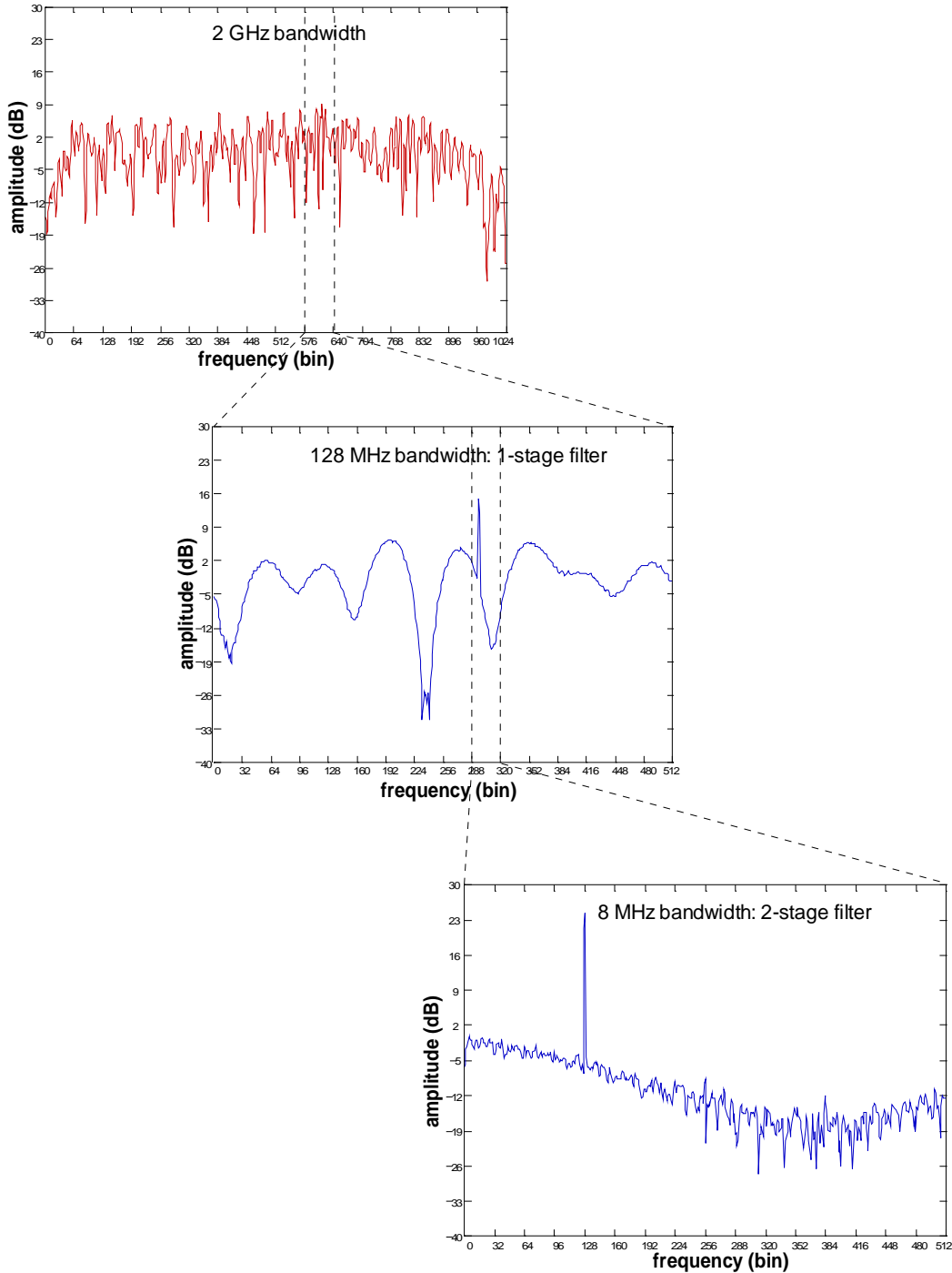
Figure 4 Simulation of 2-stage filtering with 1/16 bandpass filters used in each stage. The bandpass is much flatter than the single stage filter—evidenced by the lack of roll-off in the upper and lower parts of the bottom spectrum.
