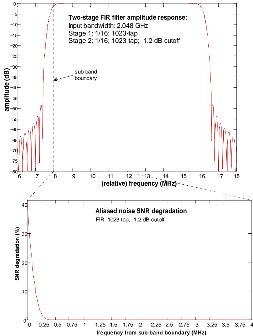
Figure 3 Two-stage filter performance with each stage performing a 1/16 bandpass using 1023-tap FIR filters. The top plot shows the amplitude response within the sub-band and just outside the sub-band boundaries. The filter has a -1.2 dB cutoff for very flat behaviour in the passband. The bottom plot shows the SNR degradation.
