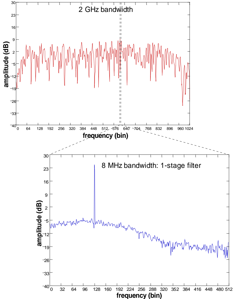
Figure 2 Simulation of 1/256 narrowband filtering and correlation of a spectrum with lots of structure and a narrowband line. The bandshape has not been corrected and the roll-off at the upper and lower edges of the band is evident (compare this to Figure 4).
