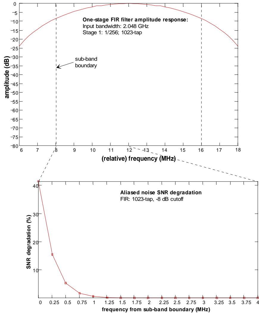
Figure 1 One-stage, 1/256 bandpass, 1023-tap FIR filter performance. The top plot shows the amplitude response across the sub-band and slightly outside the sub-band boundaries. The bottom plot shows the SNR degradation near the sub-band boundary resulting from transition band aliasing. Additionally, reject-band attenuation is about -40 dB.
