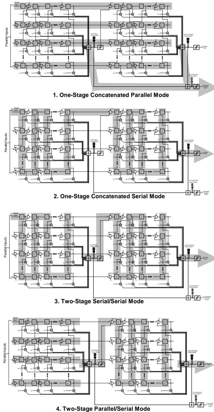
Figure 7 Proposed programmable FIR filter configurations. The correlator would normally use modes 1. and 4. Modes 2. and 3. are for more general purpose filtering applications.
