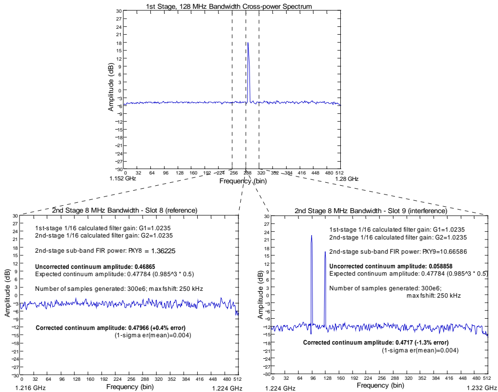
Figure 8 Plot showing the results of 2-stage correlation with and without narrowband signals. The top plot is a single stage correlation, the bottom left plot is the reference 2-stage correlation with no narrowband signals, and the bottom right is the 2-stage correlation with narrowband signals present. The continuum amplitude of the 2-stage correlation with narrowband signals is established to within -1.3 % of the expected level. The negative error is (presumably) due to higher quantization noise from the powerful narrowband signals although it is not entirely certain if this is the cause since the result is within \sim 1.5\sigma ( \sigma=0.004 ) of the expected value.
