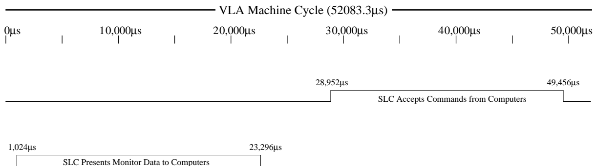
VLA Machine Cycle.
