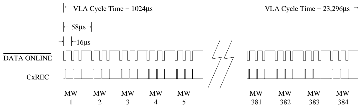
Figure 3.2.2-1. Monitor Cycle Timing.
